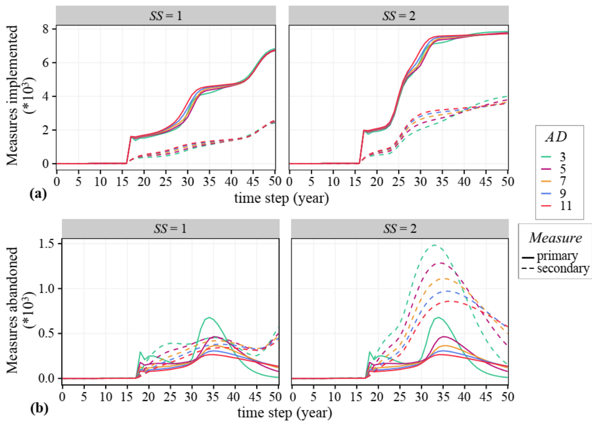
885 Figure 13. Impacts of the adaptation duration on the adaptation behaviour of agents. (a) shows the primary and secondary measures implemented, and (b) shows the primary and secondary measures abandoned. The left and right panels show simulation results without subsidies and with subsidies for flooded agents, respectively.
