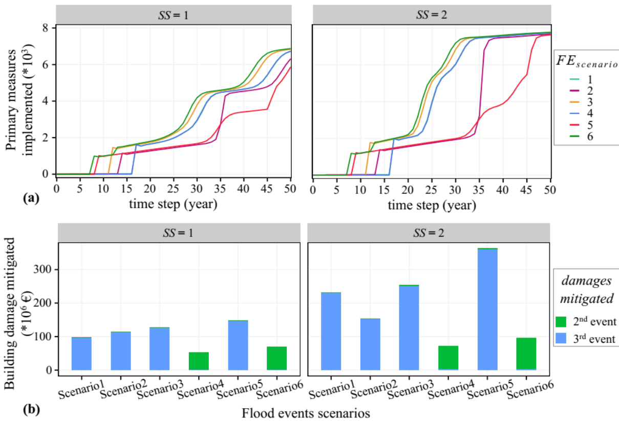
870 Figure 9. Effects of six flood event scenarios on the adaptation behaviour of agents and the associated impact. (a) shows the cumulative number of primary measures implemented, and (b) shows the potential building damage mitigated due to the primary measures implemented. In both (a) and (b), the left and right panels show the simulation results without subsidies and with subsidies for flooded agents, respectively.
