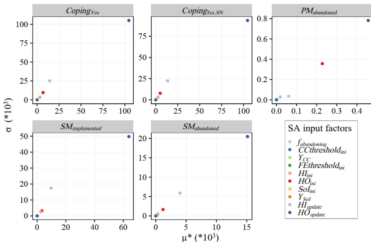
Figure D-1. Scatter plots displaying the Morris sensitivity measures \mu^* and \sigma for five of the response factors. Points representing the least important factors may not be visible as they overlap close to the (0, 0) coordinate.
