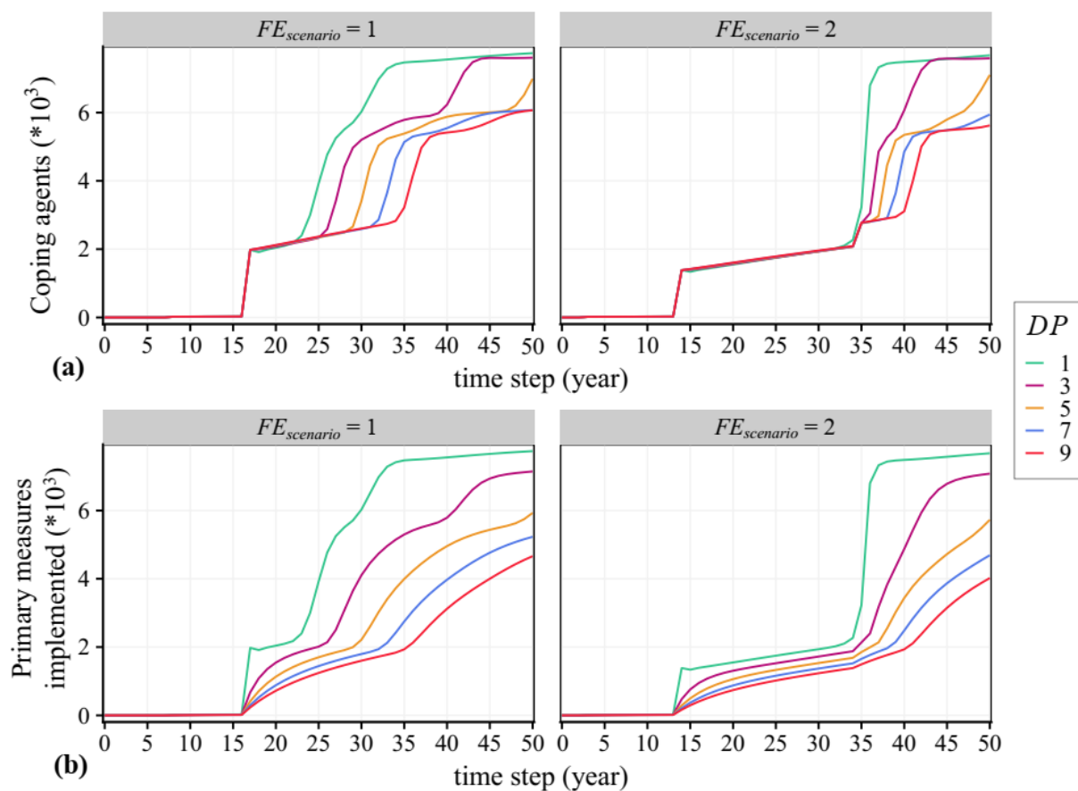
880 Figure 12. Impacts of the delay parameter on the adaptation behaviour of agents. (a) shows the coping behaviour of agents and (b) shows the cumulative number of agents that converted their coping behaviour to action, i.e., implement primary adaptation measures. Simulations that generated the results are set with SS = 2 . The left and right panels show simulation results with flood events scenarios of 1 and 2, respectively.
