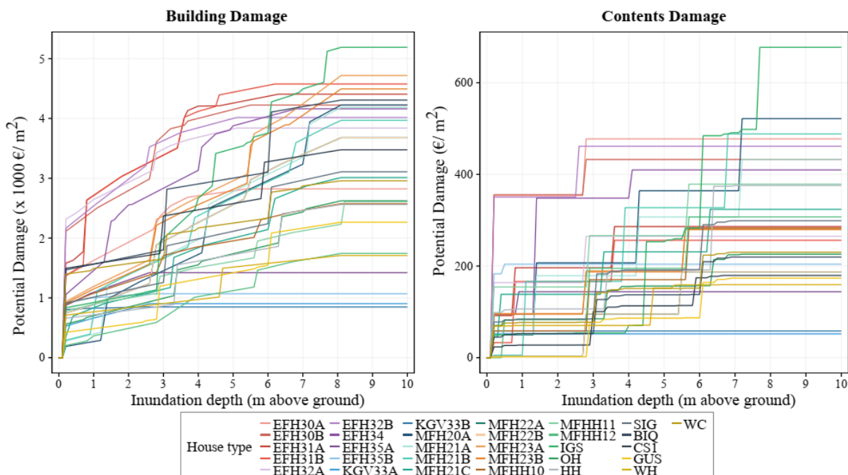
Figure 6. Depth-damage curves for building (left panel) and contents (right panel) of 31 house types in Wilhelmsburg. A description of the house type codes is given in Appendix B.
