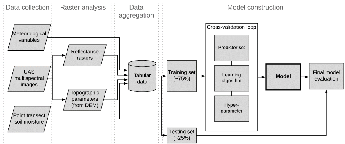
Figure 1 Process flowchart of model development.
