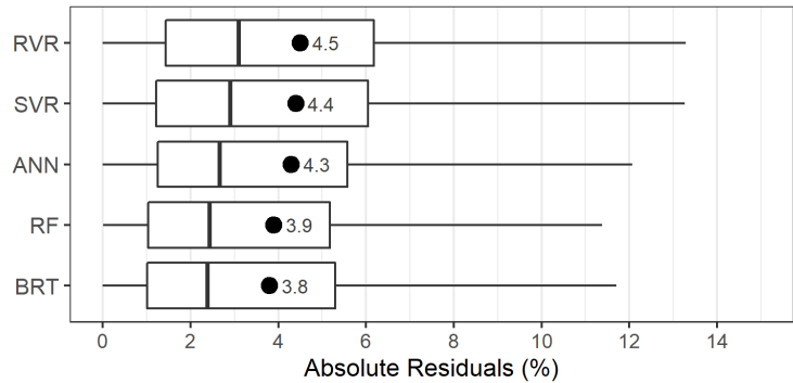
Figure 6 Distribution of residuals and MAE on the testing set by the type of machine learning algorithm. Filled circles and values to their right indicate the average MAE.
