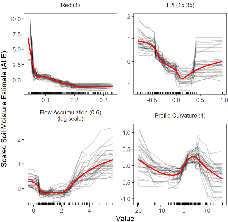
495 Figure 9 ALE plots for four selected high importance predictor variables. The black curves represent the individual effects of the 30 models, and red curves are smoothed trendlines overall individual models. Marks along the x-axis show the distribution of data in the model training set.
