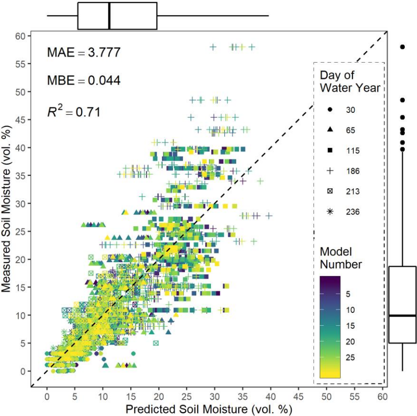
Figure 7 Scatter plot of the measured versus predicted soil moisture content for the testing sets. Marginal boxplots show the distributions of measured and predicted values. MAE, MBE, and R2 are averaged across the 30 models.
