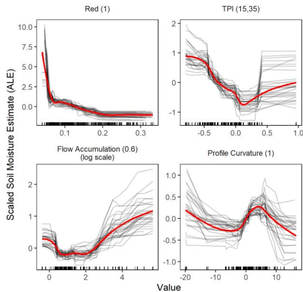
500 Figure 9 ALE plots for four selected high importance predictor variables. The black curves represent the individual effects of the 30 models, and red curves are smoothed trendlines overall individual models. Marks along the x-axis show the distribution of data in the model training set.
