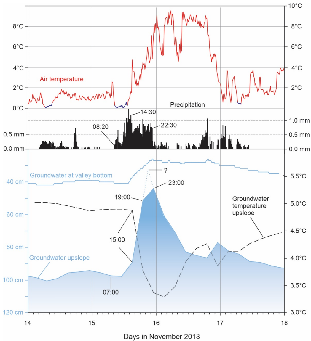
Figure 8: Air temperatures, precipitation and groundwater between 14 and 18 November 2013. The upper diagram shows air temperature (red curve) and precipitation in mm per 10 min. The lower diagram shows the groundwater level and groundwater temperature. Blue segments of the air temperature-curve show periods when the temperature is close to 0°C. Groundwater probably reached its highest level between 19:00 and 23:00, shown as a dotted line and a question mark.
