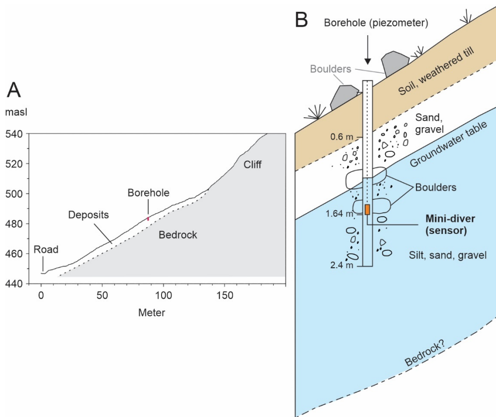
Figure 5: Profile of the hillside just south of the southern slide scar of the 2007 landslide (Fig. 4B) showing the borehole with the instrumented piezometer. A. Average steepness of the sediment-covered slope is 25–26°. The stippled line indicates where we believe the boundary between till and bedrock is located, based on observations from the 2007 slide scar (Fig. 4B). B. The mini-diver (sensor) is suspended from a wire in the piezometer and anchored 1.64 m below the surface. The top 60 cm of deposits consists of organic soil and weathered till, with firm till below that. We drilled through boulders at depths of ca. 1 m and 1.5 m.
