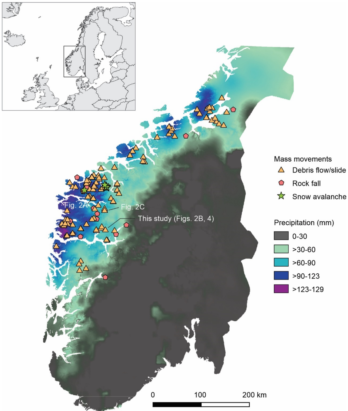
Figure 1: Mass movements that occurred on 15 and 16 November 2013 during storm Hilde in Western Norway – 114 debris flows and slides, 28 rockfalls and 7 snow avalanches and. Data retrieved from the Norwegian landslide database: https://gis3.nve.no/link/?link=SkredHendelser . Precipitation is interpolated from observations and shows the amount in mm per 24 hours, collected at 06:00 UTC 16 November (08:00 local time), data retrieved from http://www.xgeo.no/ .
