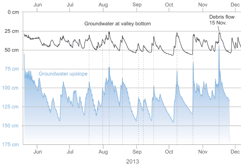
215 Figure 7: Groundwater fluctuations in June–December 2013. The upper curve (black) shows fluctuations at the weather station in the valley bottom. The blue curve shows the fluctuations in the borehole upslope. The minima and maxima occur at the same time (dotted lines), but the peaks upslope are sharper, last less than 4 hours, have higher amplitudes, and the individual peaks reach different levels. The ground in the valley bottom is saturated at a registered depth of around 25 cm.
