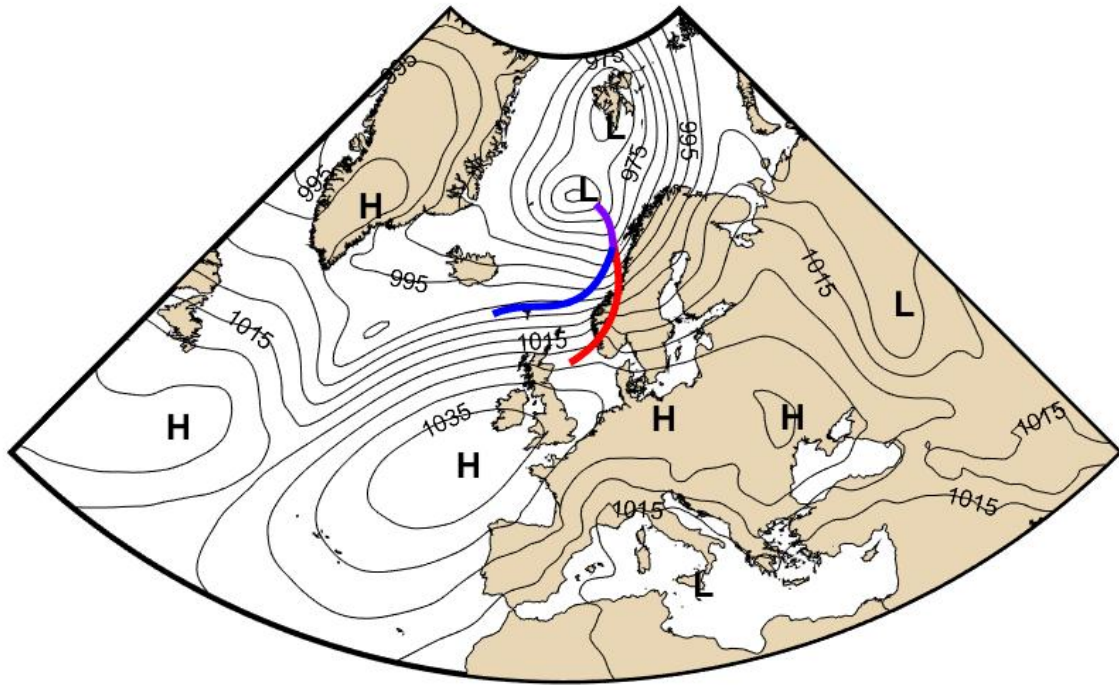
75 Figure 3: Mean sea level pressure (hPa) on 15 November at 12:00 UTC (14:00 local time). Large amounts of warm and moist air blew towards the Norwegian coast because of low pressure northeast of Iceland and high pressure southwest of England. The air was close to 100 % saturated with water vapor, which precipitated as the air cooled when it rose over the mountains in western Norway. The red line indicates the position of the warm front and the blue line is the cold front. The warm air sector lies between the red and blue lines. The purple line indicates an occluded front, which 80 means that the cold front has caught up with the warm front.
