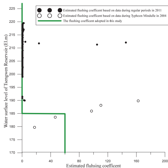
Fig. A.1 Relationship between the flushing coefficient and WSL of Tsengwen Reservoir
