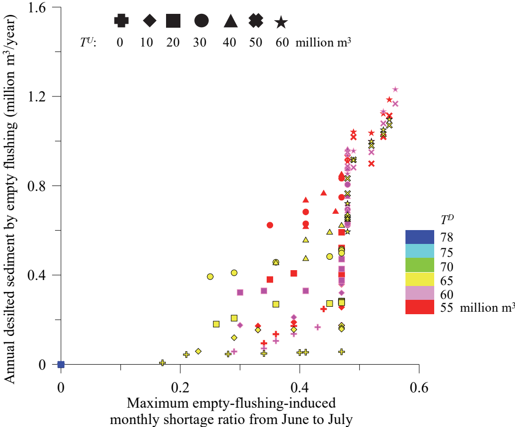
5 Fig. 8 Simulation results of various empty flushing strategies using the original storage balancing curves
