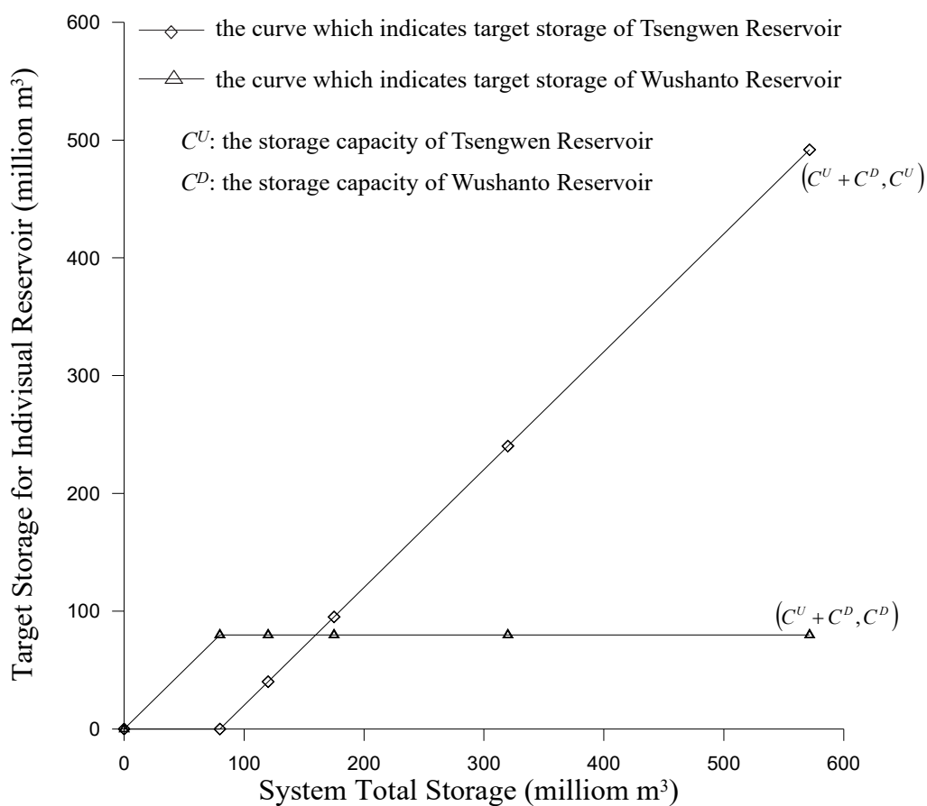
Fig. 7 Modified storage balancing curves using Tsengwen Reservoir as primary source to satisfy water demand
