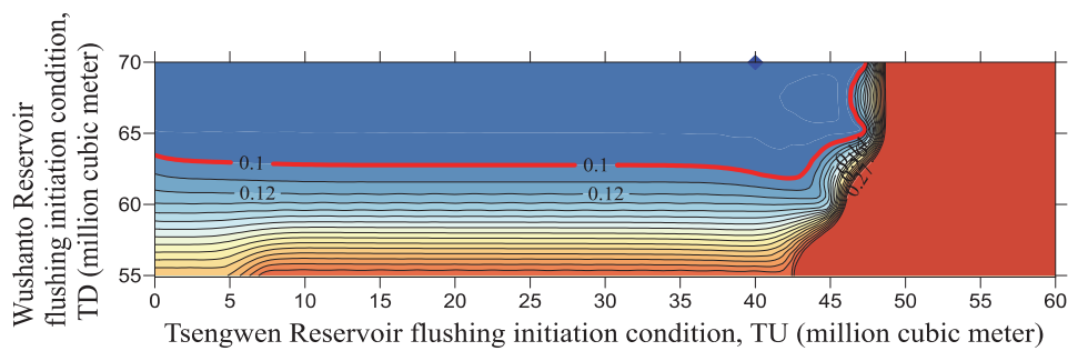
(d) Contour of the maximum monthly shortage ratio from June to July for different T^U and T^D with \psi = 60, 180 or 300
