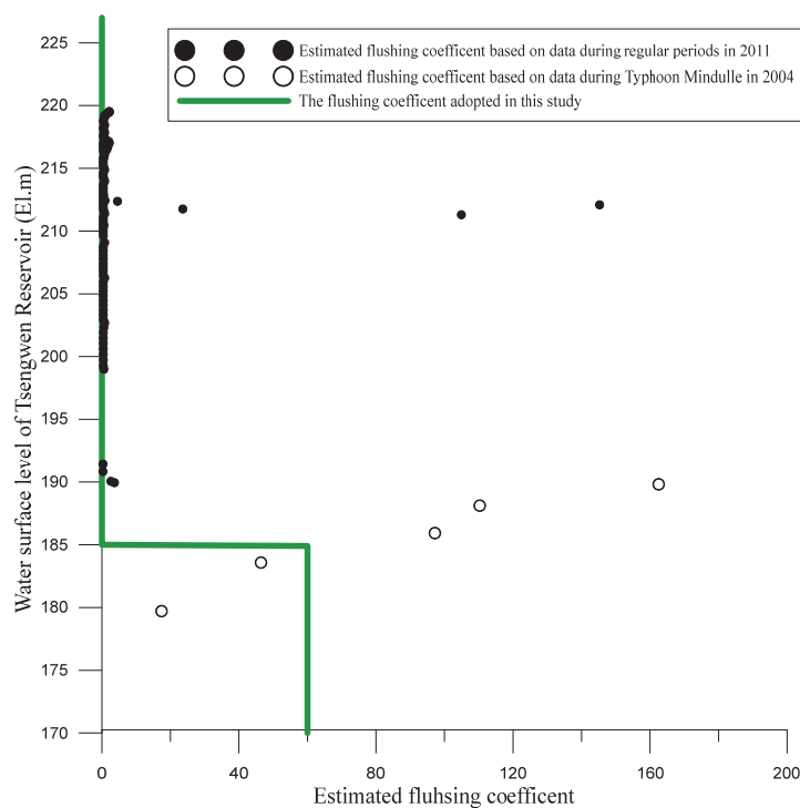
15 Fig. 13 Relationship between the flushing coefficient and WSL of Tsengwen Reservoir
