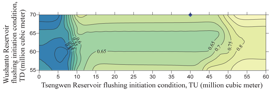
(b) Contour of the desilting volume for different T^U and T^D with \psi = 180
