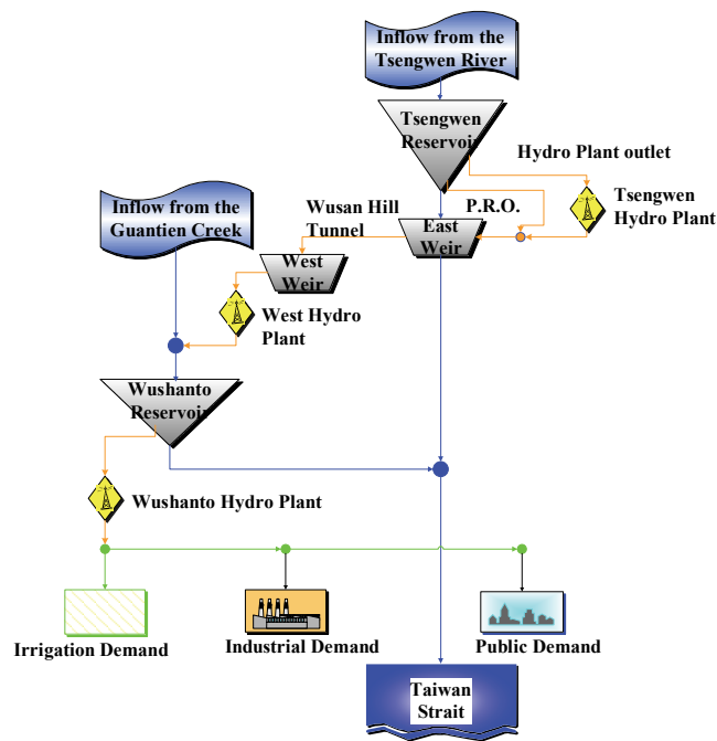
Fig. 2 Network of the joint operating system of Tsengwen and Wushanto Reservoirs
