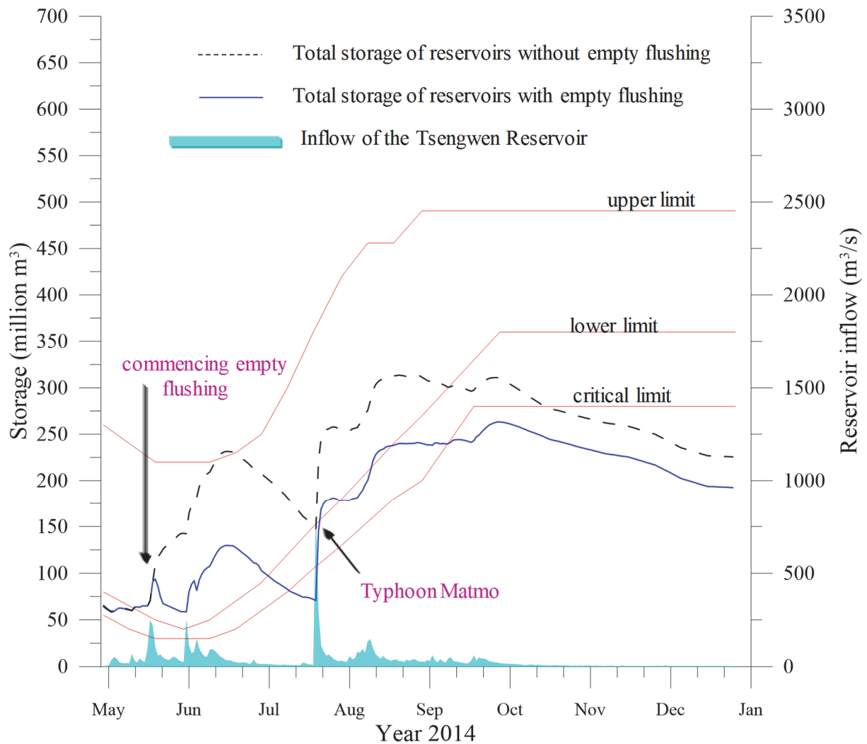
Fig. 12 Reservoir inflow and storage throughout 2014
