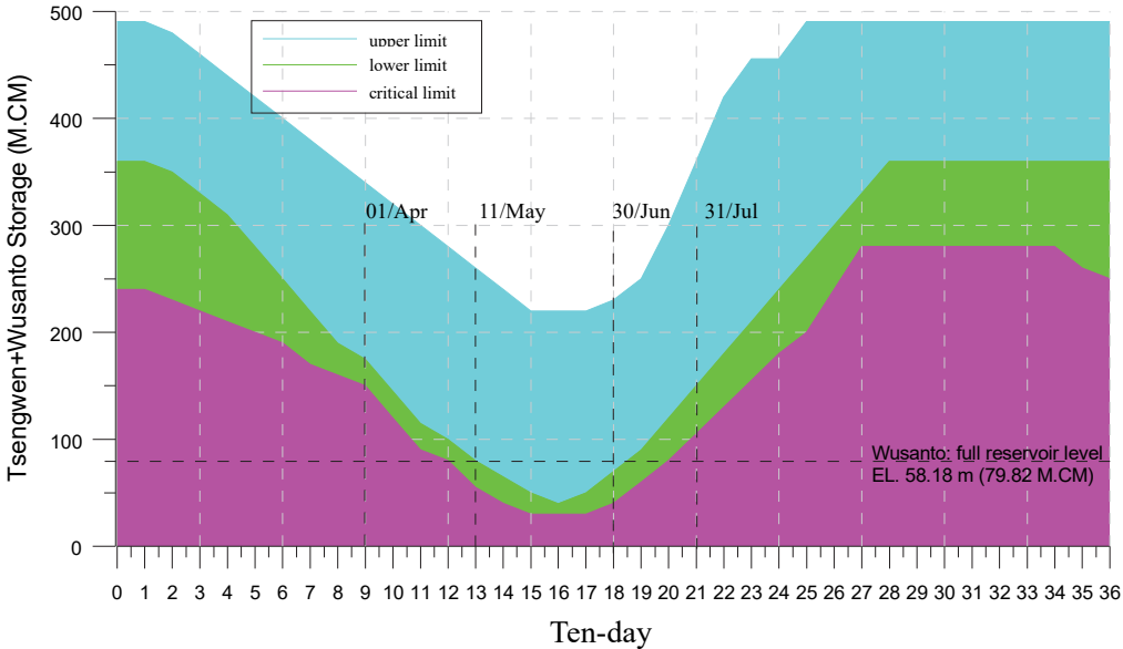
Fig. 3 Joint operating rule curves of the Tsengwen and Wushanto Reservoirs
