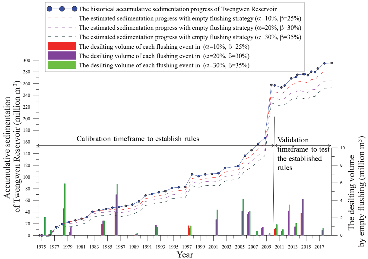
Fig. 10 The sedimentation progress of Tsengwen Reservoir with and without empty flushing
