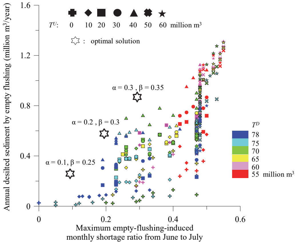
Fig. 9 Simulation results of various empty flushing strategies using modified storage balancing curves from April to June
