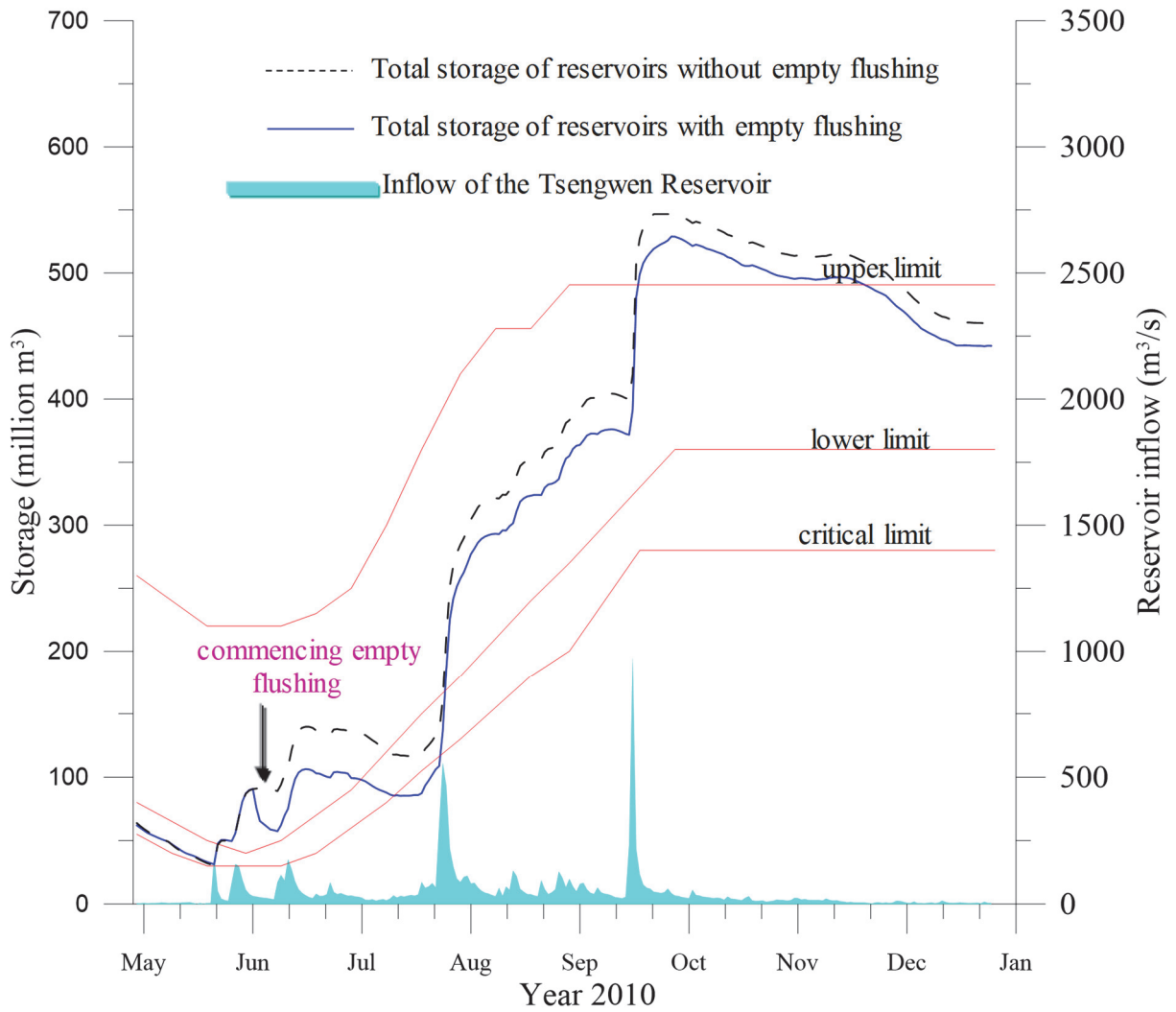
Fig. 11 Reservoir inflow and storage throughout 2010
