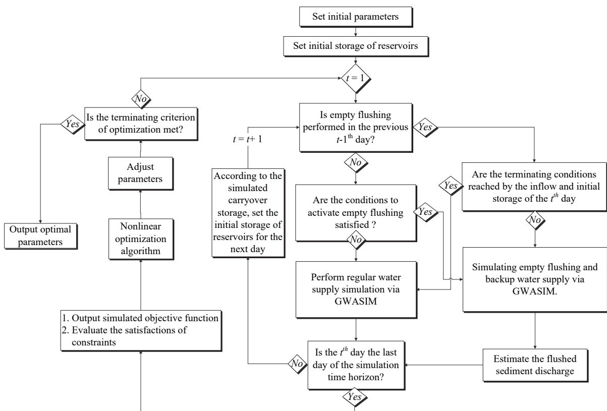
Fig. 6 The procedure to derive the optimal empty flushing strategy
