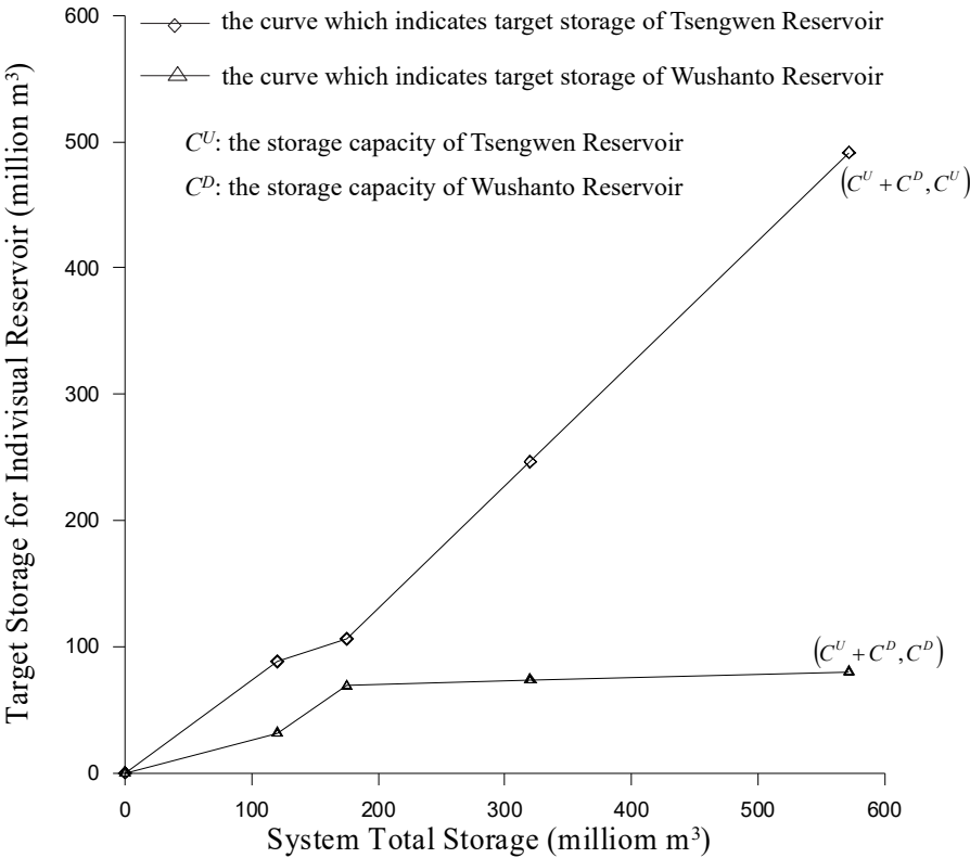
Fig. 4 Storage balancing curves for Tsengwen and Wushanto Reservoirs in the tenth ten-day period (early April)
