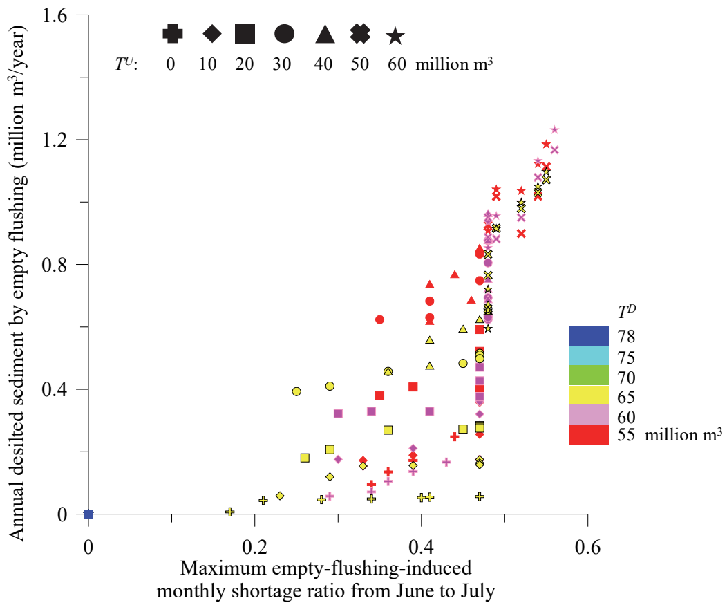
Fig. 8 Simulation results of various empty flushing strategies using the original storage balancing curves
