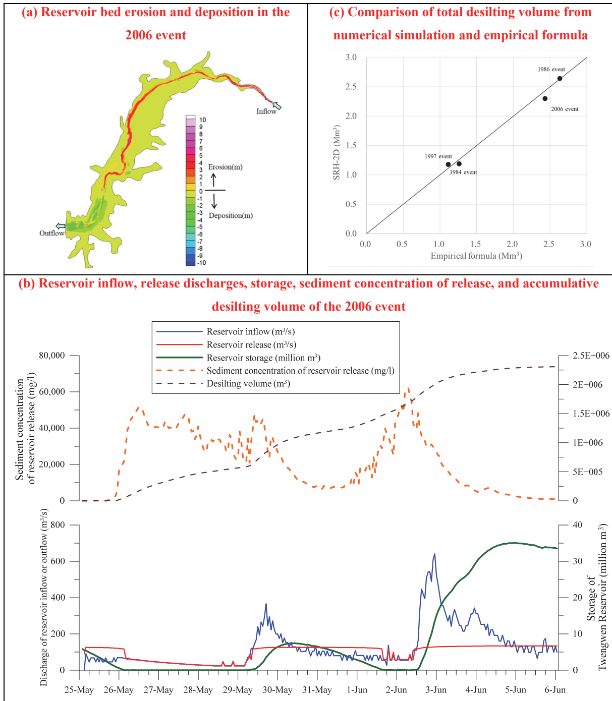
Fig. 14 Simulation results of the SRH-2D
