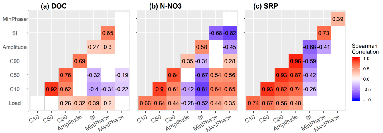
260 Figure 3. Matrices of Spearman's rank correlations of water quality (load, concentration percentiles (10 th (C10), 50 th (C50), and 90 th (C90)), and seasonality metrics) for (a) dissolved organic carbon (DOC), (b) nitrate N (N-NO 3 ), and (c) soluble reactive phosphorus (SRP) (c). Only significant (p ≤ 0.05) values are shown.
