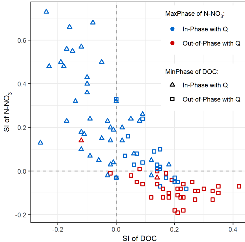
330 Figure 5. Relationship between the seasonality indices (SI) of nitrate N (N-NO 3 - ) vs. dissolved organic carbon (DOC) in the headwater catchments for which seasonality was significant for both parameters (n=98). The color and shape of symbols identify the seasonality types based on the NO 3 MaxPhase and DOC MinPhase metrics. The threshold date was 1 May: MaxPhase that occurred before were classified as “in-phase” with discharge (Q), while those that occurred after were “out-of-phase” with Q. The DOC MinPhase metric is shown to highlight the synchrony between minimum DOC and maximum N-NO 3 concentrations.
