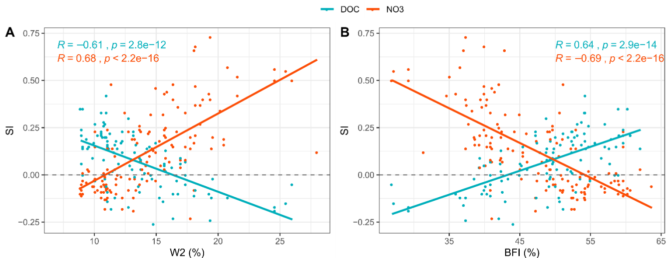
Figure 6. Relationship between the seasonality index (SI) of dissolved organic carbon (DOC) and nitrate ( \text{NO}_3 ) and the hydrological reactivity descriptors (A) flow flashiness index (W2) and (B) base-flow index (BFI) for 124 headwater catchments.
