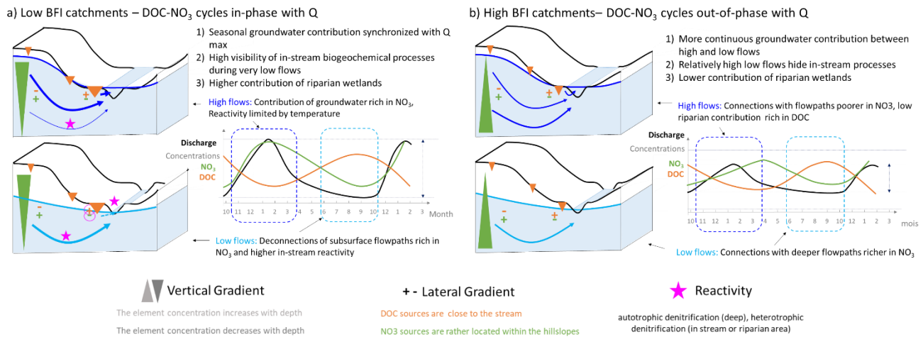
430 Figure 7. Conceptual diagram of seasonal flowpaths involved in the DOC-NO 3 seasonal cycles leading to a) in-phase cycles with discharge or b) out-of-phase cycles with discharge.
