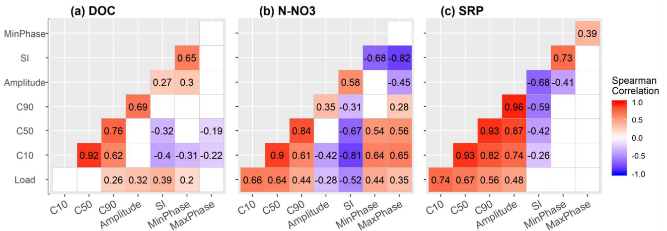
Figure 4. Matrices of Spearman's rank correlations of water quality (load, concentration percentiles (10 th (C10), 50 th (C50), and 90 th (C90)), and seasonality metrics) for (a) dissolved organic carbon (DOC), (b) nitrate N (N-NO 3 ), and (c) soluble reactive phosphorus (SRP). Only significant ( p \leq 0.05 ) values are shown.
