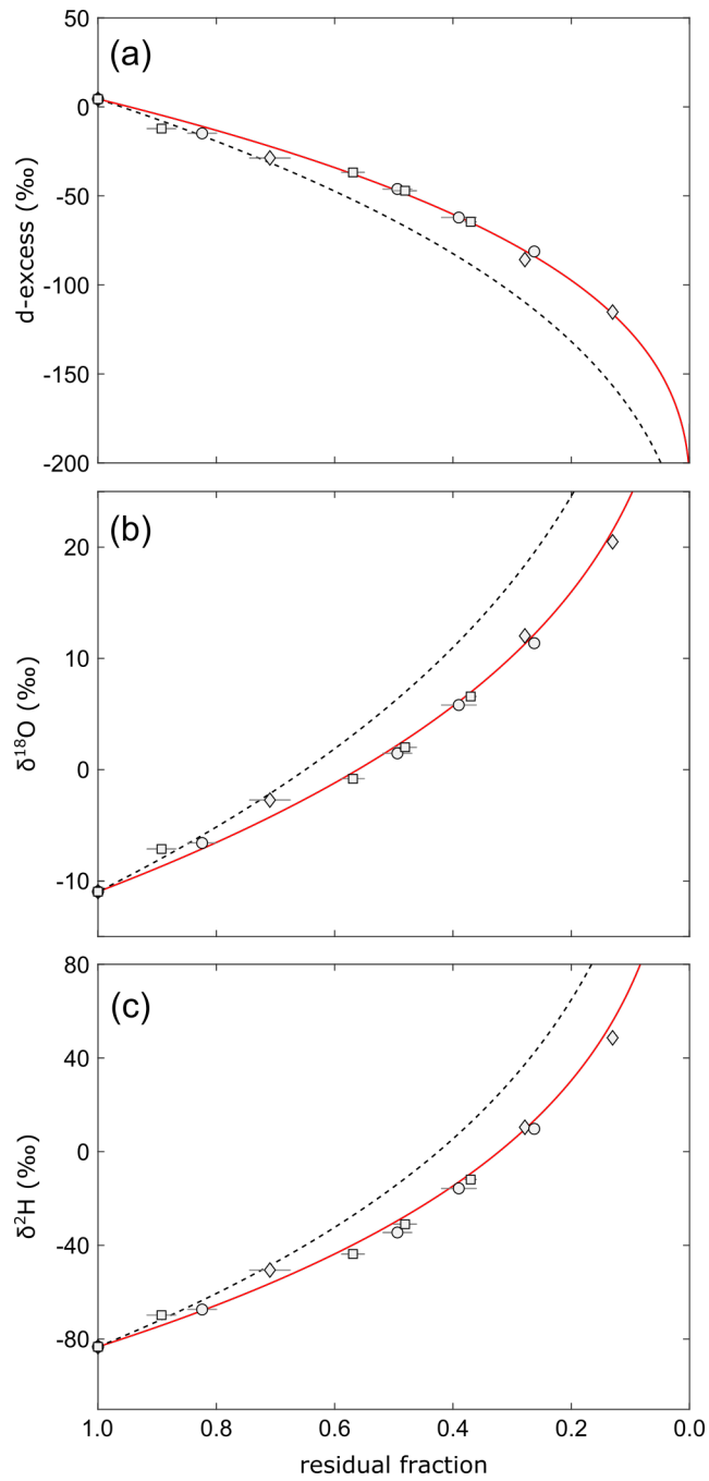
Figure 9: Isotopic evolution of remaining water in evaporation experiments, similar to figure 8. Here, the red lines show evaporation trajectories obtained by fitting the virtual outlet model ( n = 0.59 , outlet = 20%). The dashed lines represent evaporation trajectories for the simple evaporation model obtained using the same turbulence coefficient as for the virtual outlet model.
