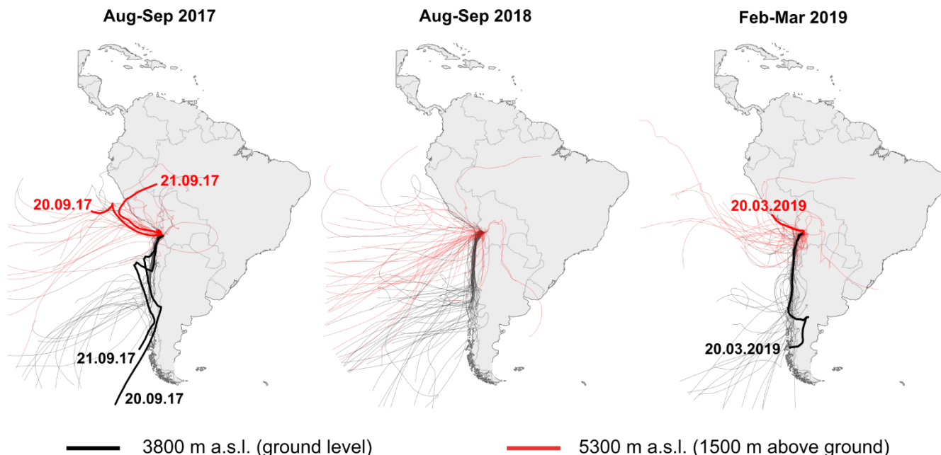
Figure 5: HYSPLIT 7-day air mass back trajectories modelled for ground level at the Salar del Huasco (~3800 m above sea level (a.s.l.)) (black) and 1500 m above ground level (5300 m a.s.l.) (red) in daily resolution for the period from 23.08.2017 to 22.09.2017. The thick red and black trajectories represent modelled back trajectories for the time of vapour sampling on 20.09.17, 21.09.2017 and on 20.03.20
