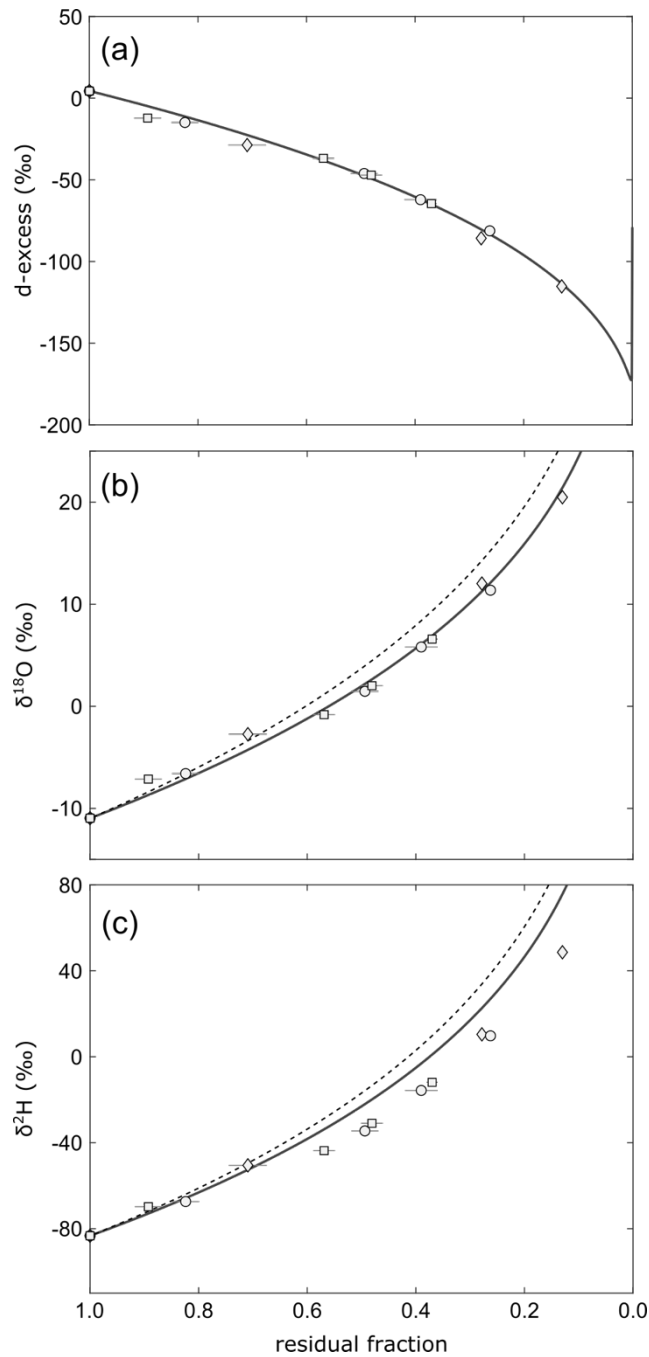
Figure 8: Evolution of (a) d-excess, (b) \delta^{18}\text{O} , and (c) \delta^2\text{H} of remaining water in the evaporation experiments. The solid lines show evaporation trajectories obtained by fitting the simple evaporation model independently to \delta^{18}\text{O} ( n=0.34 ), \delta^2\text{H} ( n=0 ) and d-excess ( n=0.44 ) vs residual fraction. Note that the \delta^2\text{H} data cannot be fitted for any reasonable turbulence coefficient. The dashed lines in (a) and (b) are evaporation trajectories modelled using the same turbulence coefficient as for the d-excess data.
