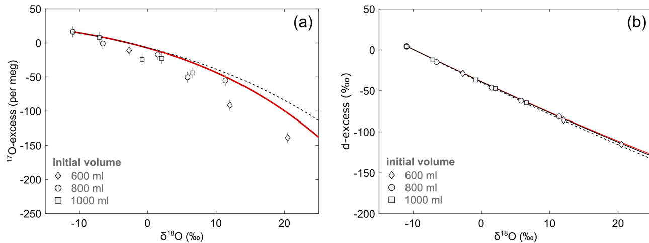
Figure 6: Isotopic data of pan evaporation experiments in the diagrams of (a) ^{17}\text{O} -excess over \delta^{18}\text{O} and (b) d-excess over \delta^{18}\text{O} . Pan evaporation experiments were carried out with different initial volume of 600 ml (diamonds), 800 ml (circles), 1000 ml (squares). Note that the symbol size can be larger than the error bars. The solid black line in panel (b) shows the best fitting evaporation trajectory ( n = 0.55 ) for the simple evaporation model. The red lines represent the evaporation trajectories modelled using the virtual outlet model with n = 0.59 and an outlet of 20% (see text). Dashed lines illustrate the evaporation trajectories modelled with the simple evaporation model using the same turbulence coefficient as for the virtual outlet model. Model input parameters are summarized in Table 2.
