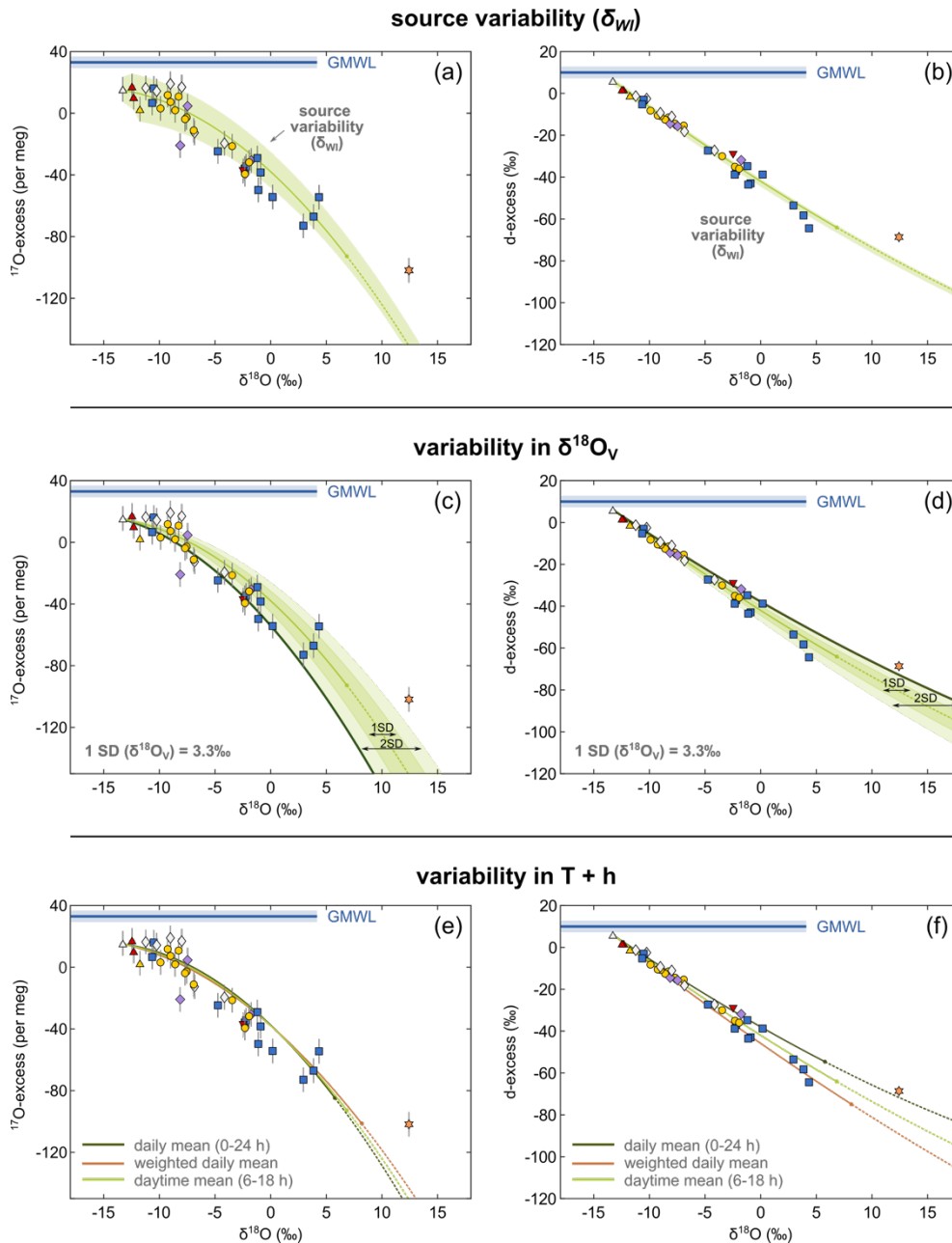
665 Figure 11: Illustration of the impact of variability and uncertainty in the model input parameters on the evaporation trajectory exemplified for lakes and ponds sampled in 09/17. The green line shows the modelled recharge evaporation trajectory for mean daytime conditions (6-18 h) at the Salar del Huasco. The shaded green areas in panel (a) and (b) illustrate the uncertainty introduced to the modelled trajectory by spatial variability in the isotopic composition of inflowing water ( \delta^{18}O_{WI} ). The dark solid lines represent corresponding evaporation trajectories in panel (a) and (b). Panel (c) and (d) show the impact of variable \delta^{18}O_v on the evaporation trajectory illustrated by multiples intervals of the SD (1SD = 2.6 ‰; shaded areas). Panel (e) and (f) illustrate the effect of uncertainty in the assumed effective evaporation time interval. Recharge evaporation trajectories have been modelled for (1) daily mean (0-24 h; h = 33 %, T = 4°C) (dark green curve), (2) daily mean h = 20 % and T = 10°C weighted for the average diurnal distribution of temperature and wind speed (brown curve), and (3) daytime mean (6-18 h; h = 27 %, T = 7°C) conditions (light green curve). 670
