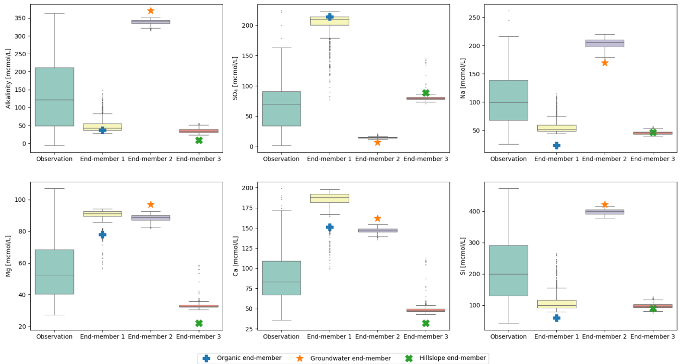
Figure 5. Uncertainties of CHEMMA predicted end-members compared with the total solute variances. Each CHEMMA end-member (end-member 1 to 3) is matched with a field measured end-member. The six subplots represents six observed solute space.
