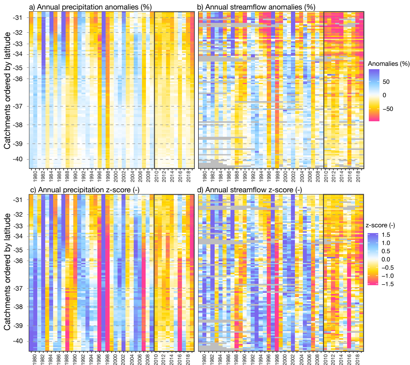
355 Figure 5: Relative annual anomalies of catchment-scale precipitation (panel a) and streamflow (panel b). Panels c and d present the z-score of annual precipitation and streamflow. The MD period (April 2010 to March 2020) is highlighted in a grey box. Each row in the heatmaps corresponds to one study catchment and the catchments are sorted from north to south to illustrate regional drought patterns.
