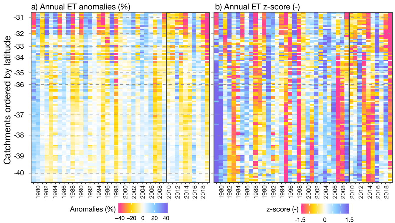
Figure S2: Panel b presents the z-score of simulated annual ET (computed as deviations from mean normalised by standard deviation). The MD period (April 2010 to March 2020) is highlighted in a grey box. Each row in the heatmaps corresponds to one study catchment and the catchments are sorted from north to south to illustrate regional patterns.
