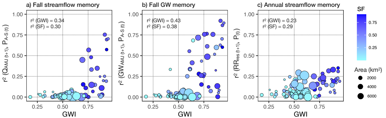
340 Figure 4: Relationship between hydrological memory and indices of groundwater and snow storages (GWI and SF, respectively). Panel a shows the fall streamflow (9-months) memory to the fall-winter precipitation of the preceding year. Panel b shows the fall GW (9-months) memory to the fall-winter precipitation of the preceding year. Panel c shows the (>12-months) memory of streamflow the precipitation of the preceding year.
