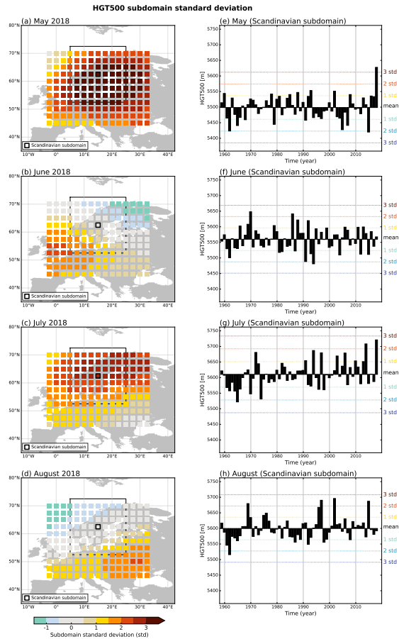
Fig. 1. Same as Figure A3 in the paper, except that the same range is used for HGT500 values in the right panel.
