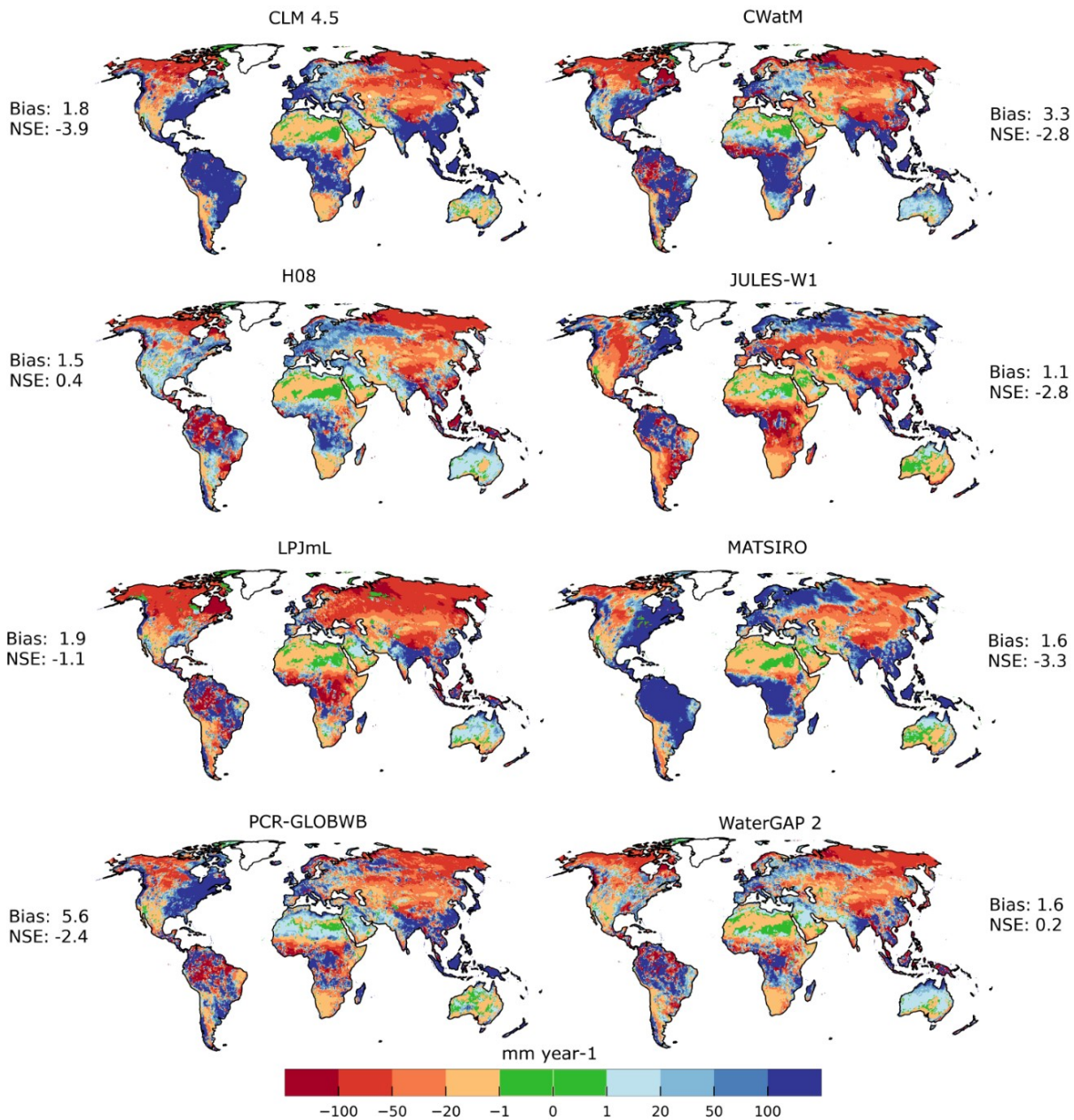
Figure 9 PI GWR per GHM – 34 years (1981-2014) mean GWR [mm year -1 ] of Mohan et al. (2018). Bias: mean (GHM Mohan et al. -1 ). NSE (Nash-Sutcliff Efficiency; (Nash and Sutcliffe, 1970)) is calculated spatially over all cells instead of time.
