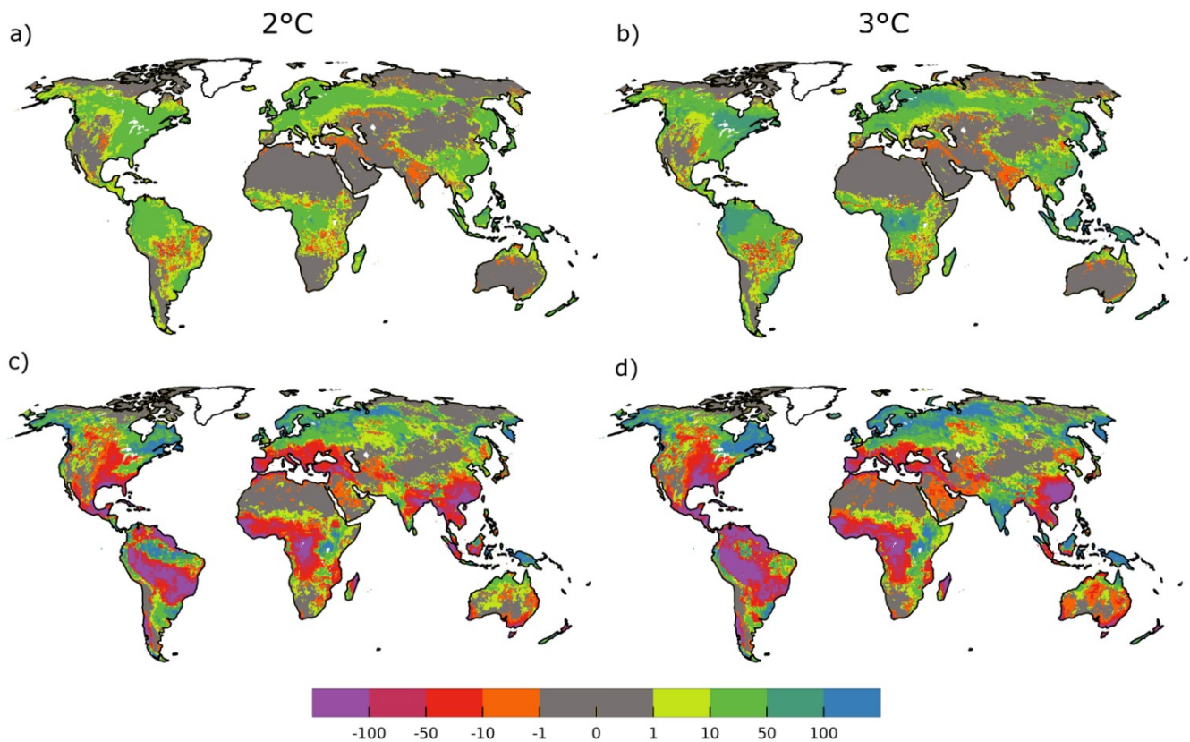
420 Figure 6 GWR (dynamic CO 2 ) – GWR (static CO 2 ) [mm year -1 ] for 2.0°C (a) and 3.0°C (b) GW. GWR (dynamic CO 2 ) – PI (dynamic CO 2 ) [mm year -1 ] for 2.0°C (c) and 3.0°C (d) GW. The figure only includes the GHM CLM 4.5 and the GCM GFDL-ESM2M. Maps show changes in GWR at a certain GW (including all RCPs that lead to that GW with a certain CO 2 concentration) with dynamically evolving CO 2 compared to static CO 2 concentrations from 2005. Green and blue means that GWR is higher when evolving CO 2 concentrations are considered, red and purple less GWR.
