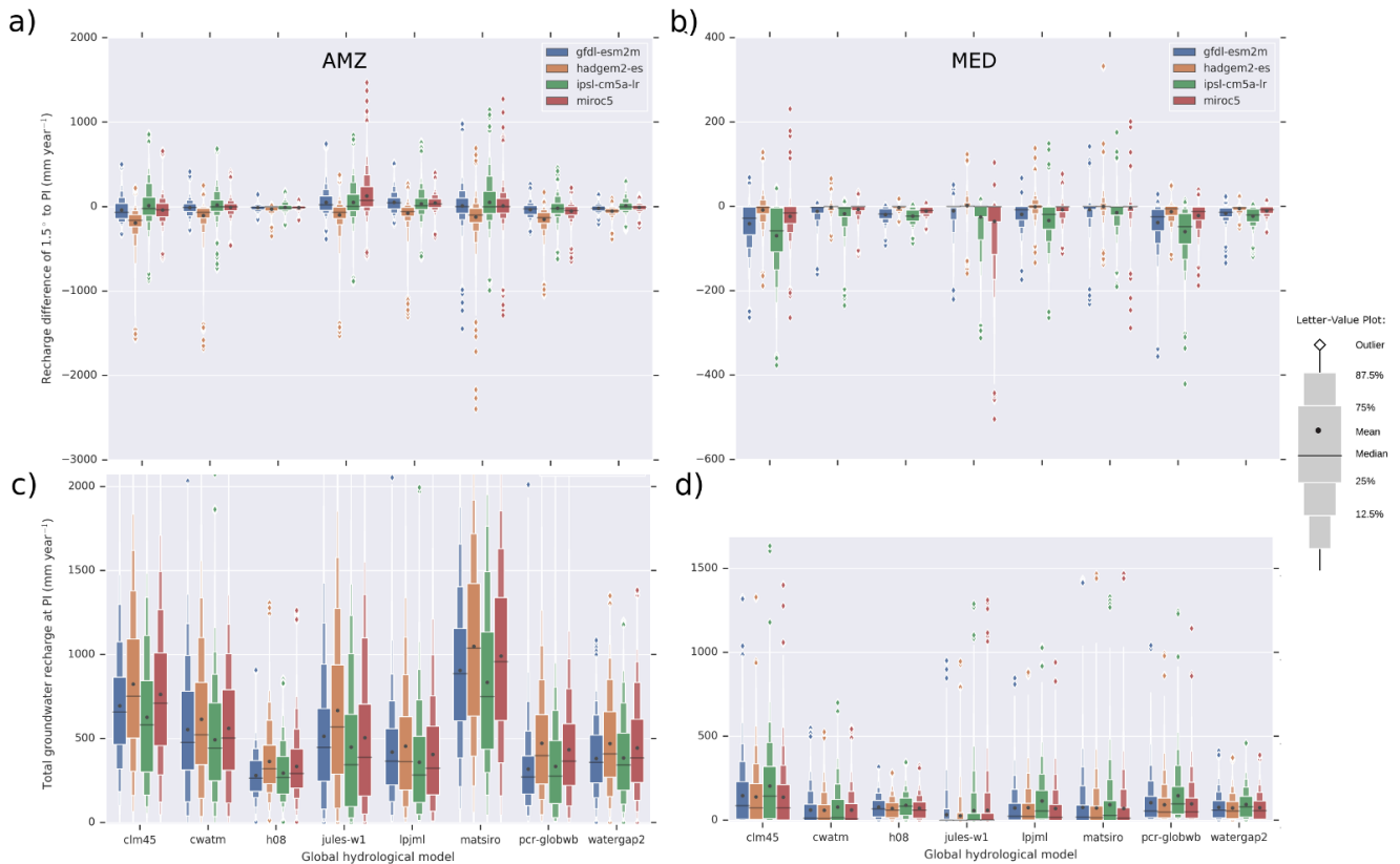
Figure 4 Letter-value plot (Hofmann et al., 2017) of absolute changes in GWR in 0.5^\circ grid cells [ \text{mm year}^{-1} ] at 1.5^\circ\text{C} GW compared to PI (a, b) and absolute PI GWR [ \text{mm year}^{-1} ] (c, d) for the Amazon (a, c) and South Europe/Mediterranean (b, d) SREX region (for all other regions and GW levels [ 2^\circ\text{C} , 3^\circ\text{C} ] see supplement). No statistical test is applied and all grid cells inside a region are included. Each box may include multiple simulations with different RCPs.
