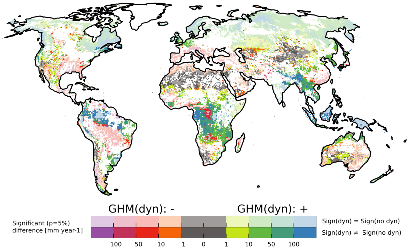
470 Figure 8 Significant absolute difference of GWR change between 1981-2010 and 2077-2099 for RCP 8.5 in between four GHMs with (dyn) and four GHMs without dynamic (or active) vegetation (no dyn). See also Table 1. Reddish (left side of the color bar) indicates that the mean change of GWR as computed by the models with dynamic vegetation is more negative or less positive than change computed by other models. White regions indicate no significance is based on the K-S test (Sect. 2.5). Solid colors indicate that the majority of the two model groups (3 out of 4 models for each group) do not have the same sign i.e. that including dynamic vegetation leads to different signs in GWR change. Lighter colors indicate where the majority agrees on the sign of change.
