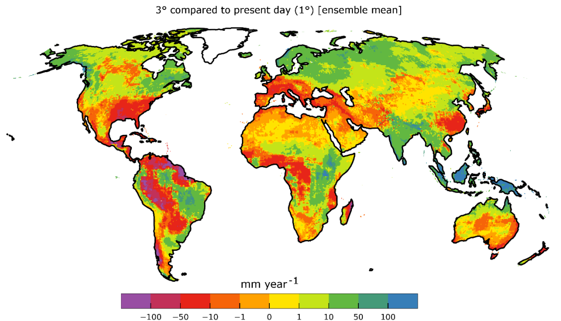
Figure 2 Ensemble mean change in GWR [ \text{mm year}^{-1} ] between conditions of present day warming of 1^\circ \text{C GW} and at 3^\circ \text{C GW} , averaged over the GWR changes of all GHM-GCM model combinations.
