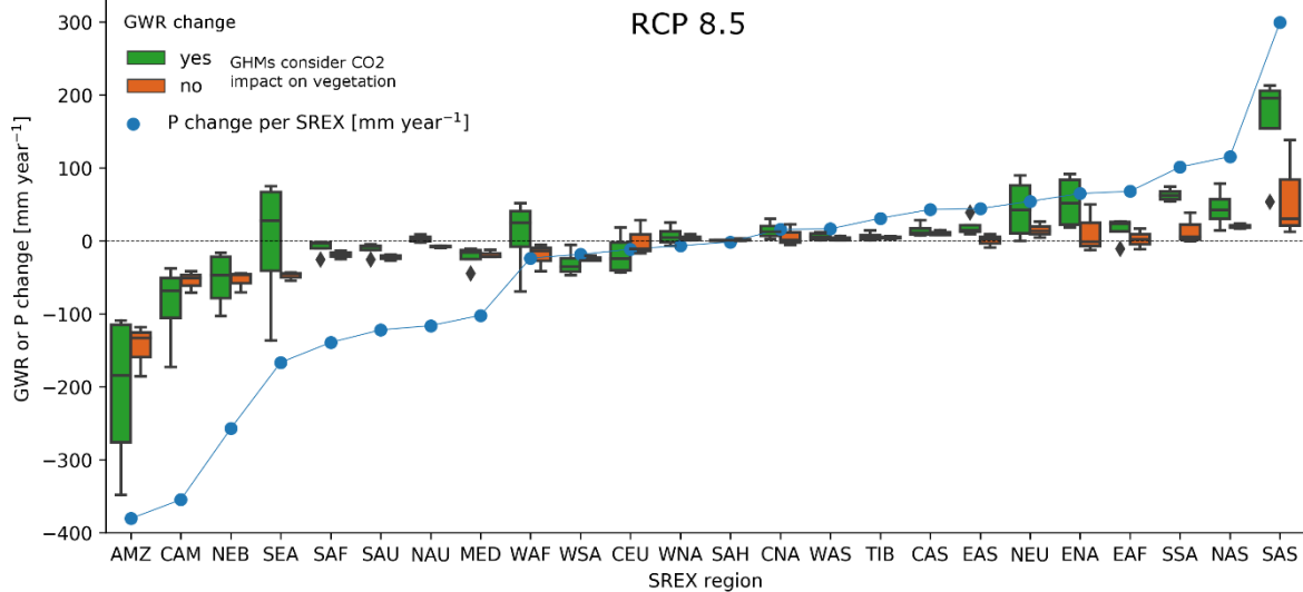
435 Figure 7 Relation of changes in precipitation (P) (mean(1981-2010) – mean(2070-2099)) to changes in GWR (mean(1981-2010) – mean(2070-2099)) depending on the model type (with or without CO 2 ; see also Table 1) per SREX (selection as in Table 3) for RCP 2.6 and RCP 8.5 for the GCM HadGEM2-ES.
