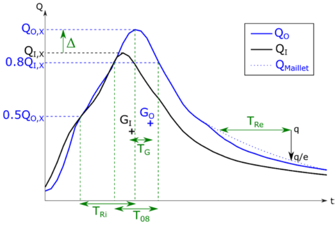
885 Figure 2: Storm hydrograph with characteristic times and discharge values. Q_{o,X} and Q_{i,X} are peakflows of outlet and inlet station hydrographs Q_o and Q_i , respectively. T_G is the elapsed time between the corresponding gravity centres G_o and G_i .
