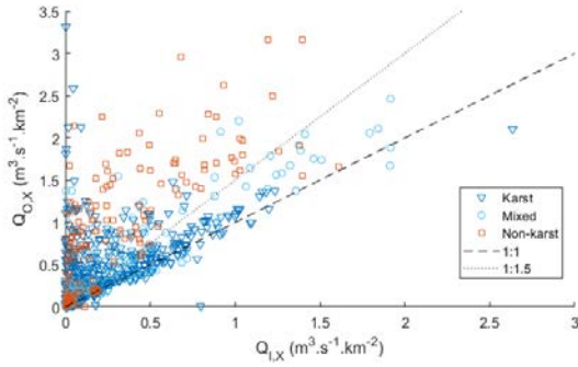
910 Figure 7: Variation of peakflow ( Q_x , see Appendix D) from inlet to outlet stations, with representation of geology type.
