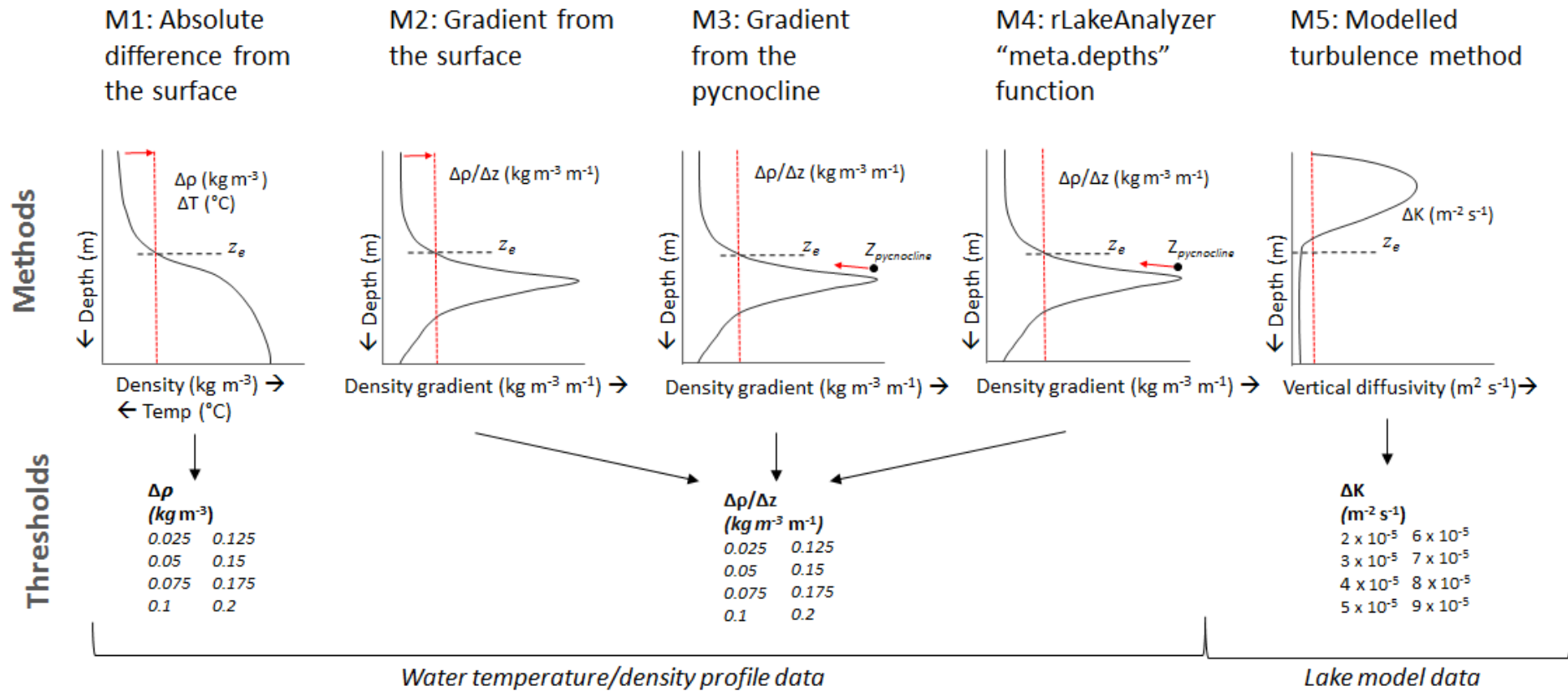
945 Figure 2. Schematic of epilimnion depth methods used in this study, including the range of threshold values for each method and the input data type (i.e. water temperature/density profile data or lake modelled data).
