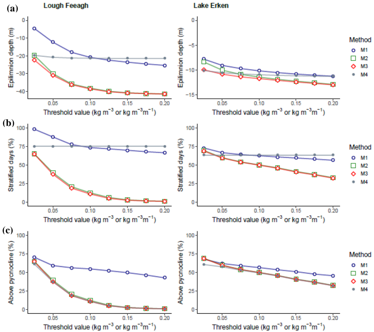
1025 Figure 6. Mean Apr-Oct epilimnion depth (m) (a), percentage of stratified days, defined as days where the epilimnion depth was identified as shallower than the lake maximum measured depth ( % ) (where a larger percentage value indicated a higher occurrence of days identified as stratified) (b), and percentage of days 1030 where the epilimnion depth was above the pycnocline, defined as the number of days where the epilimnion was identified at a depth shallower than the maximum density gradient (where a larger percentage value indicated a lower occurrence of days erroneously extending into the metalimnion) (c), for Lough Feeagh and Lake Erken.
