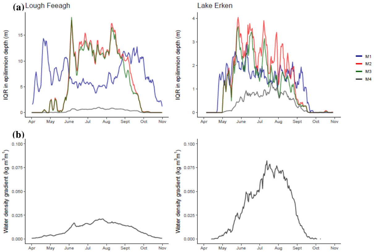
1050 Figure 7. Inter-quartile range between the shallowest and deepest estimate for each method calculated from 1055 long-term daily mean epilimnion depth estimates for each Julian day, where a large range suggests high threshold sensitivity and a small range suggests low sensitivity (a), and long-term daily mean water density gradient, calculated based on the surface and maximum measured depths (b), for Lough Feeagh and Lake Erken.
