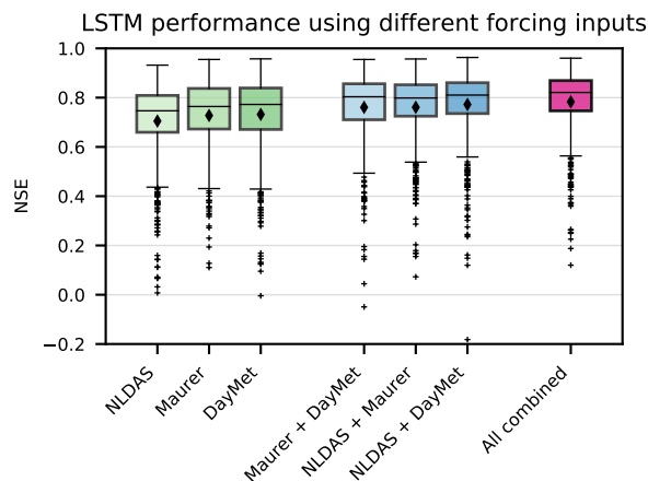
Figure 3. Test-period comparison between single-forcing and multiple-forcing LSTM ensembles ( n = 10 ) over 531 CAMELS basins. All differences are/were statistically significant ( \alpha = 0.001 ), with the exceptions of "DayMet" vs. "Maurer" ( p \approx 0.08 ) and "NLDAS + Maurer" vs. "Maurer + DayMet" ( p \approx 0.4 )
