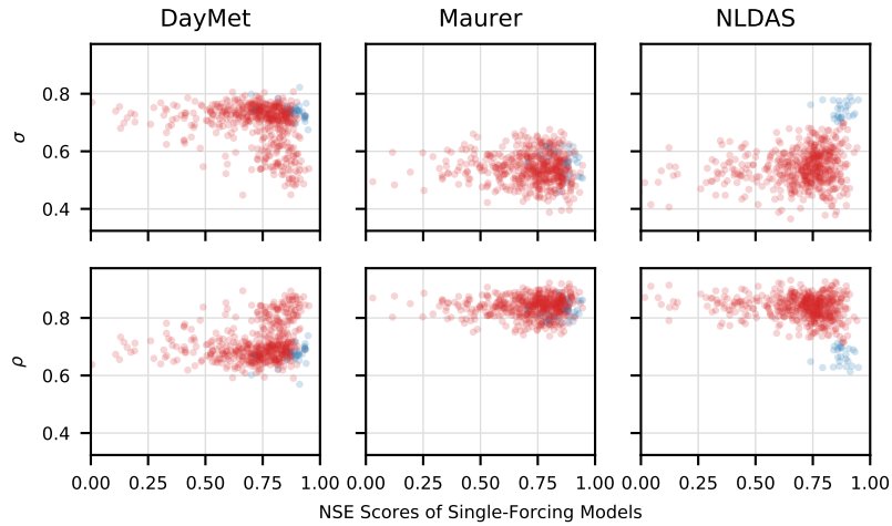
Figure C2. As in Fig. C1 the triple collocation error variances ( \sigma – Eq. C4) and truth-correlations ( \rho – Eq. C5) are plotted against NSE scores of the single-forcing LSTM models. The coloring shows the anomalous NLDAS basins in blue and all others in red. For these basins NLDAS has low correlation with the other two products but still yields high-skill simulations.
