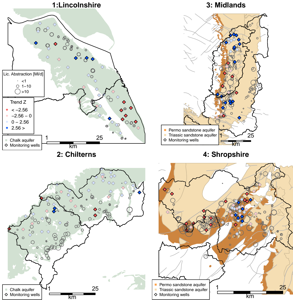
Figure 3. Trend values for monitoring wells in the four water management units (1: Lincolnshire, 2: Chilterns, 3: Midlands, 4: Shropshire). The red and blue diamonds indicate the positive or negative Z values for the Modified Mann-Kendall trend test for each monitoring well. Z values over |2.56| indicate a significant trend in the 30-year (1984-2014) groundwater level time series.
