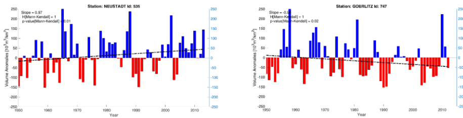
195 Fig. 4. Anomalies in annual streamflow volumes for the station of Neustadt (a) and Goerlitz (b). In the graphs, the slope of the Theil-Sens's line, H and p-value of the Mann Kendall test are also reported.
