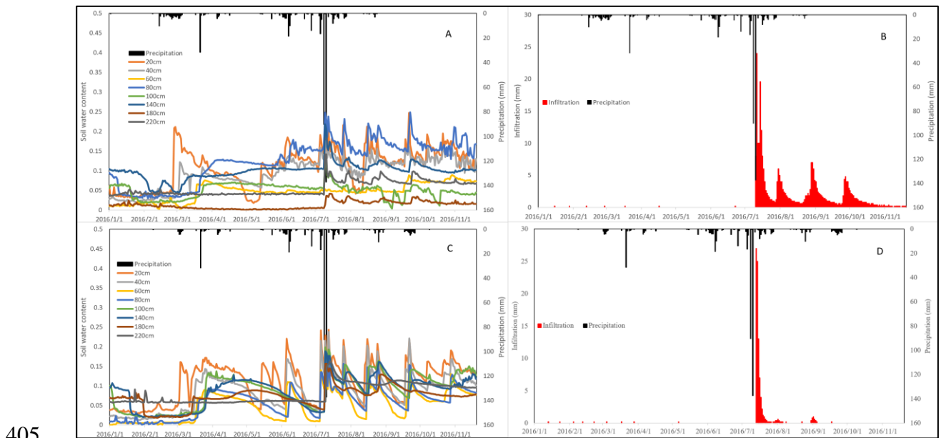
Figure 5. Effects of precipitation on soil moisture (A) and DSR (B) in bare sandy land plot; Effects of precipitation on soil moisture (C) and DSR (D) on ASK plot, 2016.
