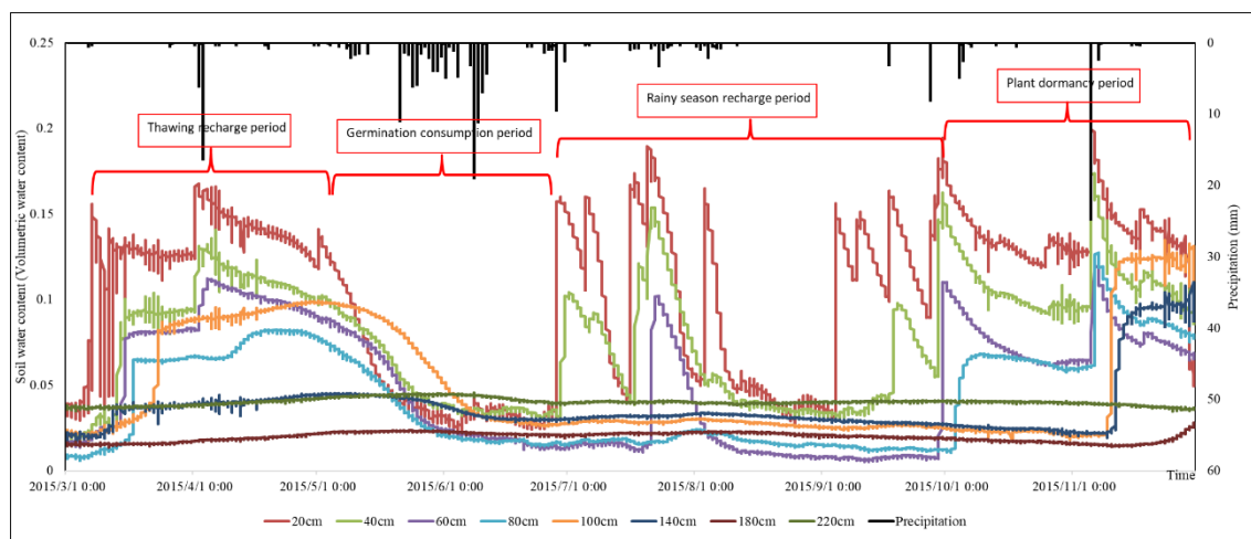
335 Figure 4 Daily soil water content distribution of ASK plot in 2015.
