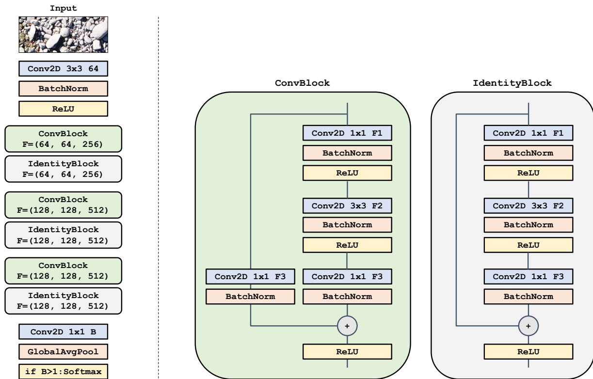
Figure B1. Illustration of the convolutional neural network architecture. Left: Full architecture where F = (F1, F2, F3) denotes the number of filters of the three convolutional layers within the residual blocks. The number of outputs B corresponds to the estimated histogram bins. To estimate a scalar (e.g. mean diameter) this B can be set to one. Right: The respective residual blocks. The ConvBlock has a learnable skip connection and is used when the number of output features is not equal to the number of input features. If constant, the IdentityBlock forwards the input.
