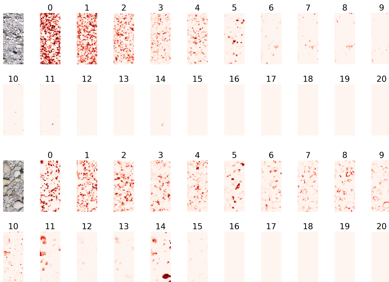
Figure 10. Activation maps after the last convolutional layer for two examples. Each of 21 maps corresponds to a specific histogram bin of the grain size distribution, where bin 0 corresponds to the smallest, bin 20 to the largest grains. Light colours are low activation, darker red denotes higher activation.
