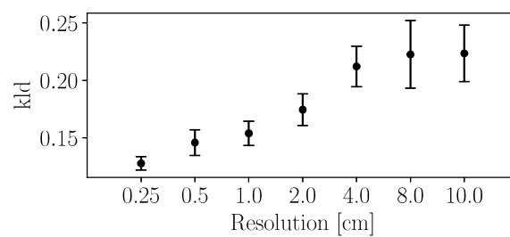
Figure E1. Resolution study for GRAINet regressing the relative frequency distribution by optimizing the KLD loss.
