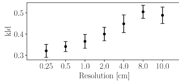
Figure E2. Resolution study for GRAINet regressing the relative volume distribution by optimizing the KLD loss.
