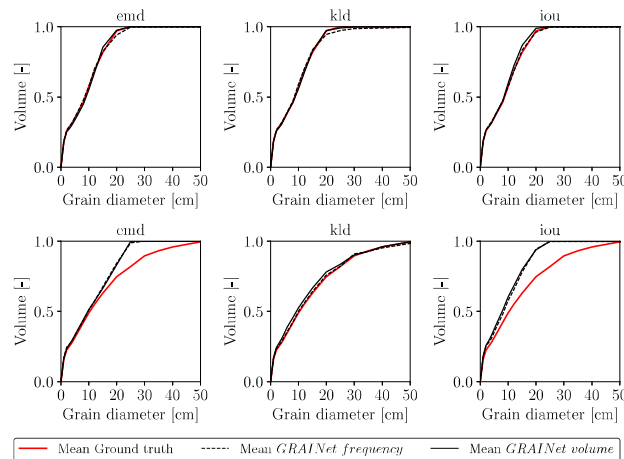
Figure 10. Grading curves resulting from optimizing different loss functions (from left to right: EMD, KLD, IoU) for two example gravel bars, namely Gr. Entle km 002.0 (top) and Reuss km 001.6 (bottom).
