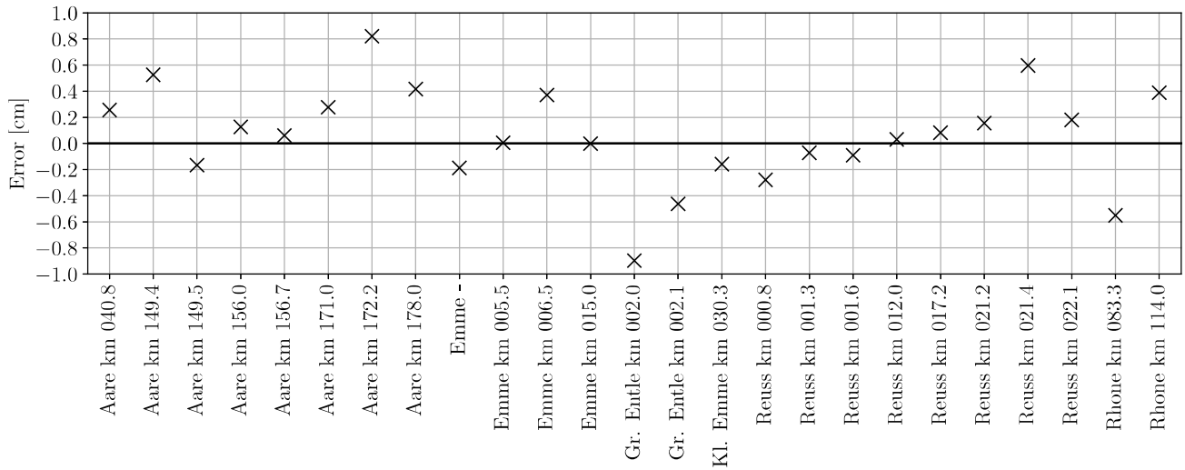
Figure 14. Error of the mean d_m per gravel bar derived from the GRAINet end-to-end d_m predictions.
