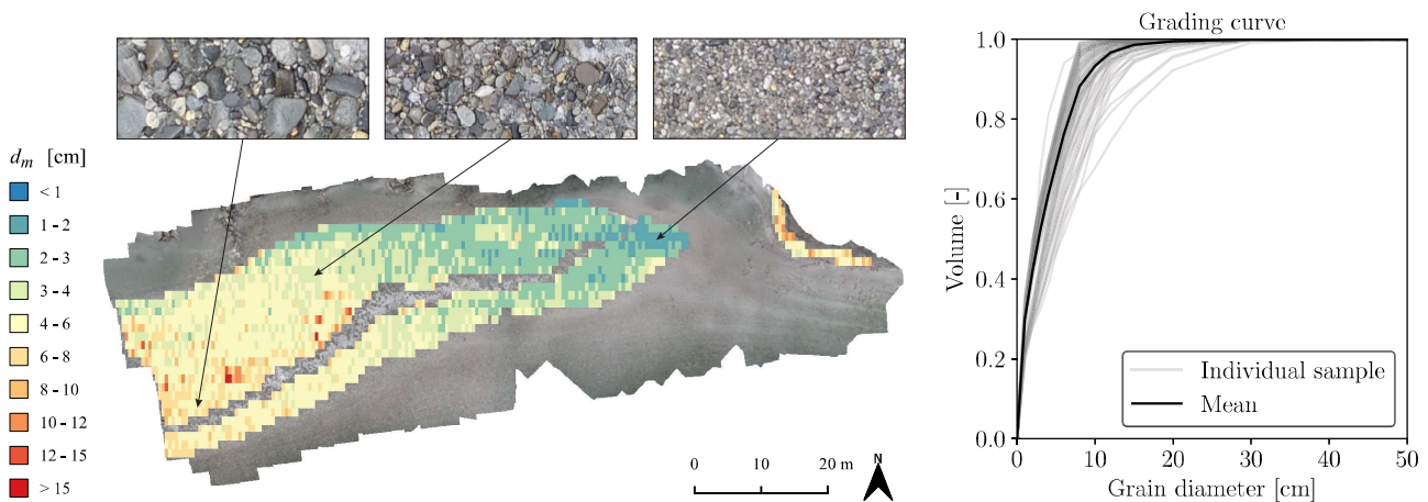
Figure 5. Illustration of the two final products generated with GRAINet on the river Rhone. Left: Map of the spatial distribution of characteristic grain sizes (here d_m ). Right: Grading curve for the entire gravel bar population, by averaging the predicted curves of individual line samples.
