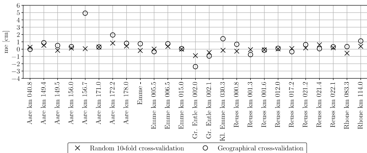
Figure D1. Mean error (bias) of the GRAINet end-to-end d_m regression per gravel bar (random – and geographical cross-validation).. A positive error implies that the GRAINet prediction was higher than the ground truth.
