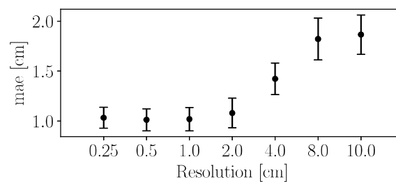
Figure 20. Performance of GRAINet d_m regression with different image resolutions (trained with MSE loss).
