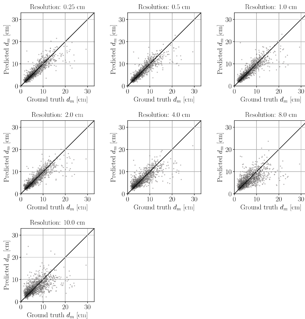
Figure E3. Scatter plots of GRAINet d_m regression with different image resolutions (trained with MSE loss).
