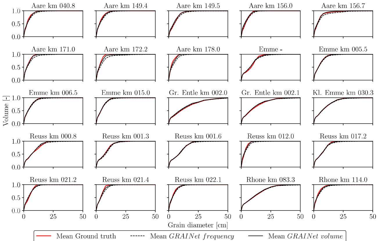
Figure 11. Grading curves of the 25 gravel bars, estimated with random 10-fold cross-validation.
