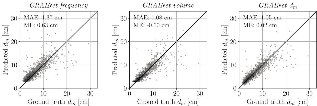
Figure 12. Scatter plots of the estimated d_m in cm from the three GRAINet outputs: frequency , volume , and d_m (left to right). The ground truth d_m on the horizontal axis and predicted d_m on the vertical axis.
