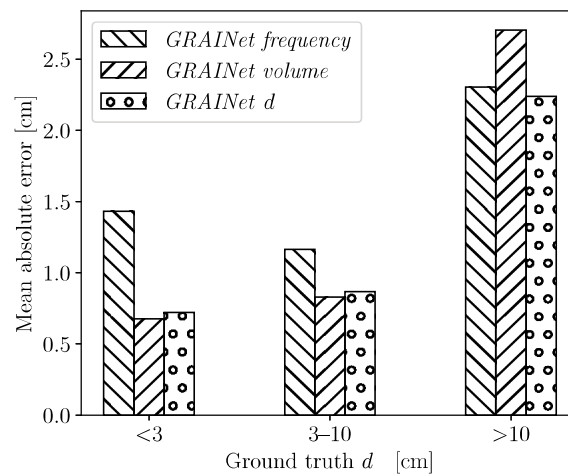
Figure 13. Mean absolute error of the predicted d_m for three d_m -categories: <3 cm, 3–10 cm, and >10 cm
