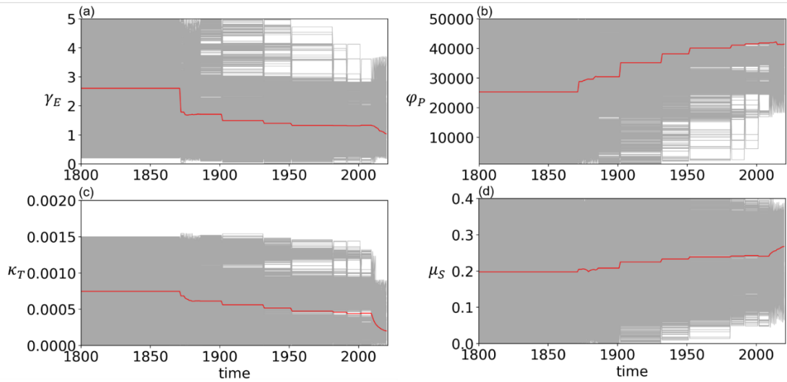
Figure S8. Timeseries of (a) the cost of levee raising \gamma_E , (b) the rate by which new properties can be built \varphi_P , (c) the rate of decay of levees \kappa_T , (d) memory loss rate \mu_S estimated by the data assimilation of observations of G and H with 5000 ensembles in the real-world experiment in the city of Rome. The timestep is annual. Grey and red lines are the ensemble members and their mean, respectively.
