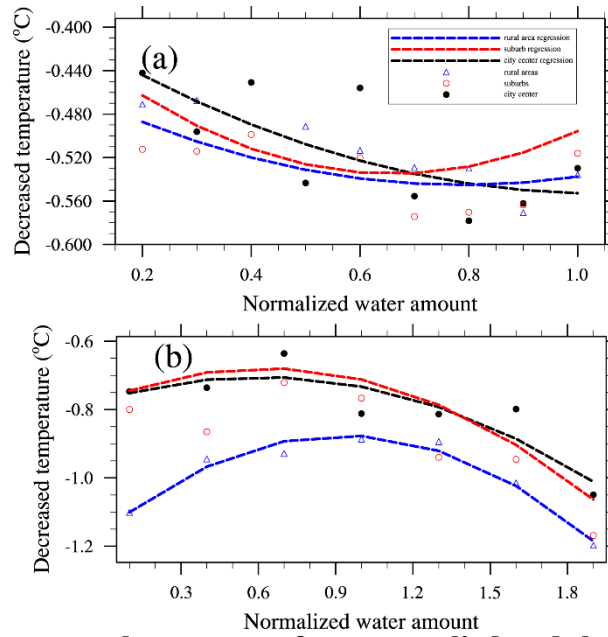
330 Figure 12. Relationships between the amount of water applied and the cooling effect: (a) for road sprinkling and (b) for urban irrigation. The black dots denote the cooling effect of water applied in the city center based on model simulations, red circles denote the cooling effect of water applied in suburbs based on model simulations, and blue triangles denote the cooling effect of water applied 335 in rural areas based on model simulations. The lines are polynomial regression curves, and black, red, and blue represent the city center, suburbs, and rural areas, respectively.
