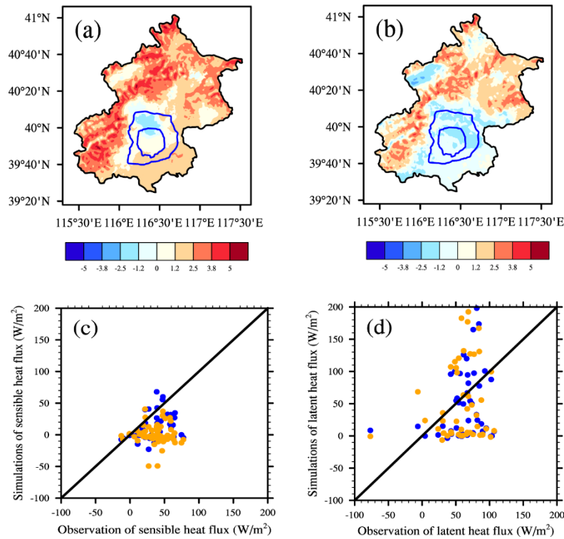
255 Figure 8. Comparisons between WRF simulations with and without water usage schemes. (a) temperature comparisons between CLDAS and WRF model simulations without urban water usage scheme, (b) temperature comparisons between CLDAS and WRF model simulations with urban water usage scheme, (c) sensible heat flux comparisons between station observation and simulation, (d) latent heat flux comparisons between station observation and simulation. Blue dots are the raw simulation results and orange dots are the simulation results with water usage schemes.
