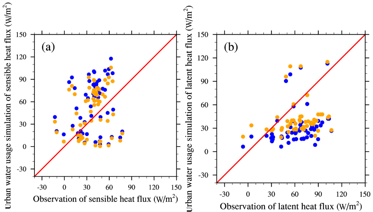
225 Figure 6. (a) Comparisons of sensible heat flux and (b) latent heat flux according to station observations and water usage simulations (including water irrigation and road sprinkling). Blue dots are the raw simulation results and orange dots are the water usage simulation results.
