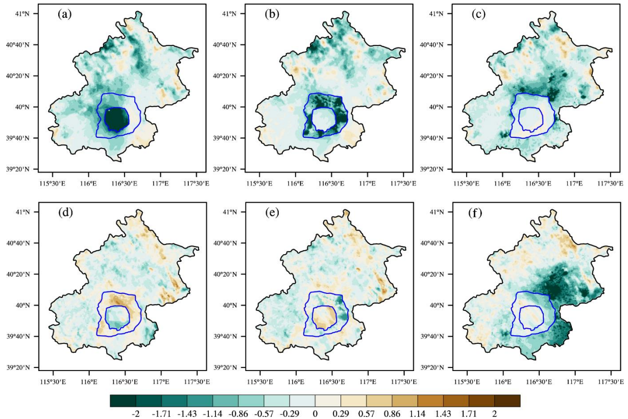
280 Figure 10. Cooling effects in the city center, suburbs, and rural areas due to urban irrigation during the day and night. (a) Cooling effect of urban irrigation in city center during the day. (b) Cooling effect of urban irrigation in suburbs during the day. (c) Cooling effect of urban irrigation in rural areas during the day. (d) Cooling effect of urban irrigation in city center during the night. (e) Cooling effect of urban irrigation in suburbs during the night. (f) Cooling effect of urban irrigation 285 in rural areas during the night. The amount of water was the estimated urban irrigation.
