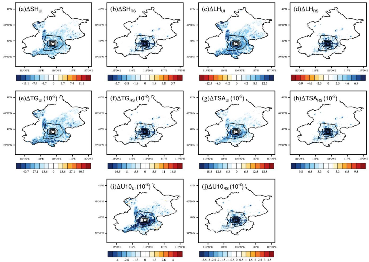
Figure 5. Changes in land surface variables due to urban irrigation (UI) and road sprinkling (RS). (a) Sensible heat flux under UI, (b) sensible heat flux under RS, (c) latent heat flux under UI, (d) latent heat flux under RS, (e) ground temperature under UI, (f) ground temperature under RS, (g) air temperature under UI, (h) air temperature under RS, (i) 10-m wind speed under UI, and (j) 10-m wind speed under RS.
