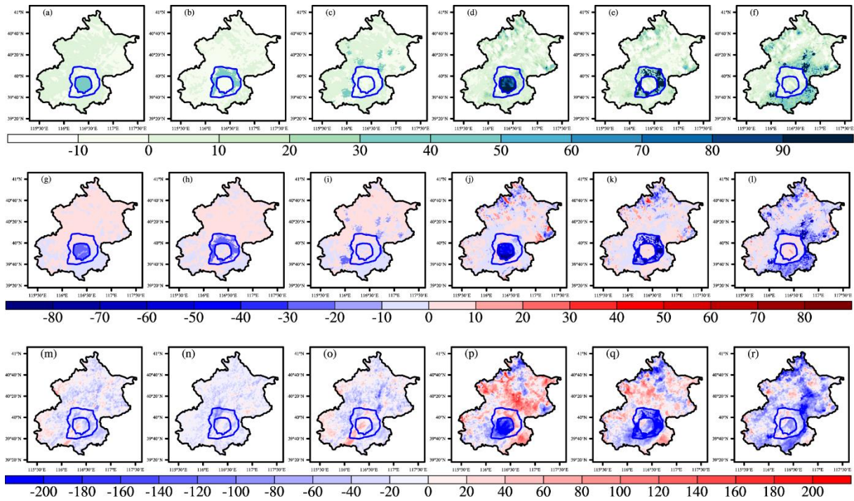
295 Figure 11. Changes in the latent heat flux, sensible heat flux, and boundary layer height due to road sprinkling and urban irrigation. (a) Changes in latent heat flux (LH) due to road sprinkling in the city center. (b) Changes in LH due to road sprinkling in the suburbs. (c) Changes in LH due to road sprinkling in rural areas. (d) Changes in LH due to urban irrigation in the city center. (e) Changes in the LH due to urban irrigation in suburbs. (f) Changes in LH due to urban irrigation in rural areas. (g)–(l) Changes in sensible heat flux in a similar manner to (a)–(f). (m)–(r) Changes in the boundary layer height in a similar manner to (a)–(f). 300
