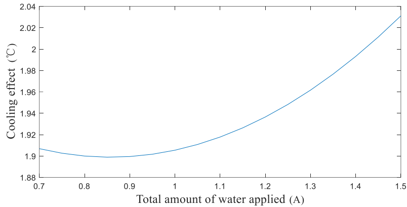
Figure 13. Sensitivity analysis based on the total amount of water applied and the cooling effect.
