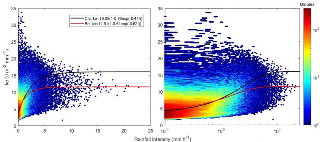
Fig. 2. (new Figure 4 in manuscript). Minutes number per intensity class (x-axis) and k_e class (y-axis) with fitted k_e - I curves at Bristol station (2015–2018), plotted on linear (left) and logarithmic (right)
