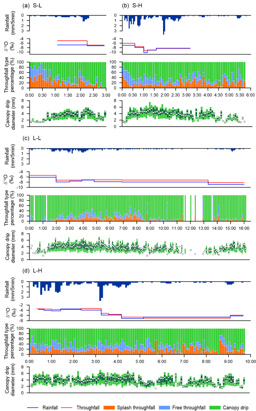
Figure 5. Temporal evolution of rainfall dynamics (5-min time step), \delta^{18}\text{O} in rainfall and in throughfall isotopic composition ( \delta^{18}\text{O} collected by the sequential samplers every 5 mm of rainfall), throughfall type percentages based on volume, and drop diameter of canopy drip for (5-min time step): a) short duration-low intensity event (S-L), b) short duration-high intensity event (S-H), c) long duration-low intensity event (L-L), and d) long duration-high intensity event (L-H). The drop diameter is
