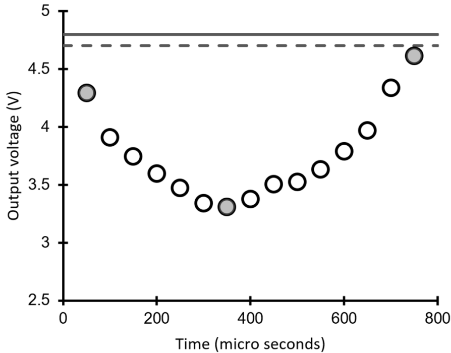
Figure A1. An example of temporal variation of output voltage by a drop passed through the laser beam. The solid line denotes base voltage, the dashed line denotes threshold voltage, the open circle denotes output voltage every 50 microseconds and the closed circle denotes the data recording onto the Arduino.
