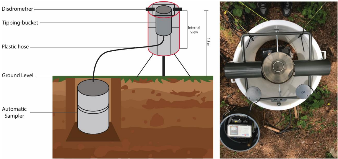
690 Figure 2. Setup for continuous measurement and sampling of open rainfall and throughfall. Diagram of the experimental equipment (left) and top view of the equipment installed in the forest stand (right).
