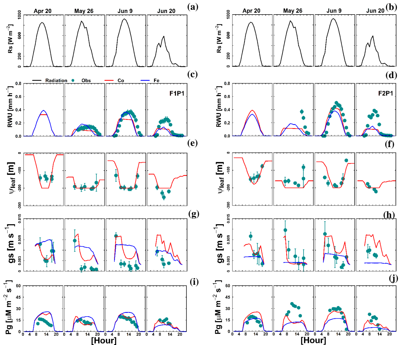
Figure 9: Diurnal courses of 4 selected measurement days: 20 April, 26 May, 9 June, and 20 June 2016 (a & b) global radiation ( R_s ) (c & d) actual transpiration (RWU), (e & f) leaf water pressure head ( \psi_{\text{leaf}} ), (g & h) stomatal conductance to water vapor ( g_s ), and (i & j) gross assimilation rate ( P_g ) at the sheltered plot (P1) of the stony soil (F1) and the silty soil (F2). The cyan dots, solid red lines, and solid blue lines denote the observed, simulated values from the Couvreur model (Co), and Feddes (Fe), respectively. Sap flow sensors were installed on 26 May 2016 at 9 AM and 5 PM for F1P1 and F2P1, respectively. Simulated stomatal conductance are from sunlit leaves. The Feddes RWU model did not simulate leaf water pressure head.
