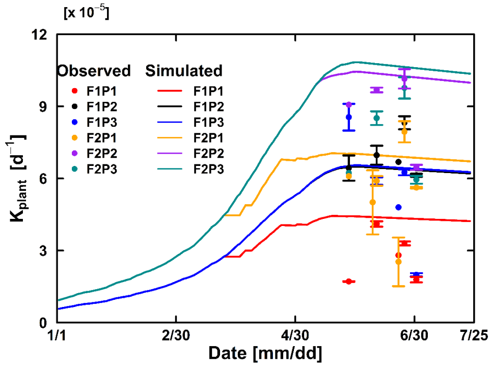
1045 Figure 10: Comparison between observed (dot) and simulated plant hydraulic conductance (solid line) by the Couvreur (Co) model in the sheltered (P1), rainfed (P2), and irrigated (P3) plots of the stony soil (F1) and the silty soil (F2). The vertical bars represent the standard deviation of 6 hourly plant hydraulic conductance values at around midday (11 AM to 4 PM) in the measurement day. Note: crop germination was on 26 th October 2015, data is showed here from 1 January 2016 to harvest 23 July 2016. Blue line was overlapped by the black line
