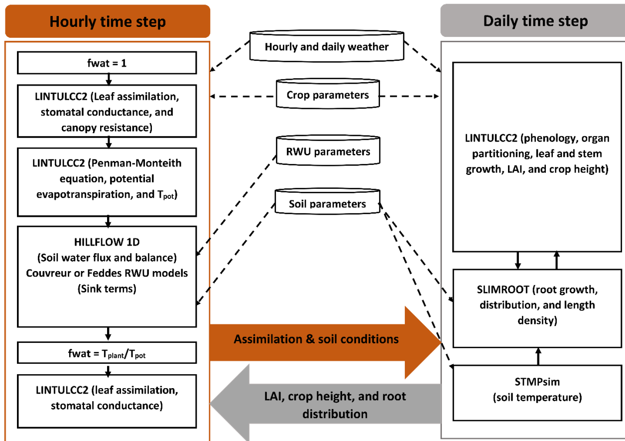
885 Figure 2: Description of the coupled root: shoot models in the study. The orange arrow indicates feedbacks from the hourly simulations to daily simulation while the grey arrow indicates feedbacks from the daily simulations to the hourly simulations. The dashed black arrows denote the weather input and parameters to the subroutines. The continuous black arrows indicate the links amongst the modelling subroutines.
