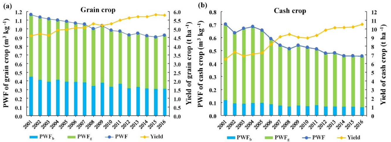
745 Figure 2: Interannual variability of national average production-based water footprint (PWF) of (a) grain and (b) cash crops in 746 China over 2001-2016.
