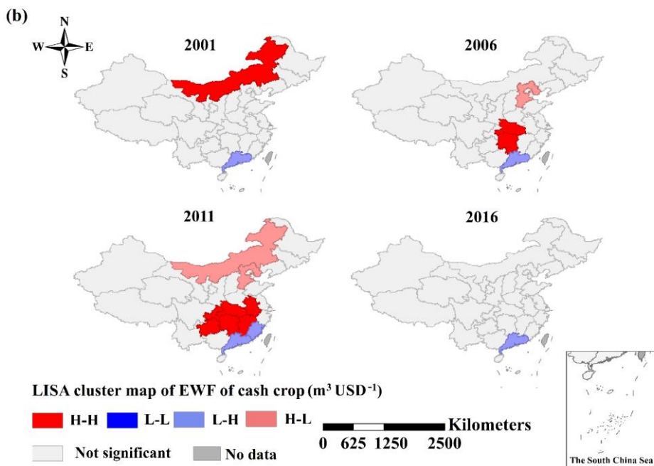
757 Figure 7: The LISA cluster maps of economic value-based water footprint (EWF) of (a) grain and (b) cash crops.
