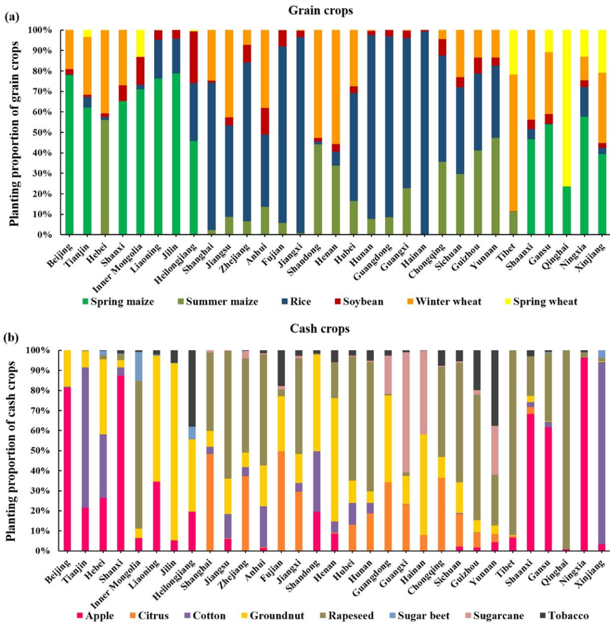
764 Figure 10: Planting structure of (a) grain and (b) cash crops in 31 provinces in 2016.
