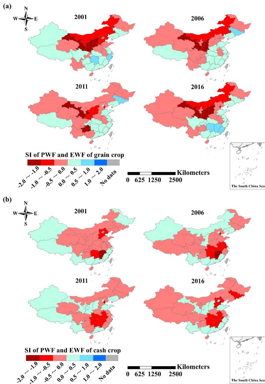
759 Figure 8: Temporal and spatial evolution of synergy evaluation index (SI) of (a) grain and (b) cash crops.
