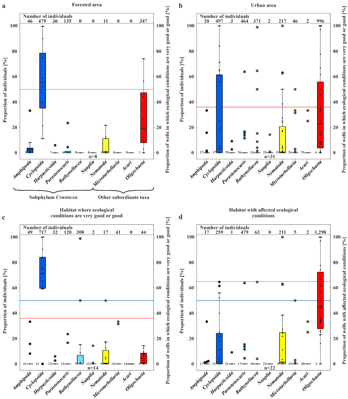
290 Figure 4: Boxplots of the amount of fauna [%]: (a) proportion of individuals and of wells in which ecological conditions are very 295 good or good (secondary axis) [%] of the forested area; (b) proportion of individuals and of wells in which ecological conditions are very good or good [%] of the urban area; (c) proportion of individuals and of wells in which ecological conditions are very good or good [%] divided based on the results of the classification scheme by Griebler et al. (2014); (d) proportion of individuals and of wells with affected ecological conditions [%] divided based on the results of the classification scheme by Griebler et al. (2014). The colour of the boxes shows the different taxa in the samples. (n = number of wells)
