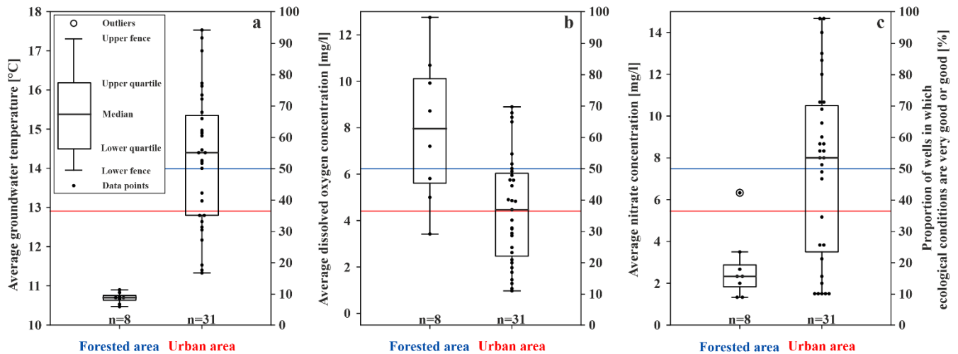
230 Figure 3: Boxplots of the physical and chemical parameters for the forested and urban area in the study site and the proportion of wells in which ecological conditions are very good or good in percentage [%] indicated by the blue (forested area) and red (urban area) lines (secondary axis); (a) average temperature of the repeated measurements [°C] at the bottom of the monitoring wells; (b) average content of dissolved oxygen [mg/l] of the monitoring wells; (c) average nitrate content [mg/l] of each monitoring well. (n = number of wells)
