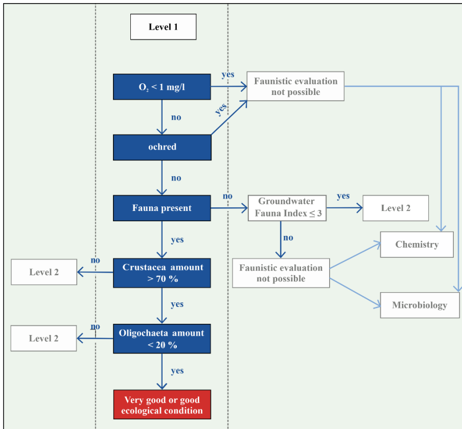
205 Figure 1: Classification scheme by Griebler et al. (2014) according to Level 1 for groundwater ecosystems on the basis of groundwater fauna (modified after Griebler et al. (2014)).
