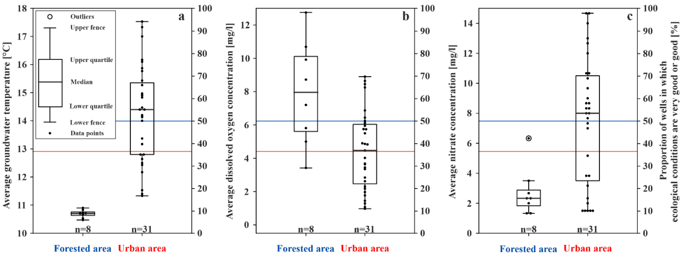
Figure 3: Boxplots of the physical and chemical parameters for the forested and urban area in the study site and the proportion of wells in which ecological conditions are very good or good in percentage [%] indicated by the blue (forested area) and red (urban area) lines (secondary axis); (a) average temperature of the repeated measurements [°C] at the bottom of the monitoring wells; (b) average content of dissolved oxygen [mg/l] of the monitoring wells; (c) average nitrate content [mg/l] of each monitoring well. (n = number of wells)
