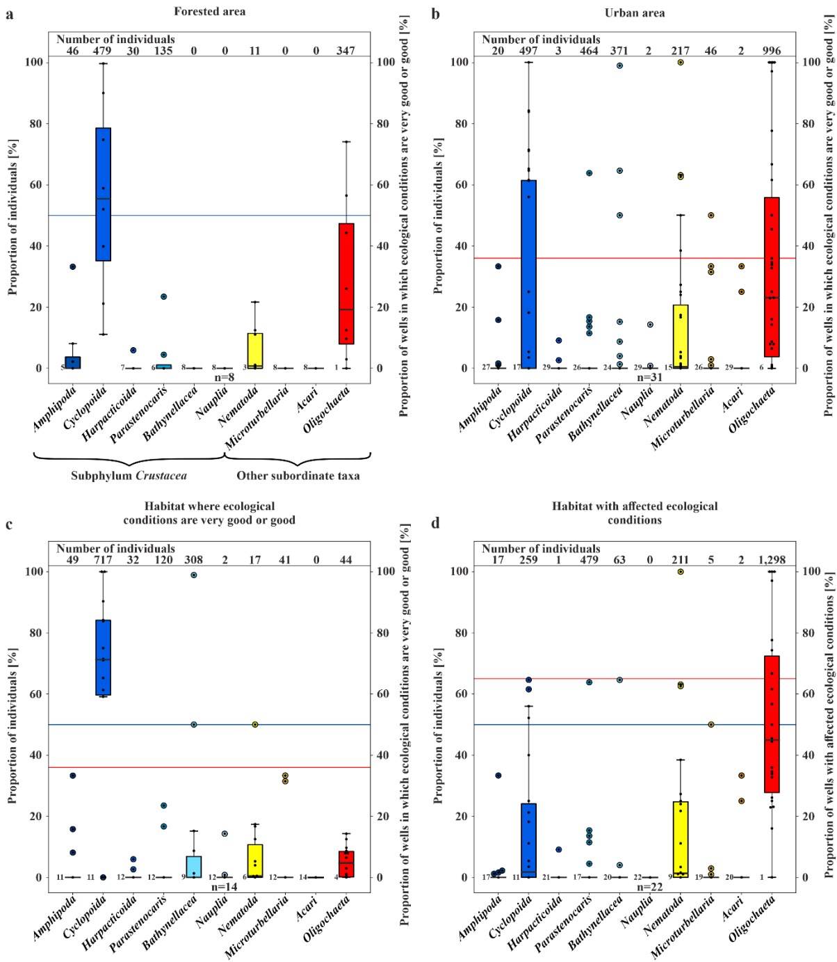
Figure 4: Boxplots of the amount of fauna [%]: (a) proportion of individuals and of wells in which ecological conditions are very good or good (secondary axis) [%] of the forested area; (b) proportion of individuals and of wells in which ecological conditions are very good or good [%] of the urban area; (c) proportion of individuals and of wells in which ecological conditions are very good or good [%] divided based on the results of the classification scheme by Griebler et al. (2014); (d) proportion of individuals and of wells with affected ecological conditions [%] divided based on the results of the classification scheme by Griebler et al. (2014). The colour of the boxes shows the different taxa in the samples. (n = number of wells)
