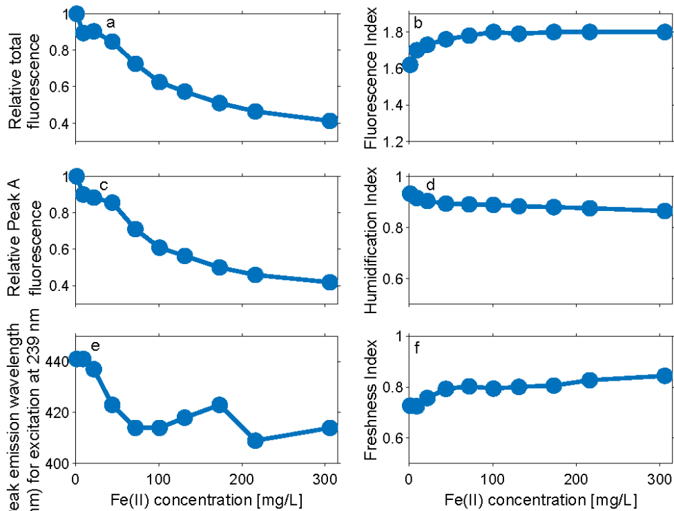
Figure 4: Effect of varying Fe(II) concentrations at pH 7.4 on: a) relative total fluorescence intensity ( OFI/OFI_0 ); c) relative fluorescence intensity of Peak A ( A/A_0 ) and e) peak fluorescence emission wavelength (nm) at excitation at 239 nm (peak A). Effect of varying Fe(II) concentration at pH 7.4 on various indices: b) fluorescence index (FI), d) humidification index (HIX), and f) freshness index (FrI). The results show that the fluorescence intensities, indices and peak emission wavelength change as Fe(II) is increased from 1 to 306 mg/L.
