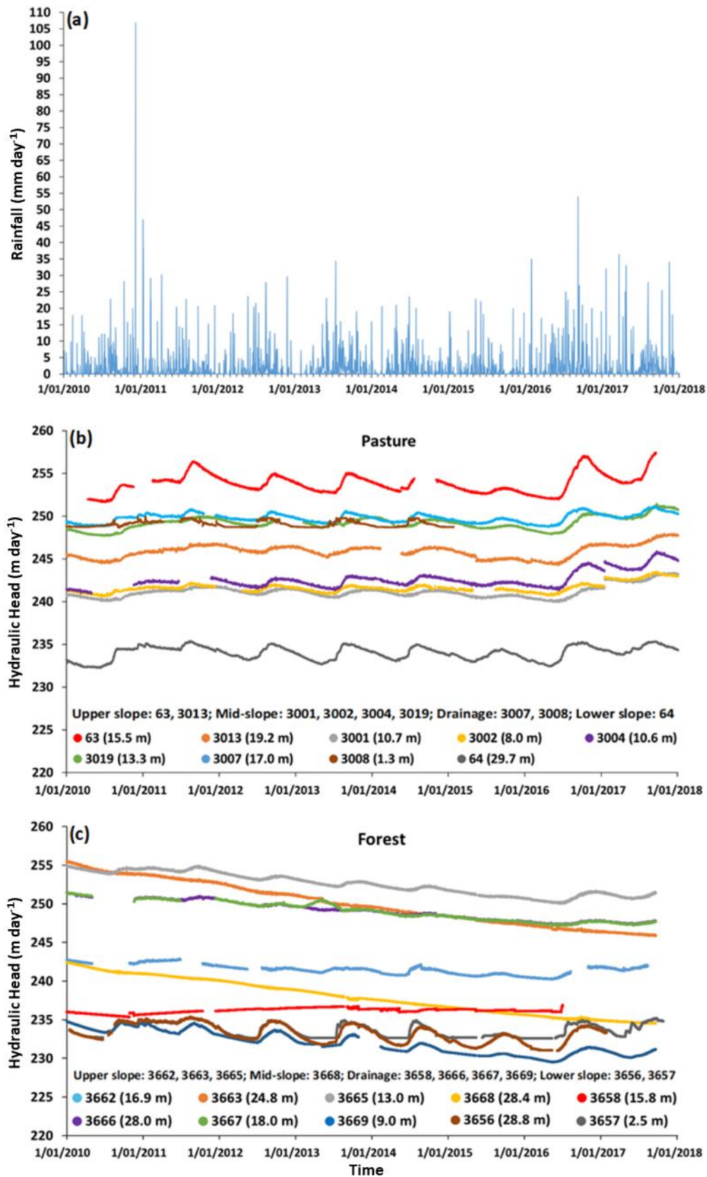
905 Figure 3: (a) Daily rainfall at Cavendish (Station 089009: ~19 km southeast of Gatun). Variation in groundwater heads from bores in (b) pasture and (c) forest (Dresel et al., 2018). The legend shows the sample depths (in parentheses) and landscape positions.
