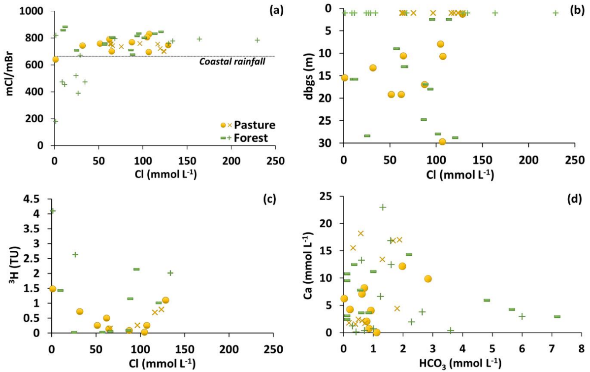
910 Figure 4: (a) Variation of molar Cl/Br ratios with molar concentrations of Cl. (b) Molar Cl concentrations across depth below ground surface (dbgs: m). (c) 3 H (TU) vs. molar Cl concentrations. (d) Molar Ca vs. HCO 3 concentrations. Cross and plus symbols are for the shallow riparian groundwater and other symbols are for the regional groundwater.
