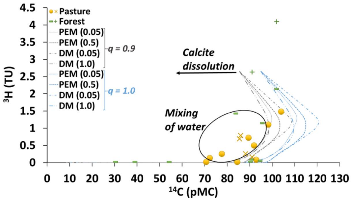
915 Figure 5: Activities of ^3\text{H} (TU) and ^{14}\text{C} (pMC) in the pasture and forest groundwater. PEM = partial exponential model (PEM ratio in brackets) and DM = dispersion model (DP parameter in brackets). Cross and plus symbols are for the shallow riparian groundwater and other symbols are for the regional groundwater. The single high ^3\text{H} activity possibly reflects recharge by winter rainfall. Samples lying to the left of the covariance curves probably record mixing between younger and older groundwater (see text for discussion).
