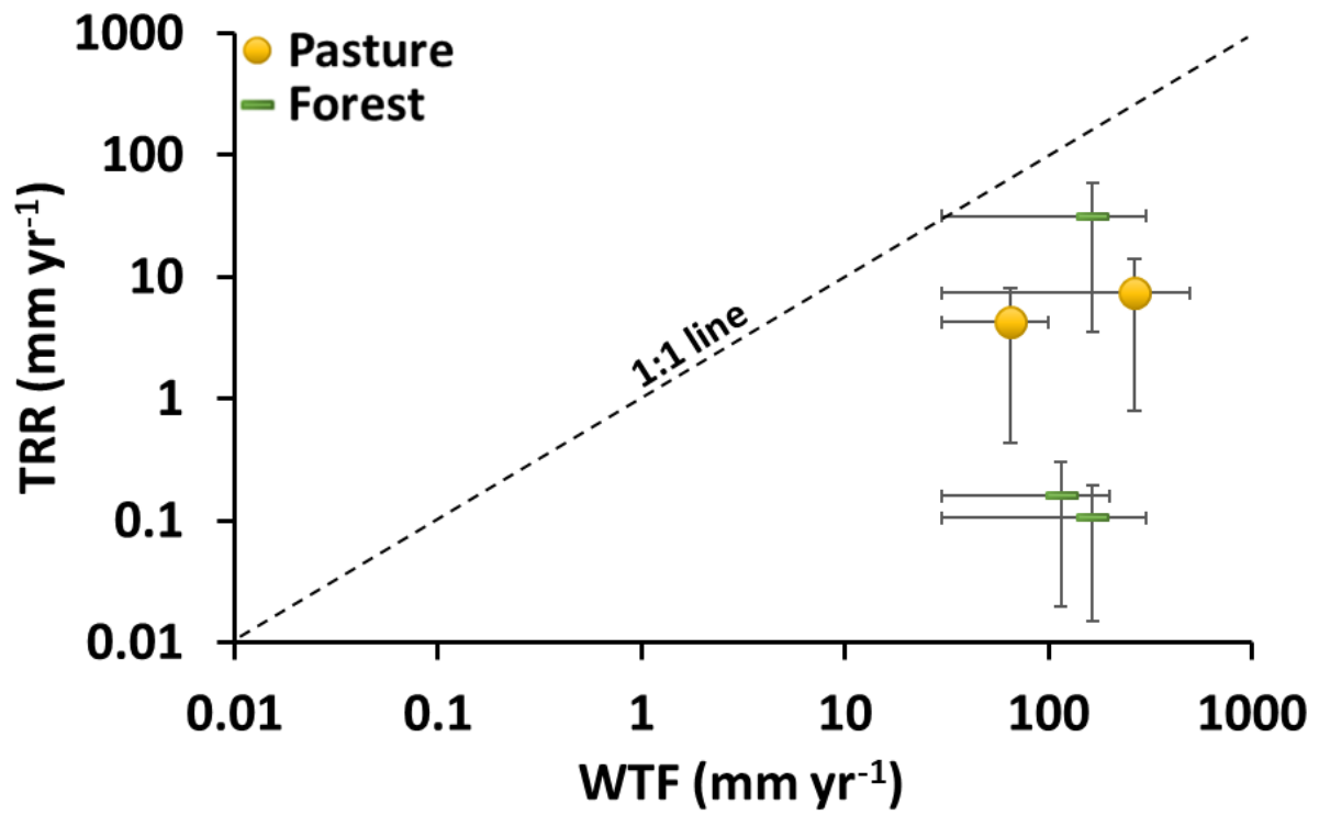
915 Figure 8: Comparison between recharge rates for the regional groundwater estimated from WTF and TRR. Bars represent the ranges of calculated recharge values from Table 1.
