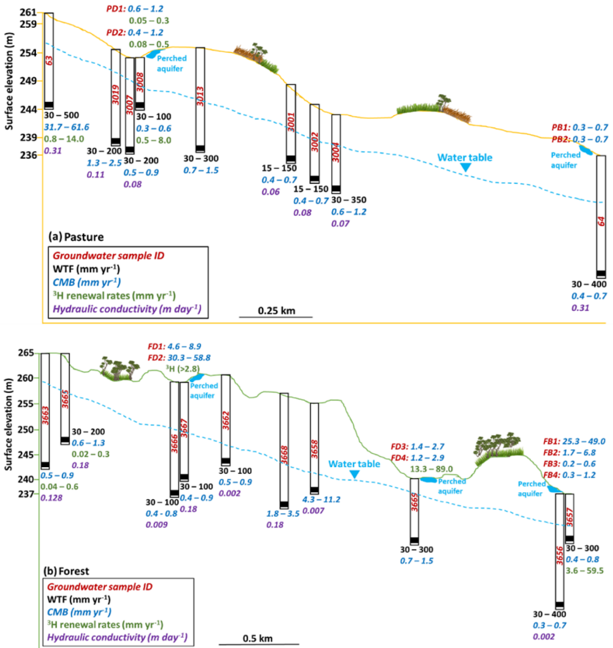
880 Figure 2: Simplified cross sections of (a) pasture and (b) forest catchments showing variability of groundwater recharge estimated via WTF, CMB, 3 H methods and variable hydraulic conductivity of the aquifer lithologies. Transects are on Fig. 1a. PD and FD represent the shallow groundwater in the pasture drainage and forest drainage areas, respectively. Data from Table 1.
