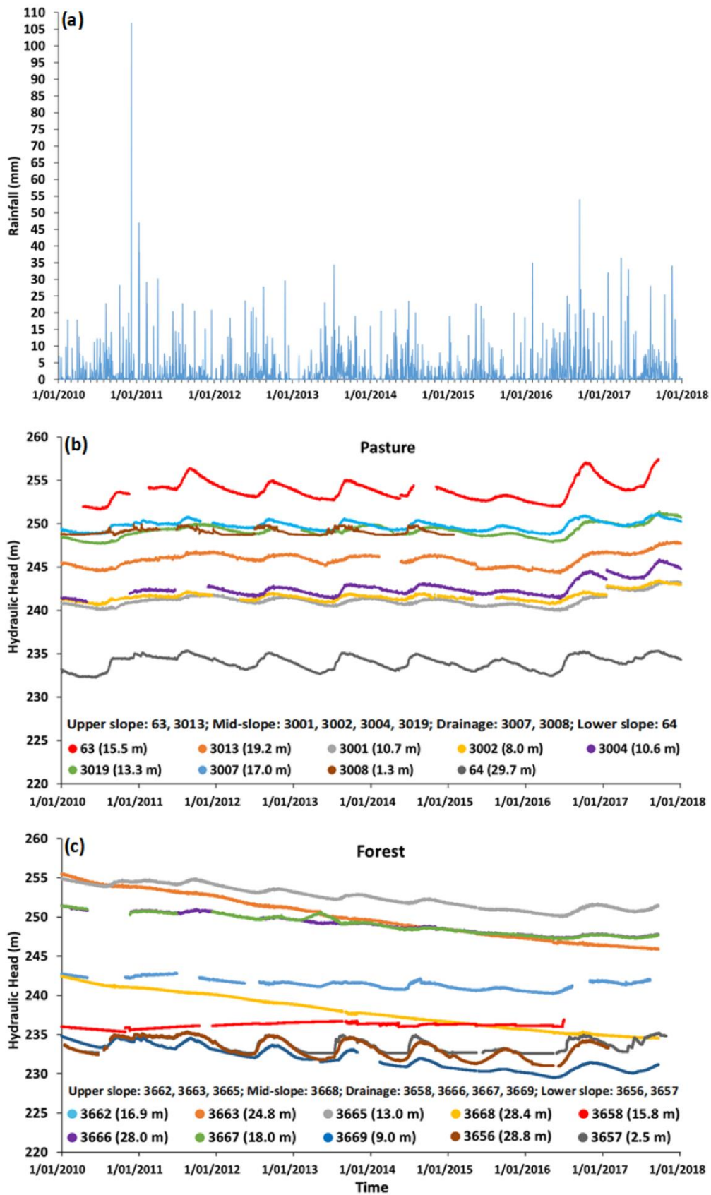
Figure 3: (a) Daily rainfall at Gatam. Variation in groundwater heads from bores in (b) pasture and (c) forest (Dresel et al., 2018). The legend shows the sample depths (in parentheses) and landscape positions.
