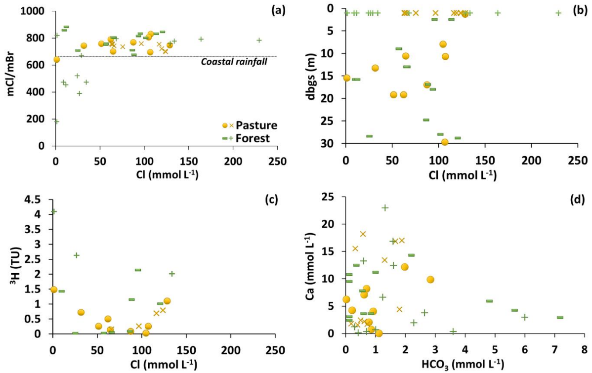
890 Figure 4: (a) Variation of molar Cl/Br ratios with molar concentrations of Cl. (b) Molar Cl concentrations across depth below ground surface (dbgs: m). (c) 3 H (TU) vs. molar Cl concentrations. (d) Molar Ca vs. HCO 3 concentrations. Cross and plus symbols are for the shallow riparian groundwater and other symbols are for the regional groundwater.
