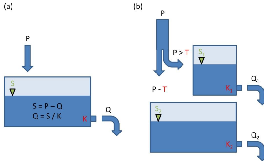
Figure 2. (a): Model-02, a single linear reservoir with state variable S and retention constant K . The reservoir is replenished by precipitation P and drained by discharge Q . (b): Model-03, with two linear reservoirs. Precipitation input is split by intensity threshold T .
