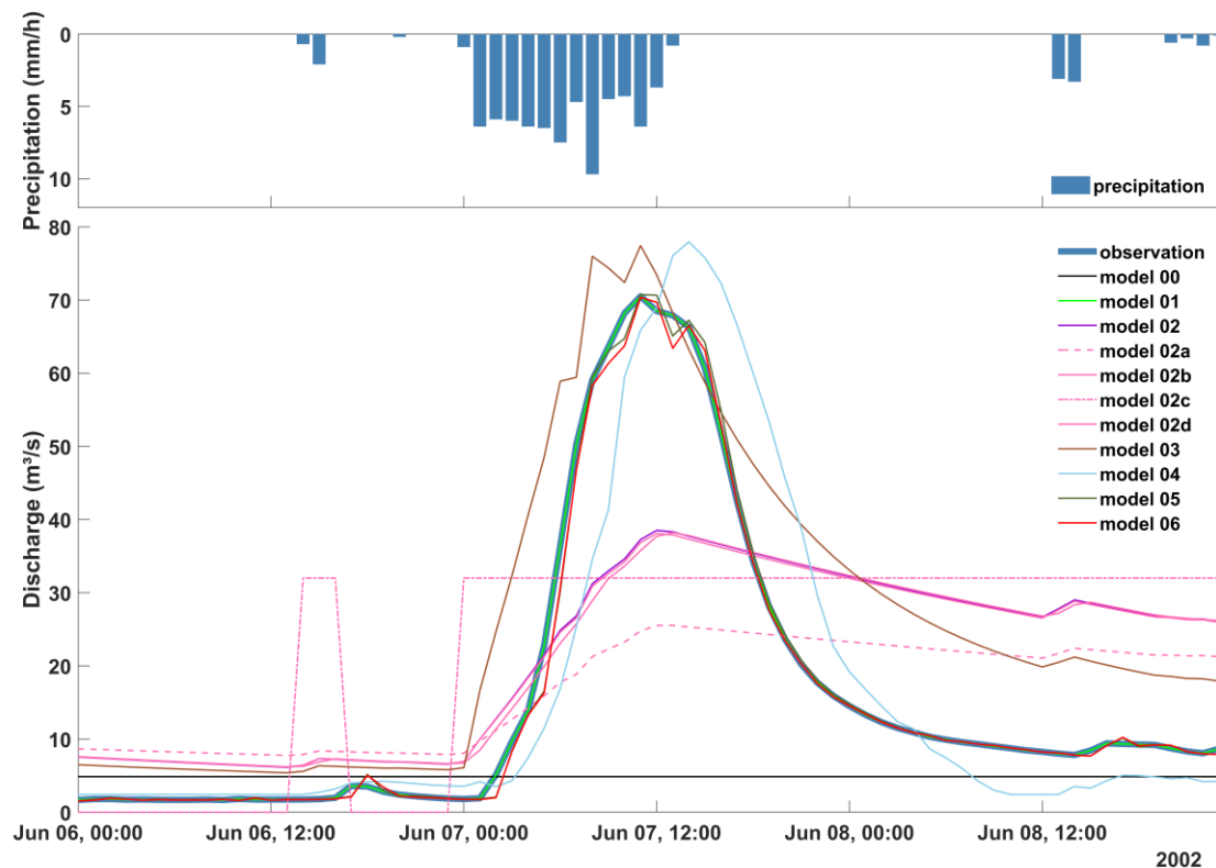
Figure 3. Top: Observed precipitation at Ebnet. Bottom: Observed discharge at gauge Hoher Steg and simulations thereof by Model-00 to Model-06 for a rainfall-runoff event in June 2002.
