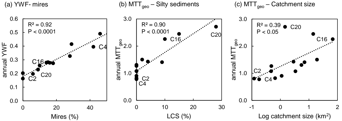
440 Figure 8: Catchment characteristics are important for travel times. The figure shows the annual averages: (a) the areal coverage of mires and the young water fraction (YWF), (b) areal coverage of silt and MTT_{geo} , and (c) catchment size and MTT_{geo} .
