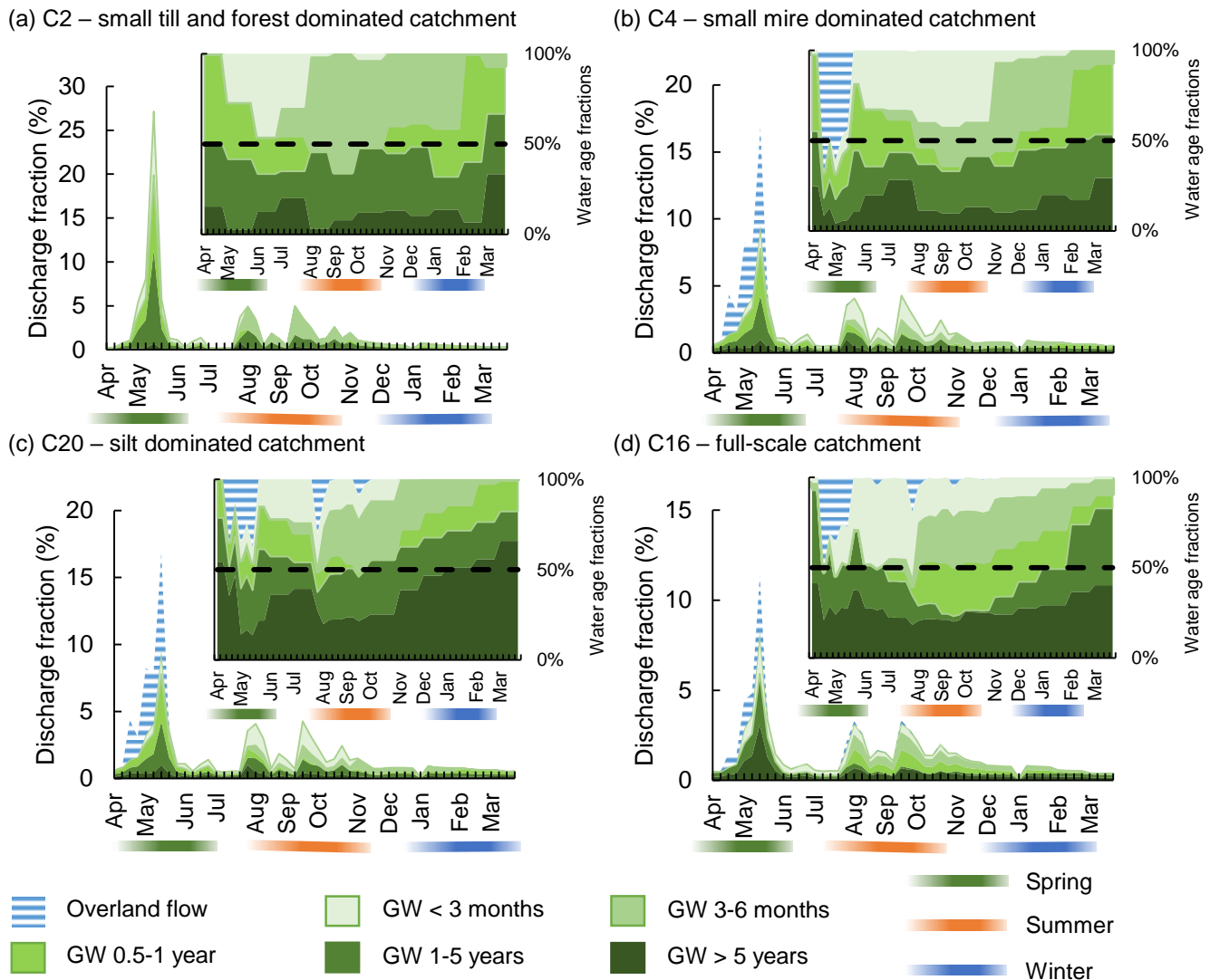
395 Figure 6: Seasonal fraction of discharge to streams. The figure shows the proportion of annual stream discharge arriving as groundwater and overland flow. Four sub-catchments are exemplified, including (a) the small till and forest dominated C2, (b) the small mire dominated C4, (c) the silt dominated C20, and (d) the full-scale Krycklan catchment C16 with mixed mires and forests (extended version in Appendix Fig. A1). The figure showcases the travel time fraction of water discharging to the streams. The fractions are both shown as part of the total annual discharge as well as the water composition. The bands below the months highlight the three investigated seasons, spring, summer, and winter. 400
