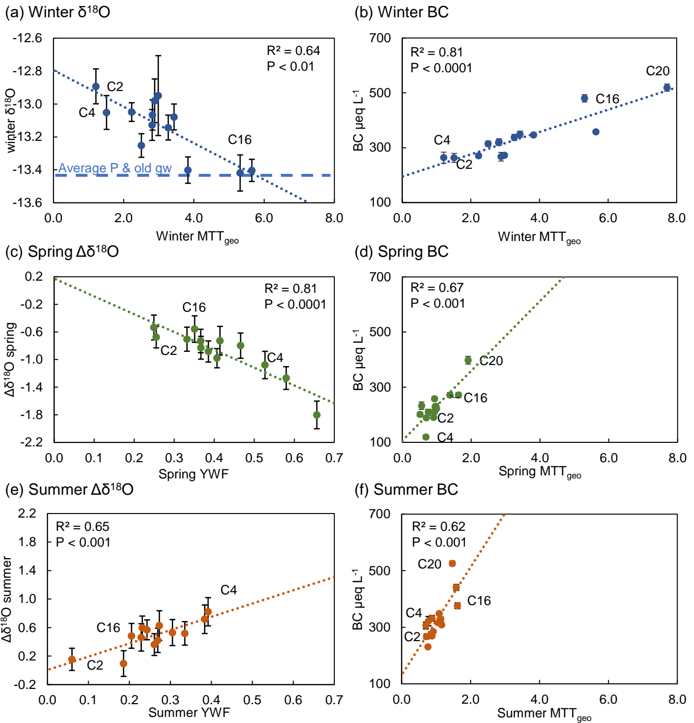
Figure 7: Relationships of seasonal MTT geo and young water fractions (YWF) with seasonal stream isotopic composition and base cation concentration. Note that δ 18 O results are for 13 sites, while the BC record comprises all 14. The sub-plots (a) to (f) show the δ 18 O (winter) or Δδ 18 O spring/summer and BC concentrations as a function of the MTT geo in winter, spring, and summer, respectively. The standard error of the mean (SEM) shown as whiskers denotes variations in field observations.
