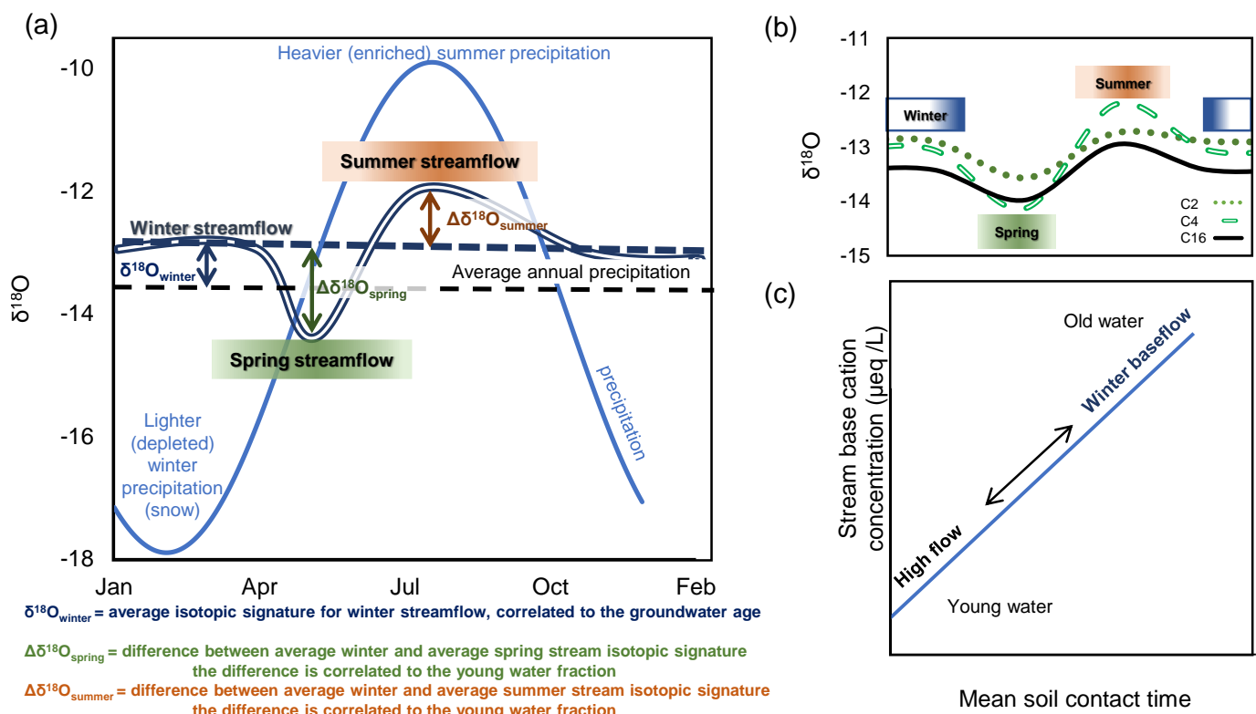
220 Figure 2: Conceptual figure of travel time to stream vs stream isotopic signature (a and b), and stream base cation concentration (c).
