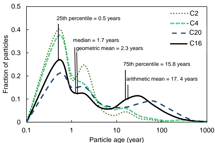
Figure 5: Examples of particle tracking results. The figure shows the agedistribution of all particles reaching sub-catchment outlets the different streams for the entire modelling period . The solid line shows the statistics for C16, including the 25th percentile, the median, the geometric mean, the arithmetic mean, and the 75th percentile (Appendix, A1). Moreover, the figure shows three other example distributions, including C2 (small forest and till dominated catchment), C4 (small mire dominated catchment), C20 (small silt dominated catchment).
