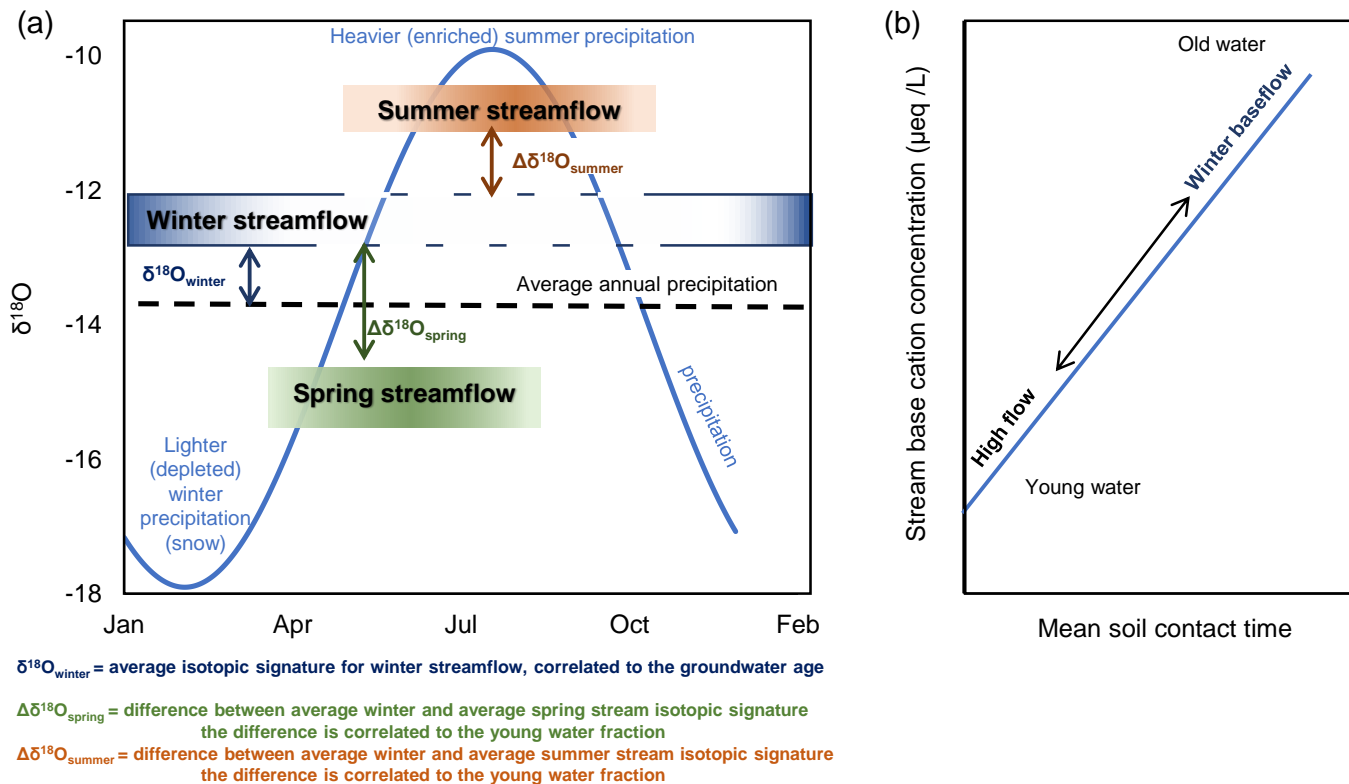
Figure 2: Conceptual figure of stream-water-travel time to stream vs. stream isotopic signature (a) and stream base cation concentration (b). (a) The connection between \delta^{18}\text{O} and stream-water-travel time to stream, where the sine curve shows the annual variations of \delta^{18}\text{O} in precipitation, and approximate seasonal winter, spring, and summer stream compositions are marked. In winter, the travel times are related to the deviation in the isotopic signature between the winter baseflow and the long-term precipitation. In spring, the fraction of young water is correlated to the difference between the spring stream signature and the winter baseflow. In summer, the fraction of young water is correlated to the difference between the stream signature and winter baseflow. (b) The connection between base cation (BC) concentration and soil contact time. The longer time the water spent in the mineral soil, the higher the stream concentrations of BCs will be due to soil weathering.
