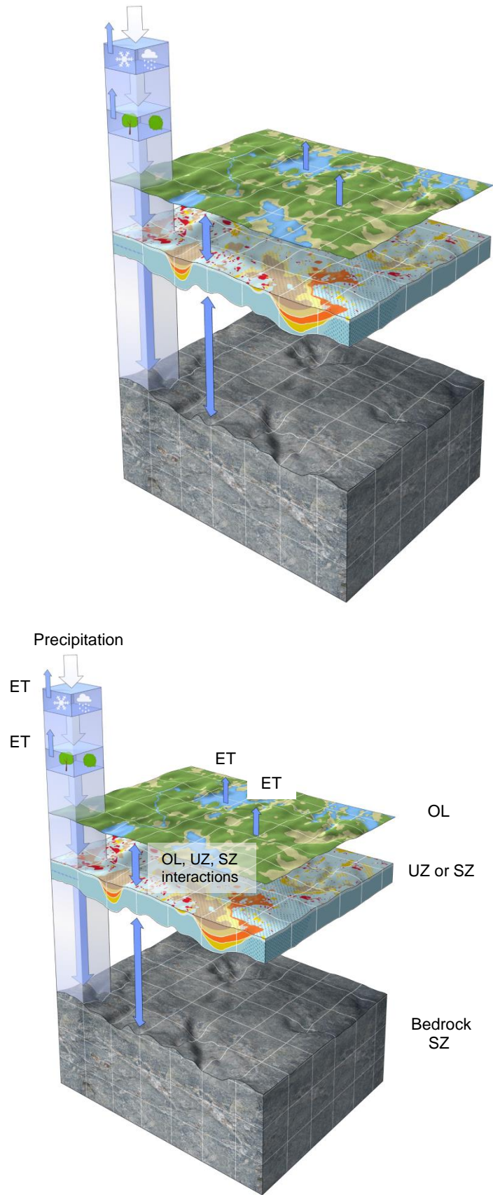
Figure 3: Schematic of a general Mike SHE model set up. Precipitation falls on the ground as rain or snow. Evapotranspiration (ET) processes include canopy interception, open surface evaporation, root uptake, and soil evaporation from the unsaturated zone (UZ). The overland flow
