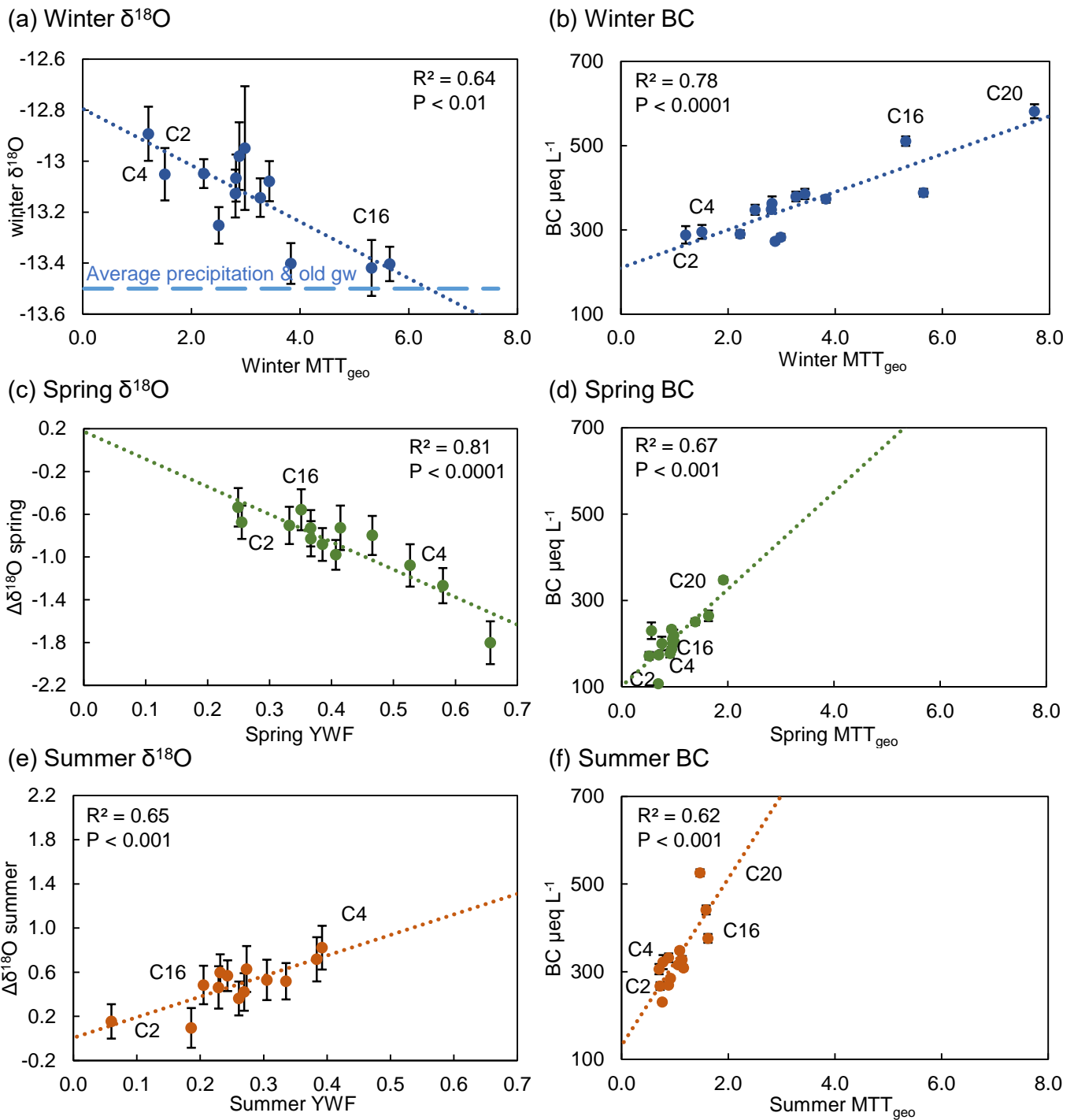
Figure 7: Relationships of seasonal \text{MTT}_{\text{geo}} and young water fractions (YWF) and \text{MTT}_{\text{geo}} compared to with seasonal stream isotopic composition and base cation concentration. Note that \delta^{18}\text{O} results are for 13 sites, while the BC record comprises all 14. The subplots (a) to (f) show the \delta^{18}\text{O} (winter) or \Delta\delta^{18}\text{O}_{\text{spring/summer}} and BC concentrations as a function of the \text{MTT}_{\text{geo}} in winter, spring, and summer, respectively. The standard error of the mean (SEM) shown as whiskers denotes variations in field observations.
