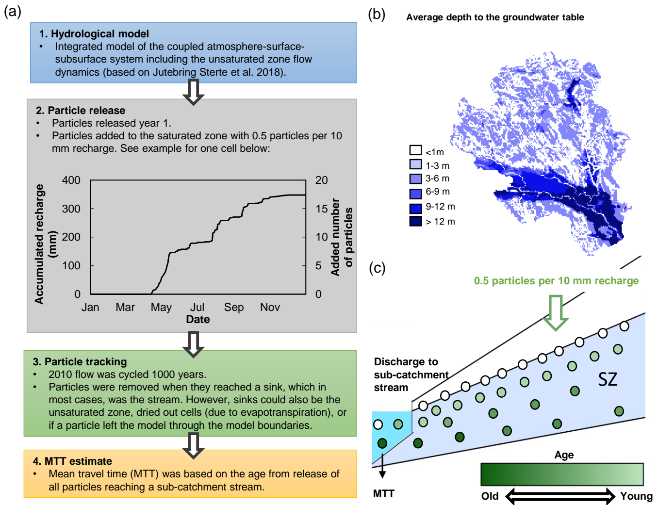
Figure 4: Particle model setup. (a) Steps of particle tracking (b) Average depth to the groundwater table. The main part of the model area has a calculated depth to the groundwater table between 0-3 m and varied daily. (c) Schematic illustration of particle tracking set up. Particles were added to groundwater recharge at the transient groundwater table. The age of these particles was zero at the time of recharge, then . Thereafter , they followed the groundwater flow resulting in , increasing in age until reaching a stream or lake.
