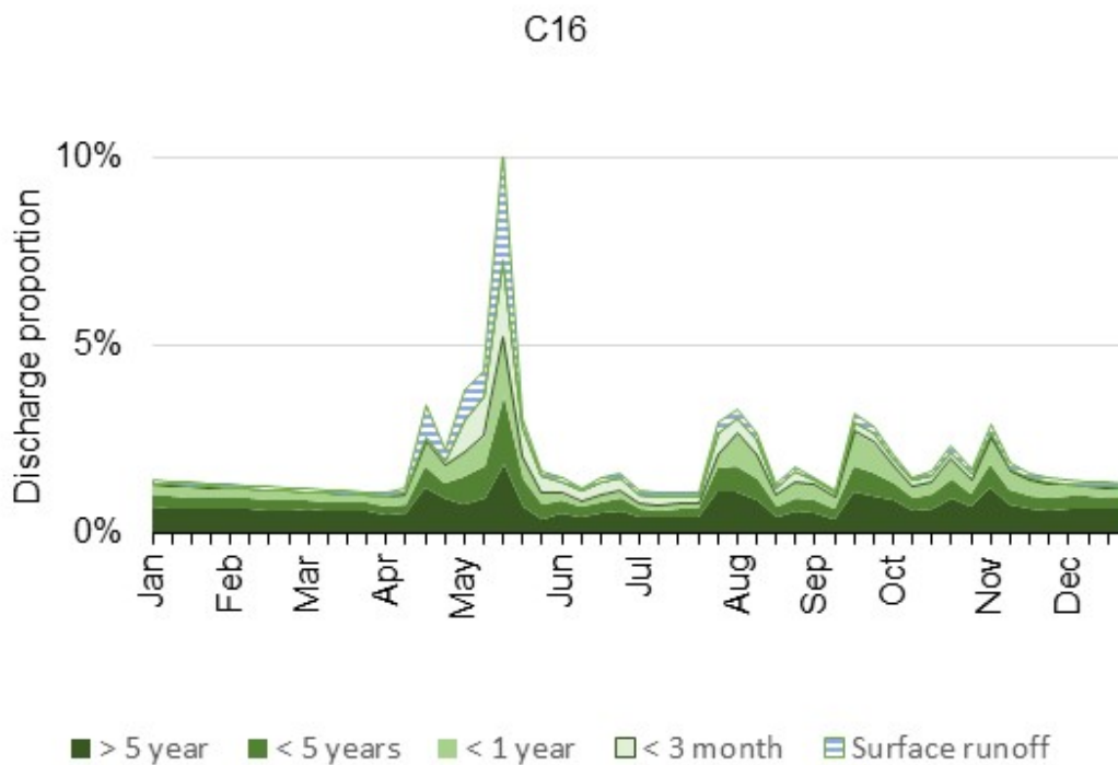
Fig. 6. Discharge distribution
