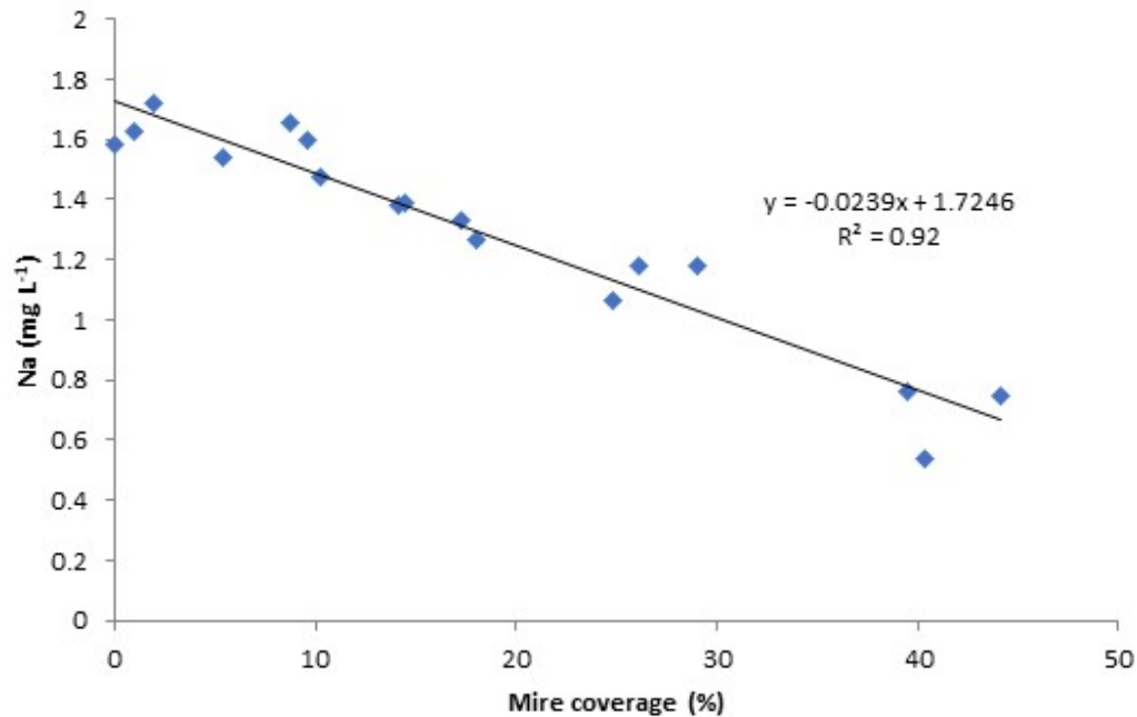
Fig. 3. Na concentrations
