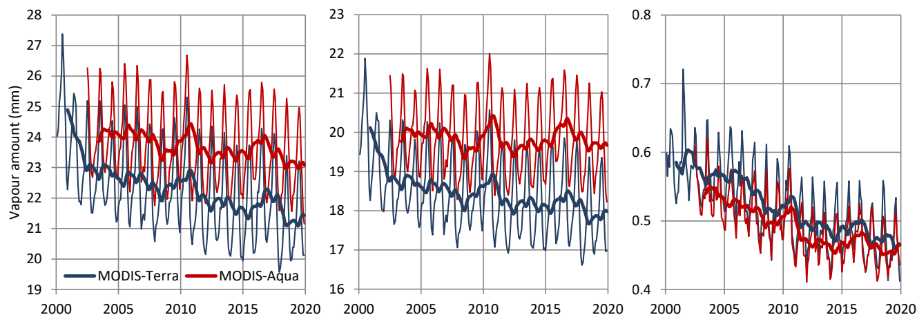
Figure 8: Variation of water vapour amount as in Figure 7 but only for the MODIS data set and separately for the Terra and Aqua platforms: (left) total of the vertical column; (middle) from surface to 680 hPa; (right) from 440 to 10 hPa. Thin and thick lines of the same colour represent monthly values and running annual averages (right aligned), respectively. Sources of data are indicated in the legend and detailed in Table 1.
