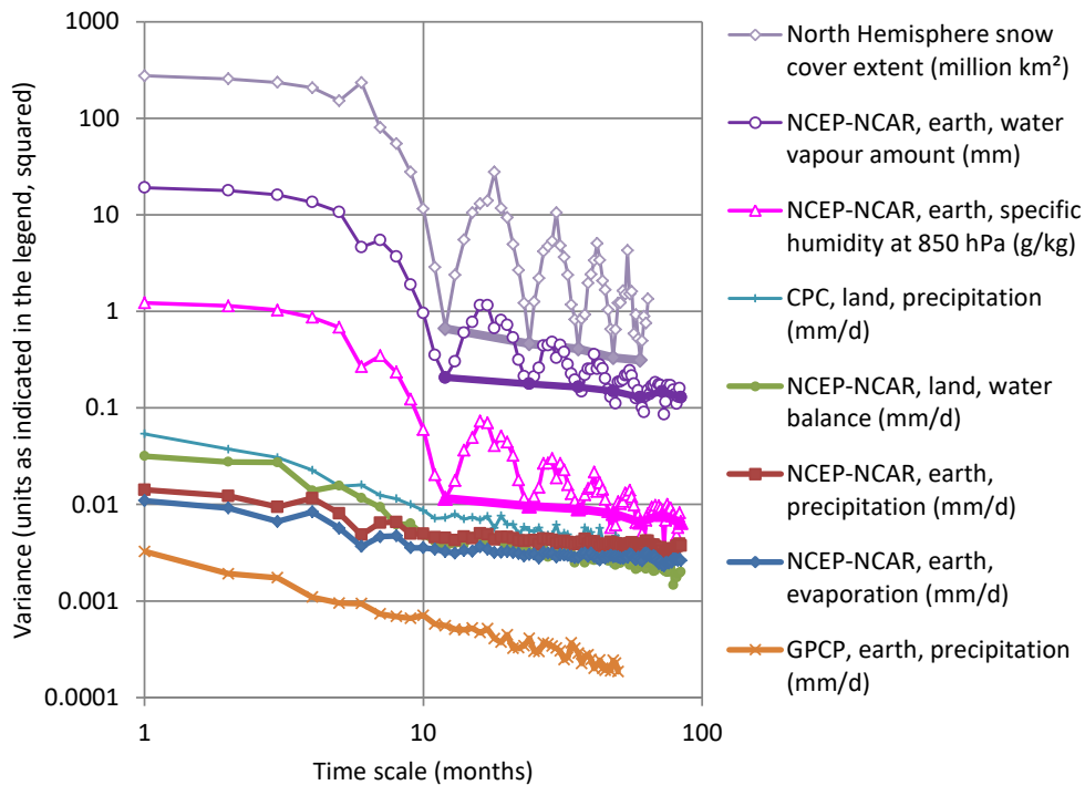
Figure 18: Climacograms of the indicated processes calculated from monthly time series; for some series with prominent seasonality the climacograms from annual time series are also plotted with thicker lines of same colour. For time scales larger than annually all slopes in the double logarithmic plots are close to -0.2 , suggesting a Hurst parameter 0.90 (or larger if bias is taken into account). Exceptions are the NH snow cover extent with a slope of -0.47 , suggesting a Hurst parameter 0.76 and the GPCP precipitation series with a slope of -0.72 , suggesting a Hurst parameter 0.64 .
