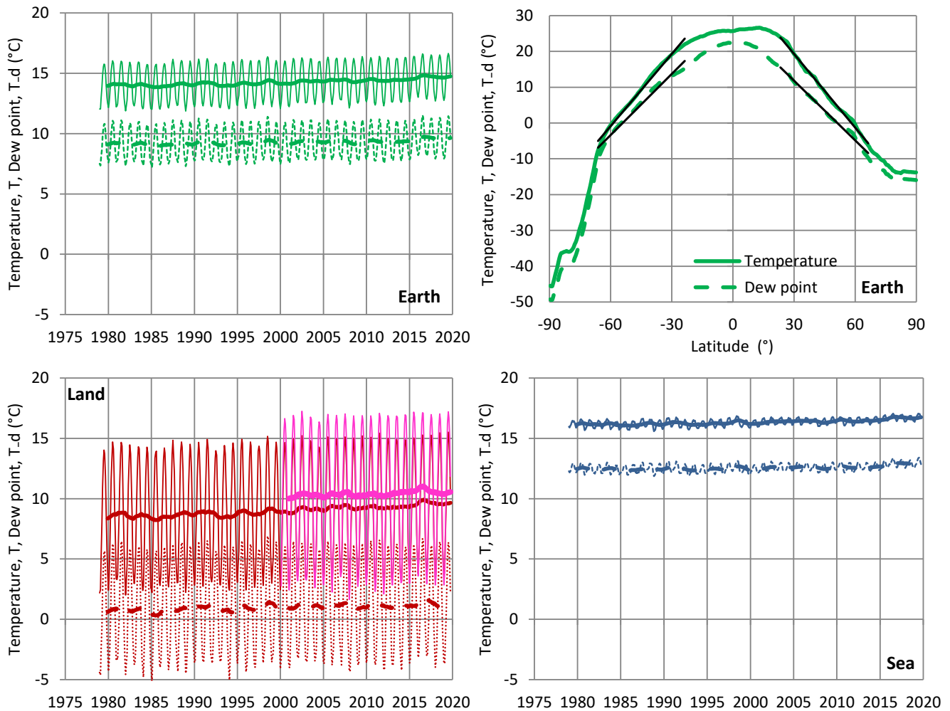
Figure 2: (Upper left) Variation of the globally averaged temperature (continuous lines) and dew point (dashed lines) at the level of 2 m above ground. Thin and thick lines of the same colour represent monthly values and running annual averages (right aligned), respectively. (Upper right) Zonal distribution of earth temperature and dew point; for the temperate zone ( \pm 23.5^\circ to \pm 66.5^\circ ) the fitted slopes are also plotted (in black), which are \pm 0.68^\circ\text{C}/^\circ and \pm 0.56^\circ\text{C}/^\circ , respectively. (Lower left and right) As upper left but for the land and sea parts. Sources of data: ERA5 reanalysis as detailed in Table 1; for comparison and validation, in the Land graph the MODIS-terra land-surface temperature (averages of daytime and nighttime datasets, available since 2000) is also plotted in magenta.
