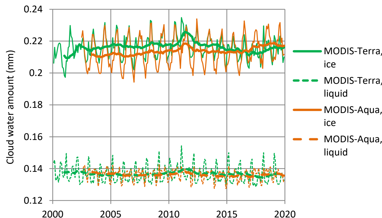
Figure 9: Variation of cloud water amount (in ice and liquid phase). Thin and thick lines of the same colour represent monthly values and running annual averages (right aligned), respectively. Sources of data are indicated in the legend and detailed in Table 1.
