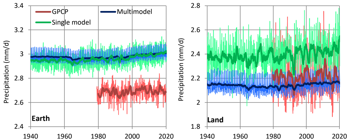
Figure 17: Comparison of climate model outputs (for specification of which see text) with reality, as quantified by GPCP satellite observations. “Multimodel” refers to CMIP5 scenario runs, entries: CMIP5 mean – rcp85. “Single model” refers to CCSM4 – rcp85, ensemble member 0, where CCSM4 stands for Community Climate System Model version 4, released by NCAR. Thin and thick lines of the same colour represent monthly values (but with rates expressed in \text{km}^3/\text{year} ) and running annual averages (right aligned), respectively.
