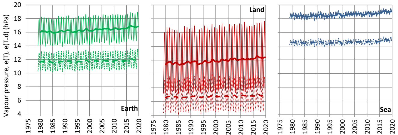
Figure 4: Variation of the saturation water pressure e(T) (continuous lines) and e(T_d) (dashed lines) for the average temperature T and dew point T_d as shown in Figure 2. Thin and thick lines of the same colour represent monthly values and running annual averages (right aligned), respectively. Sources of data: ERA5 reanalysis as detailed in Table 1.
