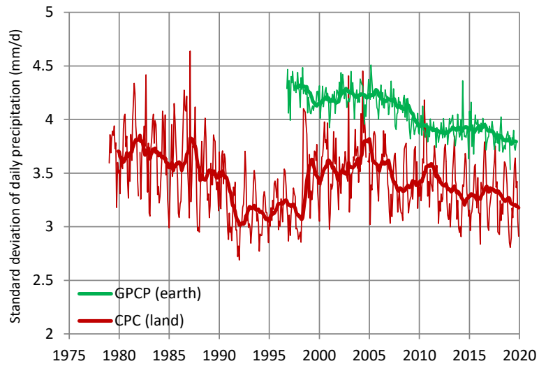
500 Figure B3: Variation of the standard deviation of daily precipitation in each month, areally averaged. Thin and thick lines of the same colour represent monthly values and running annual averages (right aligned), respectively. Sources of data are indicated in the legend and detailed in Table 1.
