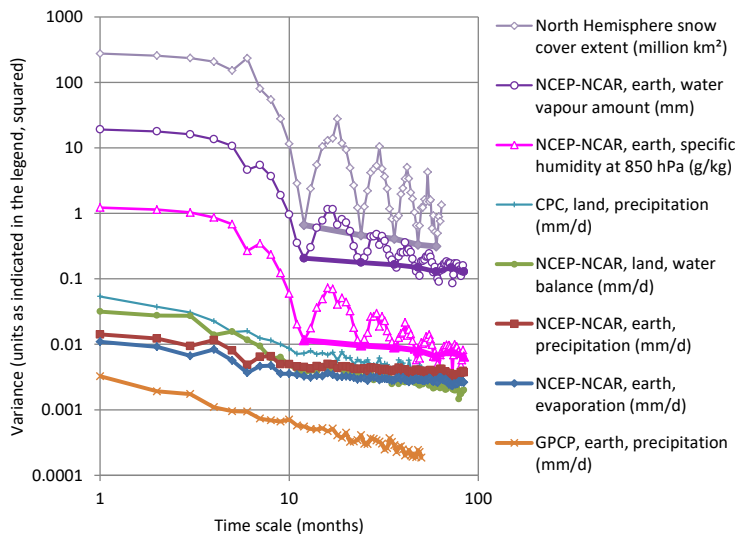
480 Figure 18: Climacograms of the indicated processes calculated from monthly time series: for some series with prominent seasonality the climacograms from annual time series are also plotted with thicker lines of same colour. For time scales larger than annually all slopes in the double logarithmic plots are close to -0.2 , suggesting a Hurst parameter 0.90 (or larger if bias is taken into account). Exceptions are the NH snow cover extent with a slope of -0.47 , suggesting a Hurst parameter 0.76 and the GPCP precipitation series with a slope of -0.72 , suggesting a Hurst parameter 0.64 .
