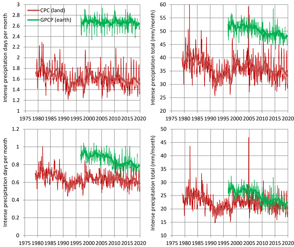
505 Figure B4: (Left column) Average days per month with precipitation exceeding a threshold value, which is 10 mm/d for the upper row and 20 mm/d for the lower row; (right column) monthly total of daily precipitation exceeding the threshold value. Thin and thick lines of the same colour represent monthly values and running annual averages (right aligned), respectively. Sources of data are indicated in the legend and detailed in Table 1.
