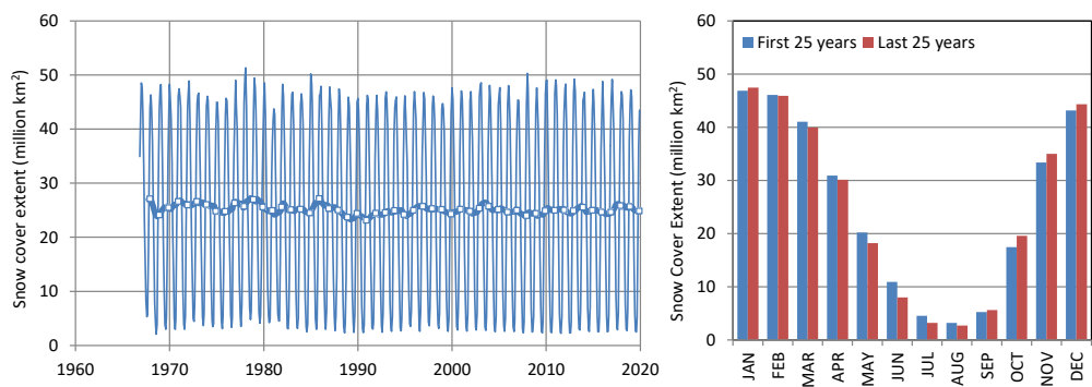
Figure 11: (Left) Variation of the snow cover extent in the northern hemisphere according to GSL; thin and thick lines represent monthly values and running annual averages (right aligned), respectively, and squares are annual averages aligned at December of each year. (Right) Seasonal variation of the snow cover, separately for the first and last 25 years of record.
