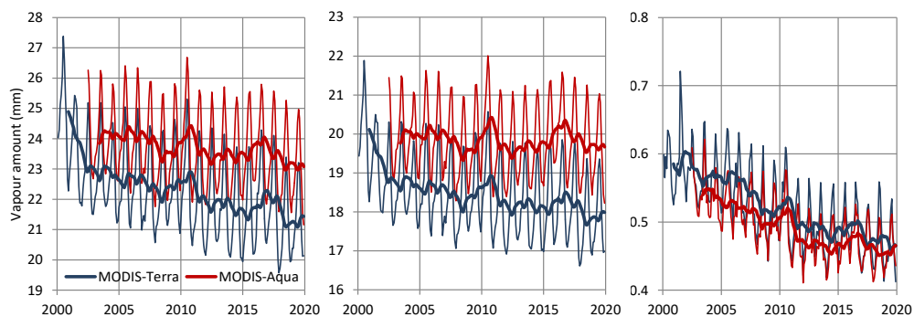
1435 Figure 8: Variation of water vapour amount as in Figure 7 but only for the MODIS data set and separately for the Terra and Aqua platforms: (left) total of the vertical column; (middle) from surface to 680 hPa; (right) from 440 to 10 hPa. Thin and thick lines of the same colour represent monthly values and running annual averages (right aligned), respectively . Sources of data are indicated in the legend and detailed in Table 1.
