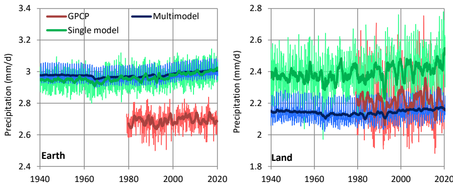
475 Figure 17: Comparison of climate model outputs (for specification of which see text) with reality, as quantified by GPCP satellite observations. “Multimodel” refers to CMIP5 scenario runs, entries: CMIP5 mean – rcp85. “Single model” refers to CCSM4 – rcp85 ensemble member 0, where CCSM4 stands for Community Climate System Model version 4, released by NCAR. Thin and thick lines of the same colour represent monthly values (but with rates expressed in \text{km}^3/\text{year} ) and running annual averages (right aligned), respectively.
