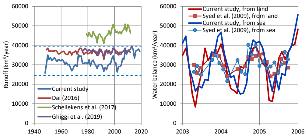
Figure 16: Comparison of results of the current study for surface runoff with those of (left) Dai (2016, Figure 2.8 digitized), Schellekens et al. (2017, Figure 7 digitized, ensemble mean) and Ghiggi et al. (2019, Figure 8a digitized, ensemble mean) at the annual scale, and (right) Syed et al. (2009, Figure 7 digitized) at monthly scale (but with rates expressed in \text{km}^3/\text{year} ). Dashed lines in the left panel are 95% confidence limits of the 30-year climatic average of the current study.
