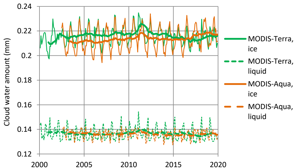
1440 Figure 9: Variation of cloud water amount (in ice and liquid phase). Thin and thick lines of the same colour represent monthly values and running annual averages (right aligned), respectively . Sources of data are indicated in the legend and detailed in Table 1.
