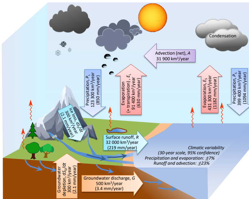
1460 Figure 14: Proposed quantification of water balance.
