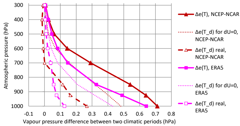
Figure 6: Vertical profile of the difference between two climatic periods of average water vapour water pressure e(T) and e(T_a) = U e(T) over land at levels of atmospheric pressure ranging from 1000 to 300 hPa. Sources of data: NCEP-NCAR and ERA5 reanalyses as detailed in Table 1 (entries 3, 4, 6, 7). For the NCEP-NCAR data, the differences are of the 30-year climatic periods 1948-77 and 1990-2019 and for the ERA5 data of the 20-year climatic periods 1980-99 and 2000-19.
