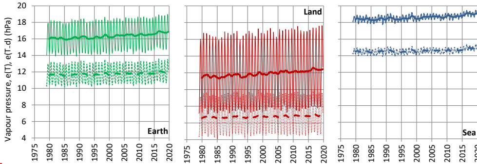
Figure 4: Variation of the saturation water pressure e(T) (continuous lines) and e(T_d) (dashed lines) for the average temperature T and dew point T_d as shown in Figure 2. Thin and thick lines of the same colour represent monthly values and running annual averages (right aligned), respectively. Sources of data: ERA5 reanalysis as detailed in Table 1.
