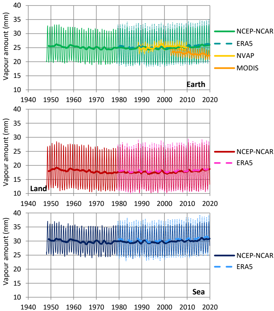
Figure 7: Variation of water vapour amount. Thin and thick lines of the same colour represent monthly values and running annual averages (right aligned), respectively. Sources of data are indicated in the legend and detailed in Table 1. The plotted values for MODIS represent the averages from Terra and Aqua platforms.
