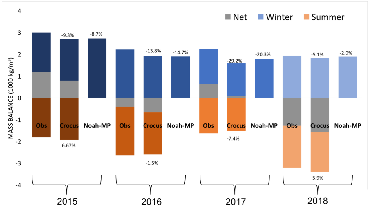
780 Figure 9: Box plot of winter, summer and net balance for the mass balance years 2015-2018 for Rembesdalskåka. Only winter mass balance is shown for Noah-MP.
