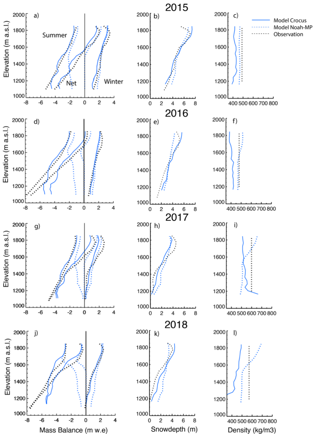
775 Figure 8: Left panels: Mass balance across Rembesdalskåka with height (a, d, g and j). Middle panel (b, e, h and k): Accumulated snow thickness associated with the winter mass balance. Right panel (c, f, I and l): Snow density of the accumulated snow. Each row represents a different year.
