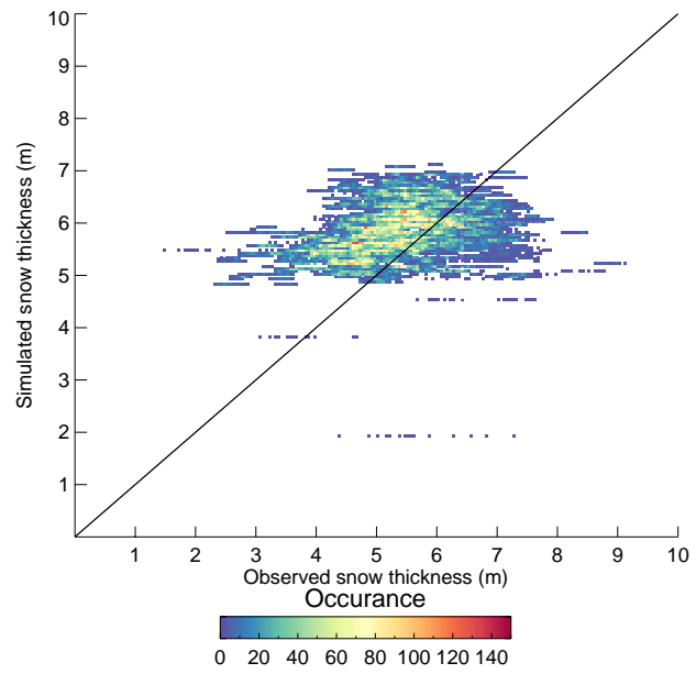
Figure 13: Simulated and GPR observed snow depth for 2017, but with no effect of sublimation from snow drift in the simulations.
