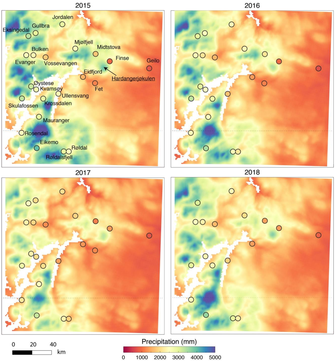
740 Figure 3: Simulated and observed precipitation (October – September) for mass balance years 2015-2018. Circles represent observations from AWS. The location of Hardangerjøkulen is also indicated.
