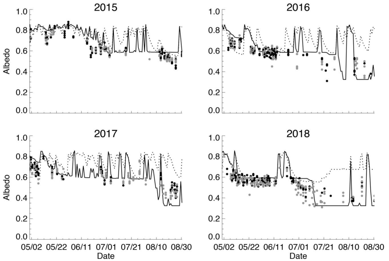
Figure 15: Same as Figure 14 but at a Northwest part of Hardangerjøkulen, where snow at times completely melts to the ice surface.
