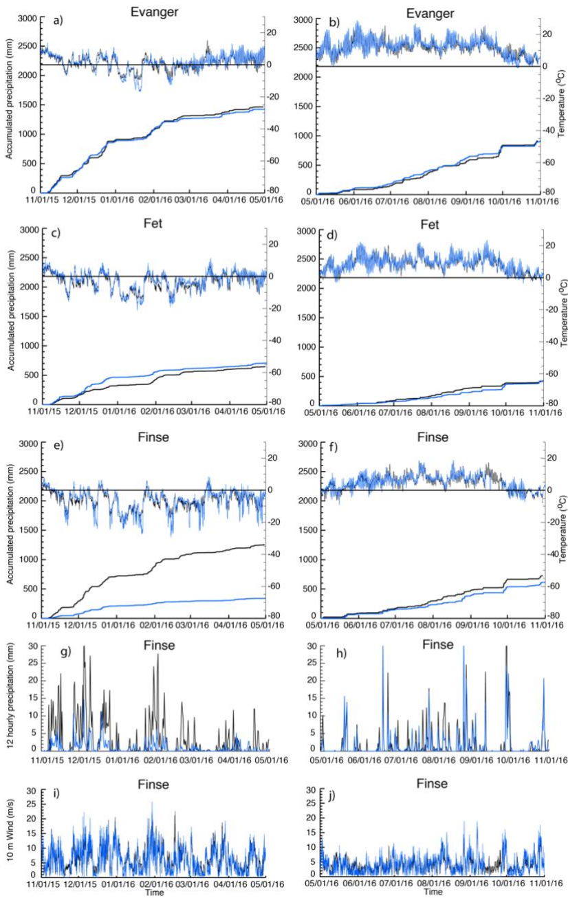
750 Figure 5: Observed (blue) and modeled (black) accumulated precipitation and temperature at Evanger (a, b), Fet (c, d) and Finse (e, f) stations for the 2016 winter season (left panel) and 2016 summer season (right panel). g) and h) shows time series of precipitation. The bottom panel (i, j) shows the 10 m wind speed at Finse.
