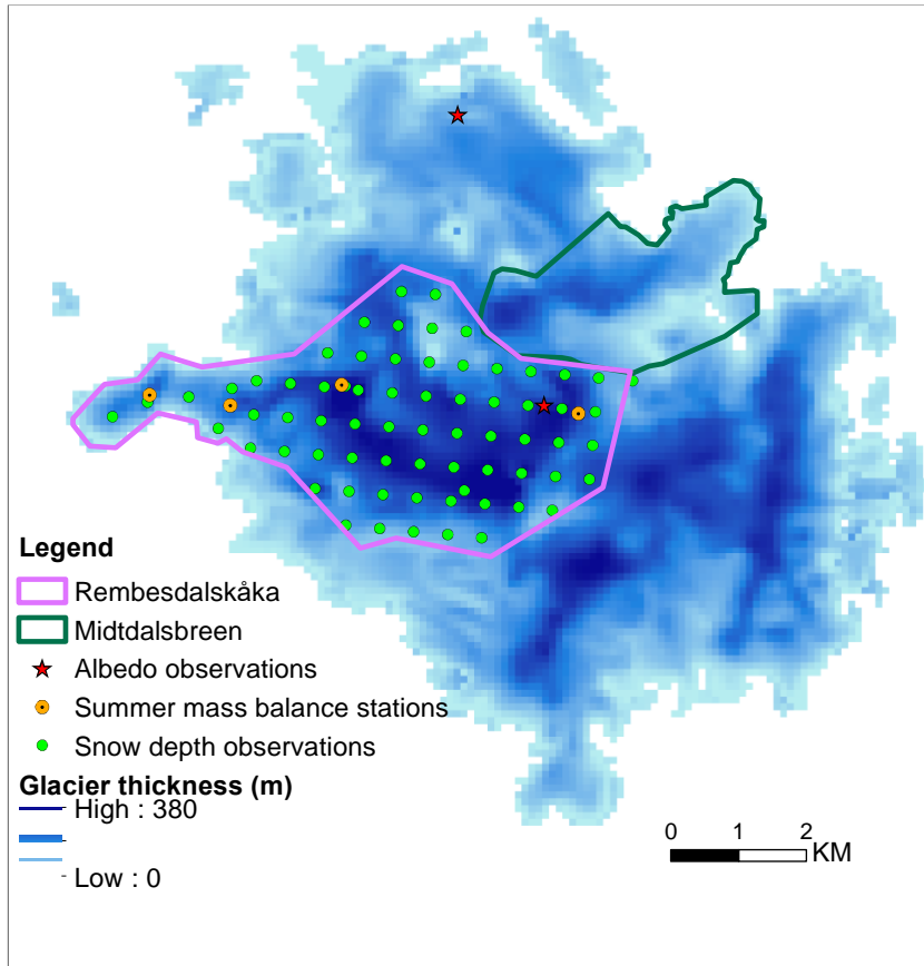
730 Figure 1: Glacier thickness and present extent for Hardangerjøkulen. The outlet glaciers Rembesdalskåka, Middalsbreen are also indicated. The green dots indicate locations where stake observations for winter balance were obtained, while orange dots indicate location of observations for summer balance. Stars shows location of albedo comparison with model against observations.
