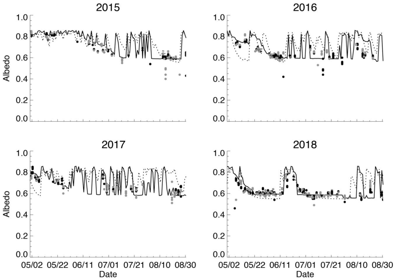
Figure 14: Observed and modeled albedo at the top of Hardangerjøkulen. Dots represent observed albedo from the MODIS satellite (Grey: Terra, Black: Aqua). Solid line is albedo from the Crocus snow model, dashed line is albedo from the Noah-MP snow model.
