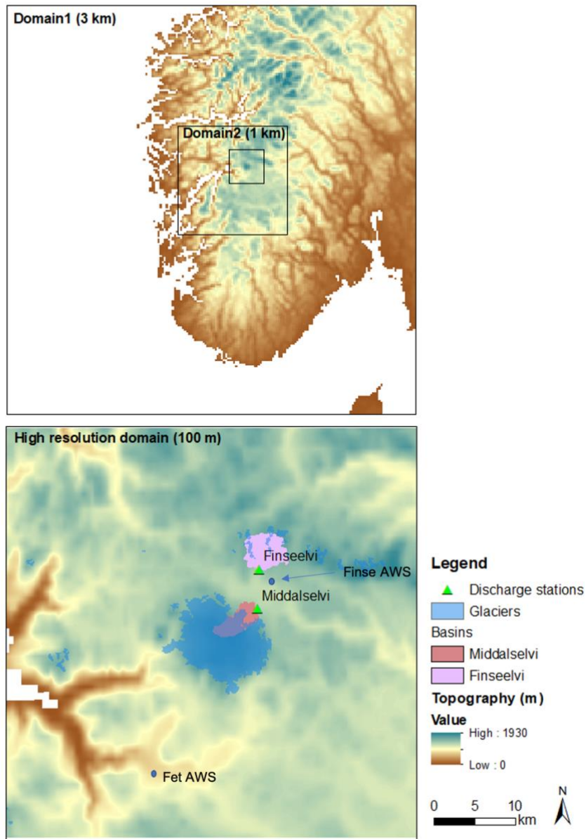
735 Figure 2: Model domains. The top figure shows the WRF domains with 3 km and 1 km grid spacing. The bottom figure shows the domain of the high resolution (100 m grid spacing) used with WRF-Hydro/Glacier. Furthermore, the outline of Hardangerjøkulen and the river basins of the two rivers with discharge observations are included as well.
