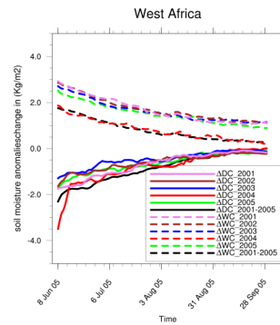
Fig. 1: Changes in daily soil moisture for 5 years (2001 to 2005) and their climatological mean during JJAS over West African domain, from dry ( \Delta DC ) and wet ( \Delta WC ) experiments with respect to their corresponding control experiment.
