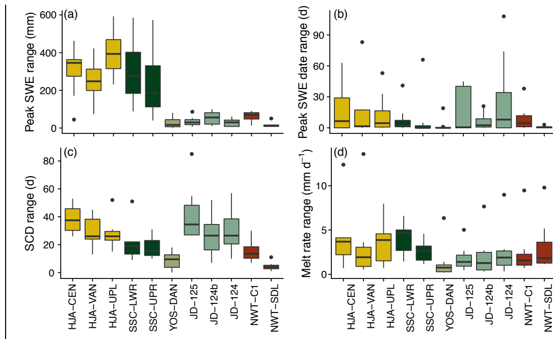
Figure 5. The annual range in simulated peak SWE (a), peak SWE date (b), snow cover duration (c), and melt rate (d) due to precipitation phase method selection at the study stations.
