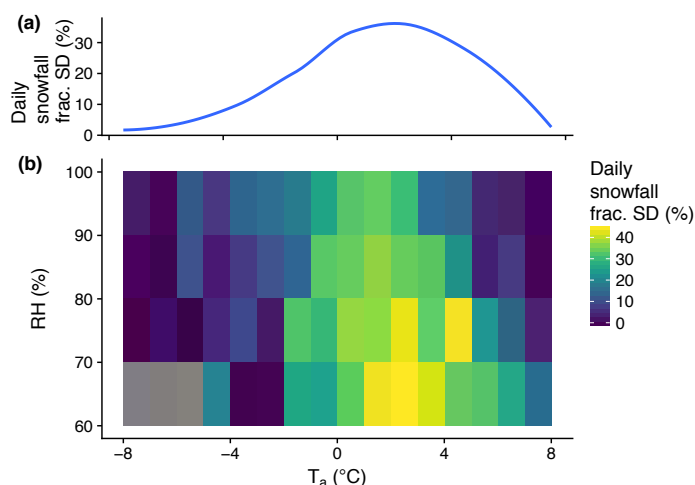
Figure 6. The standard deviation of daily snowfall fraction as a function of T_a (a) and as a function of T_a and RH (b). We binned the meteorological quantities within the ranges shown and calculated the standard deviation of snowfall fraction per T_a bin (a) and T_a /RH bin (b) using simulated precipitation phase from all stations and all methods.
