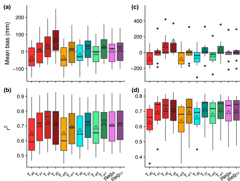
5 Figure A1. Mean bias (top row) and r^2 (bottom row) values for the SNOWPACK simulations relative to observed SWE (a,b) and snow depth (c,d). The boxplots show the median, interquartile range, minimum, maximum, and outlying values for each objective function for the different precipitation phase methods at all stations. The open triangles indicate the mean objective function value for that precipitation phase methods at all stations.
