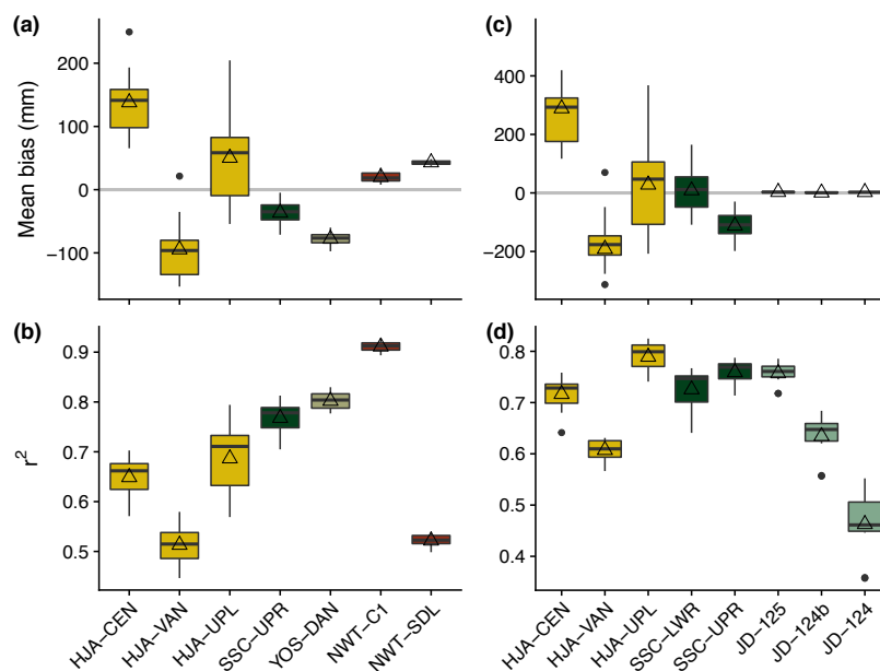
5 Figure A2. Mean bias (top row) and r^2 (bottom row) values for the SNOWPACK simulations relative to observed SWE (a,b) and snow depth (c,d). The boxplots show the median, interquartile range, minimum, maximum, and outlying values for each objective function for the different precipitation phase methods at a given station. The open triangles indicate the mean objective function value for all precipitation phase methods at that station.
