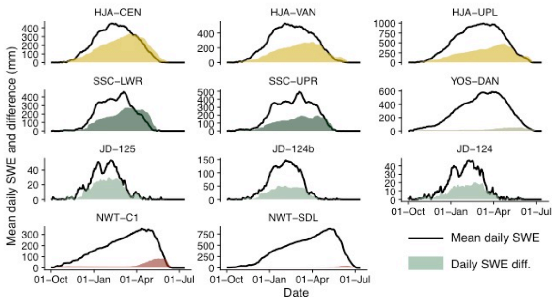
Figure 4. Mean daily SWE (solid black line) and the difference between maximum and minimum mean daily SWE (shading) at the study stations. The mean daily SWE was computed by averaging the simulated SWE on each day for all precipitation phase methods across the simulation years. The difference was calculated by subtracting the minimum mean daily SWE from the maximum mean daily SWE produced by the different precipitation phase methods (mean daily SWE plots broken out by precipitation phase method can be viewed in Figs. S1–S11). The T_{a0} and T_{a0} methods typically produced the minimum mean daily SWE, while T_{a3} and T_{d1} produced the maximum.
