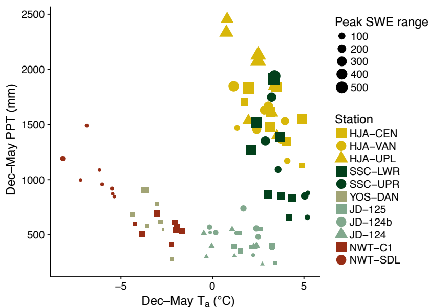
Figure 8. Range in annual peak SWE as simulated by the different precipitation phase methods at the 11 study stations. Each point represents one simulation year at a given station and larger points correspond to larger differences in maximum minus minimum peak SWE. Predicting the peak SWE range as a function of Dec-May T_a and PPT using multiple linear regression yielded an r^2 of 0.81 ( p -value < 0.0001).
