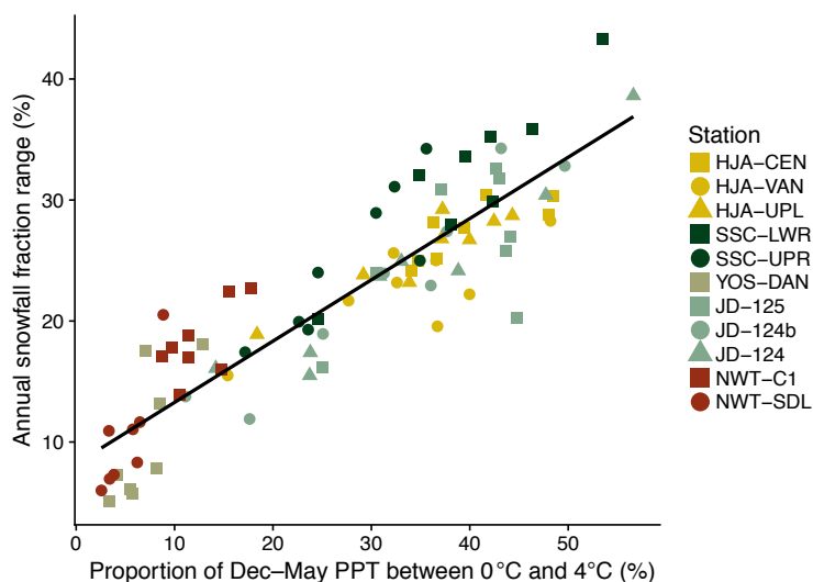
Figure 7. Range in annual snowfall fraction as predicted by the proportion of Dec–May PPT falling between 0°C and 4°C. Each point represents one simulation year at a station identified by the color and shape. The black line of best fit was calculated using ordinary least squares regression ( r^2 = 0.80 , p -value < 0.0001).
