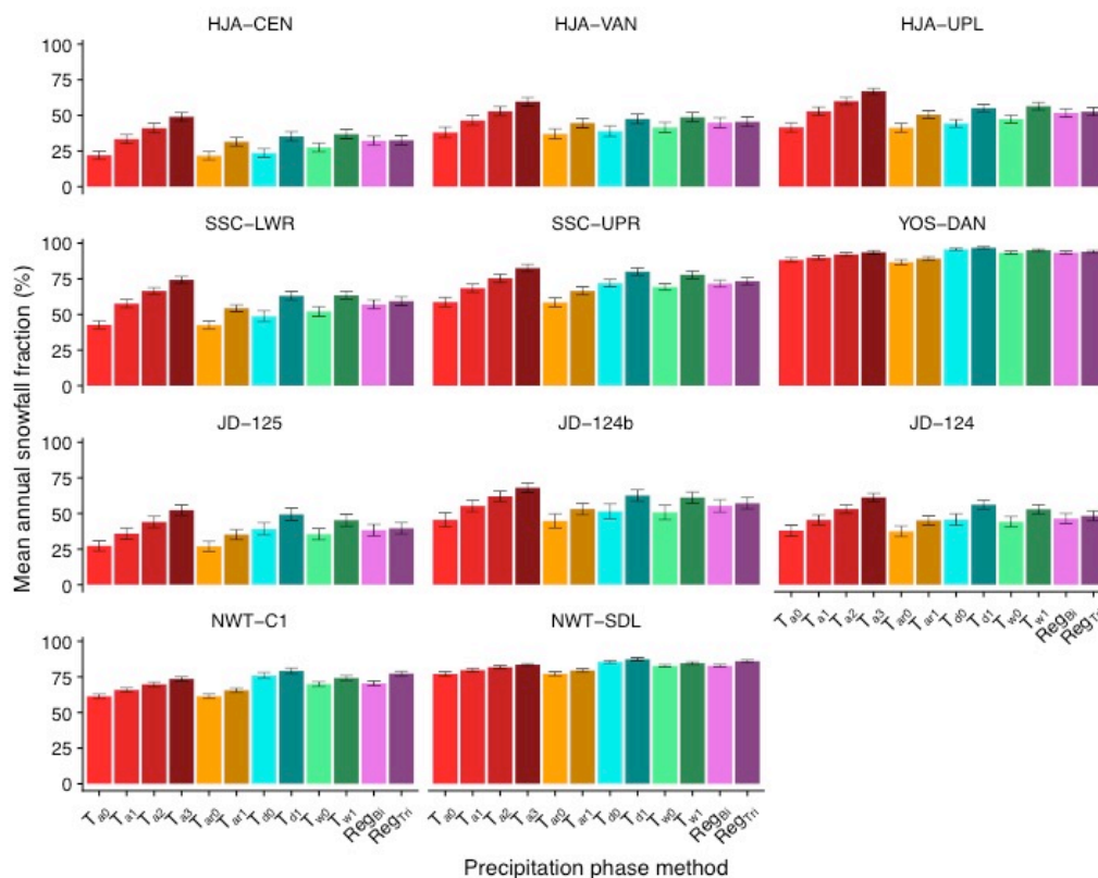
Figure 3. Mean annual snowfall fraction at the 11 study stations for the 12 different precipitation phase methods. The whiskers represent the standard error of annual snowfall fraction for the 8 simulation years. For this plot and all subsequent figures showing the station data, the maritime sites are shown in the top two rows, the intermountain site is in the third row, and the continental site is in the bottom row.
