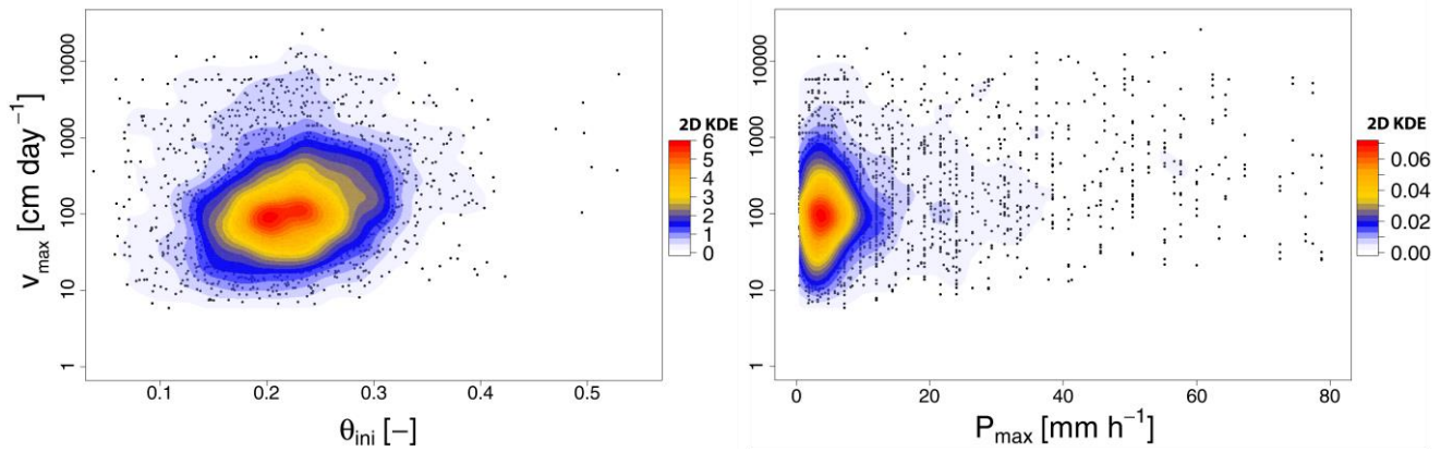
Figure 9: Measured SR maximum pore water velocities ( v_{max} ) in relation to \theta_{ini} and P_{max} . Color contours indicate 2D kernel density estimation (2D KDE). The points show single event values.
