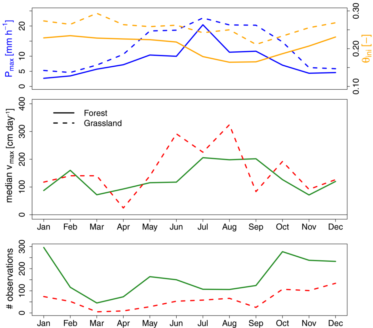
Figure 12: Monthly mean P_{\max} and \theta_{ini} (upper diagram), monthly median v_{\max} for the two land covers (middle diagram) and number of observed v_{\max} values ( SR that reached either 30 or 50 cm) for each land cover and month (lower diagram). The solid lines represent the forest and the dotted lines the grassland response.
