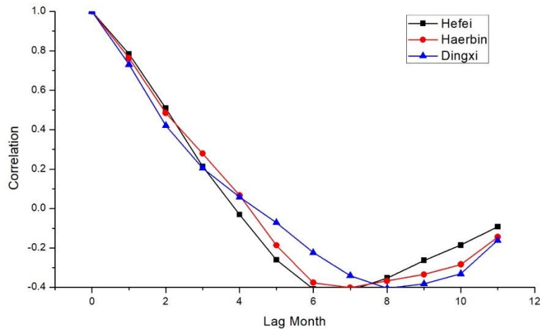
Figure 1 Autocorrelation of simulated SM as a function of the monthly lag of three selected stations.
