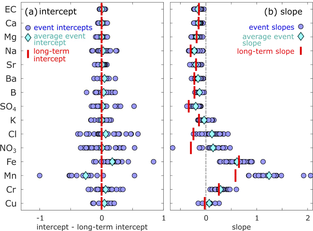
Figure 3: A comparison of event-scale and long-term cQ intercepts (a) and slopes (b). Blue circles represent intercepts and slopes for individual events, light-blue diamonds represent the averages of all events, and red bars indicate the slopes and intercepts of the long-term cQ relationships. If the red bar is close to the light-blue diamond, the long-term slope or intercept value is a good approximation of the average event slope or intercept. In panel (a), event cQ intercepts are expressed relative to the long-term average for better visual comparison of the solutes. Event-scale intercepts and slopes vary substantially for solutes in the lower half of the figure (from chloride to chromium), but vary little for most groundwater-sourced solutes. Because we normalized discharge by the mean discharge value, long-term intercepts approximate the average event-intercepts. Long-term slopes also approximate the event slopes for most groundwater-sourced solutes, but long-term slopes are more negative than event slopes for, e.g., chloride, nitrate, and manganese.
