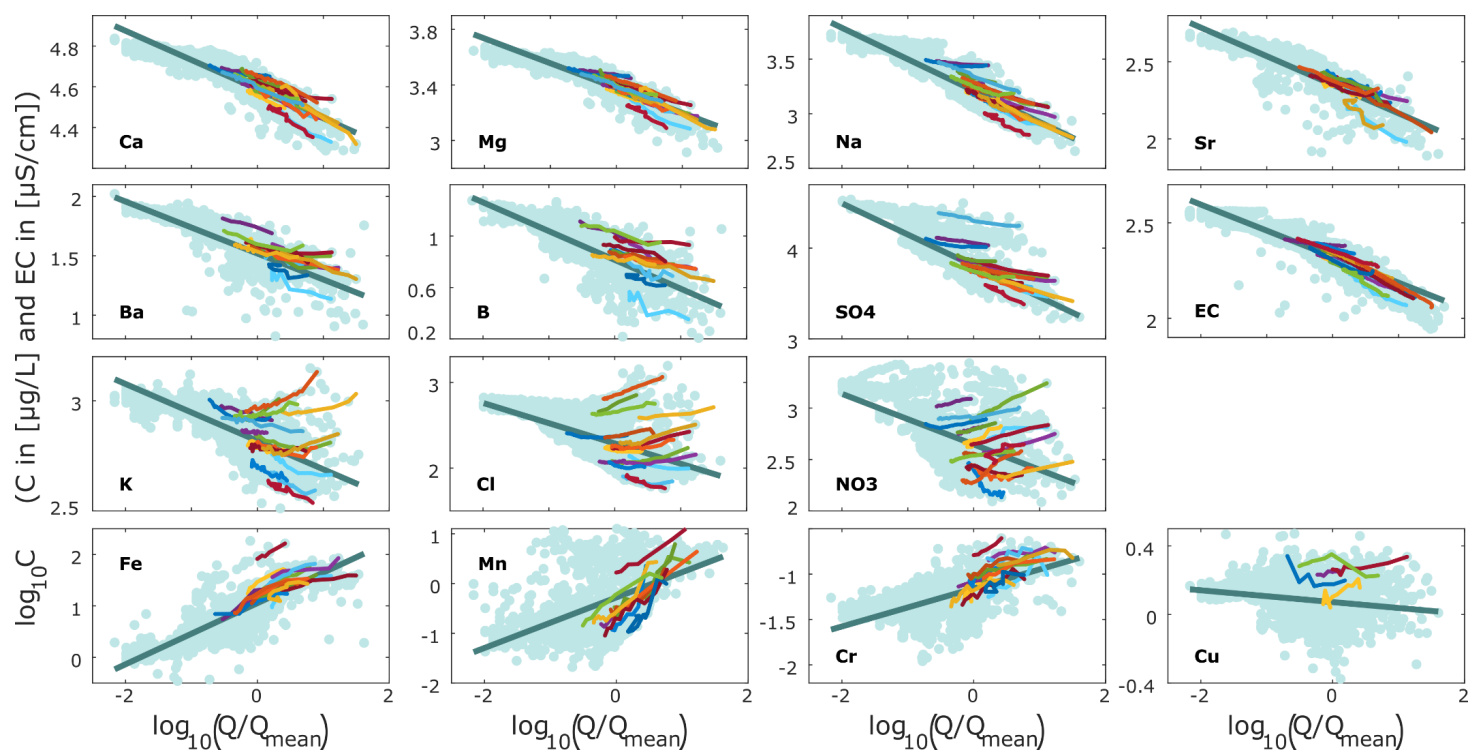
Figure 2: Long-term cQ relationships from the entire recession time series (data points are shown in light blue and the dark blue line indicates the power-law fit), compared to the cQ behavior of individual events (colored lines; up to 20 events are shown for better visibility). Discharge is normalized by the average discharge of the time series. Most solutes exhibit a long-term dilution pattern, whereas the trace metals iron, manganese, and chromium exhibit a long-term mobilization pattern. The cQ relationships vary much more from event to event for some solutes (e.g. potassium, chloride, and nitrate) than for others (e.g. calcium, magnesium, sodium, and EC).
