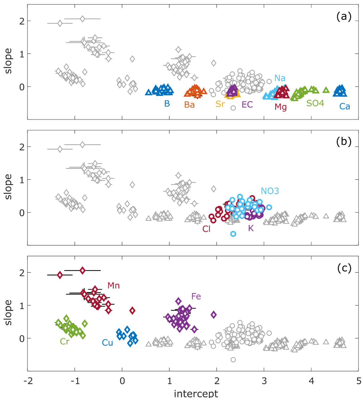
Figure 4: Scatter plots of event cQ slopes and intercepts of the 14 different solutes and EC (error bars indicate one standard error). Solutes from different dominant sources cluster and exhibit similar ranges of variability. (a) Groundwater-sourced solutes cluster closely around similar slopes and show little inter-event variability in both slopes and intercepts. (b) Intercepts and slopes of solutes with significant atmospheric input (i.e., chloride, nitrate, and potassium) vary substantially among events. (c) The slopes of trace metals are generally higher than those of the other solutes (indicating predominantly mobilization behavior), and are also highly variable among events. The uncertainty in the estimated slopes and intercepts is mostly smaller than the variability between events, indicating that the observed inter-event variability in slopes and intercepts reflects real-world behavior rather than sampling and measurement noise.
