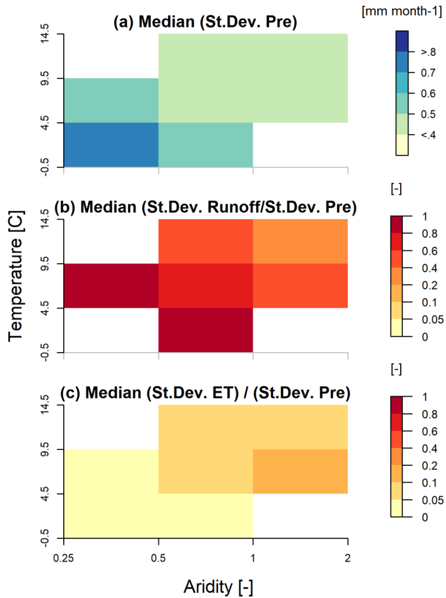
Figure S2: Same as figure 4 in the main text, but with results obtained from the model calibrated using GPCC precipitation data.
