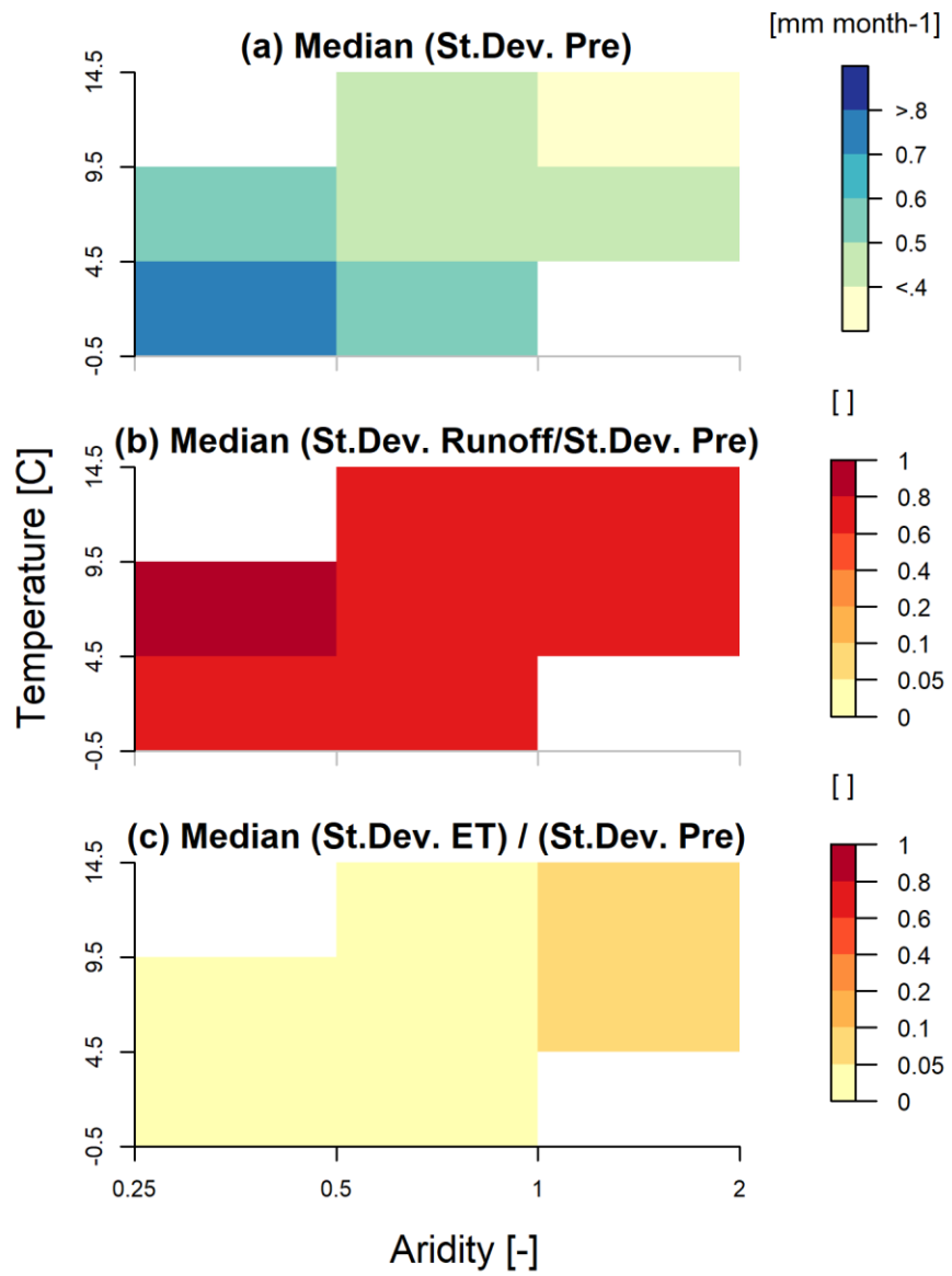
10 Figure S3: Same as figure 4 in the main text, but with results computed for whole year.
