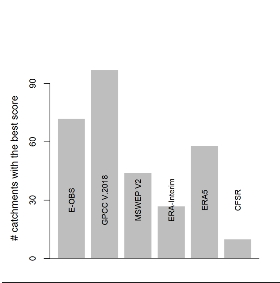
Figure S5: Same as figure 5 in the main text, but with results obtained from the model calibrated using GPCC precipitation data.
