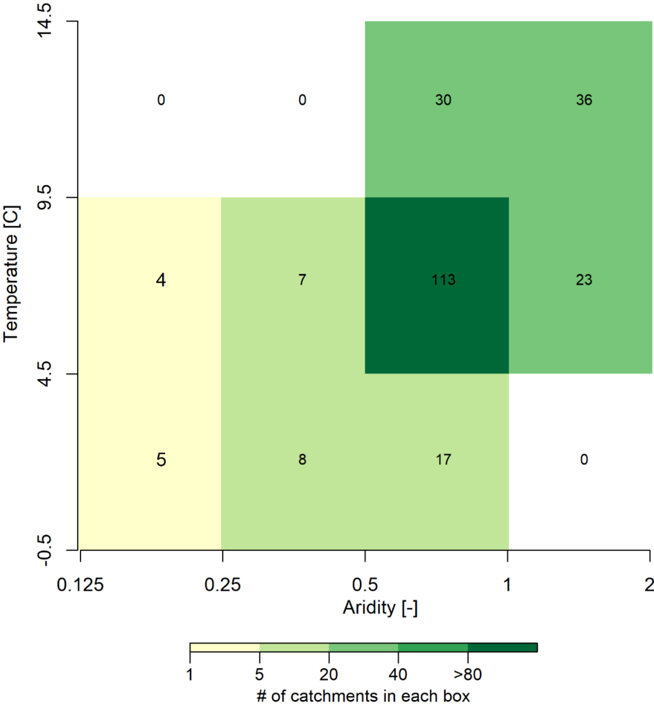
Figure S1: Number of considered catchments in each climatic box. Overall, 243 catchments across Europe are evaluated in this study.
