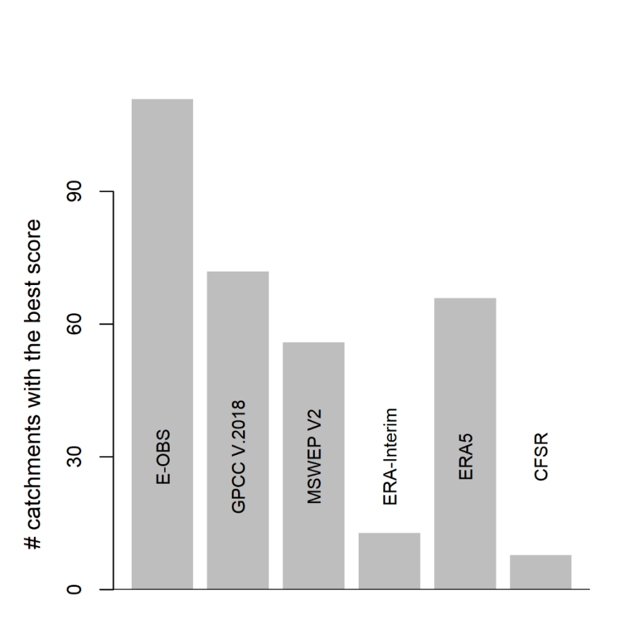
Figure S4: Same as figure 5 in the main text, but with results computed for whole year.
