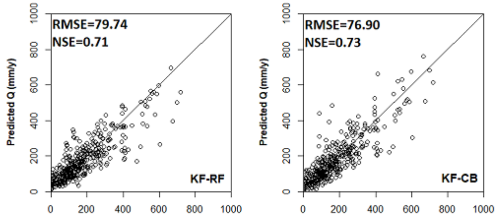
Fig. 1. Model performance of KF-RF: K-Fold cross-validated random forest model, KF-CB: k-fold cross-validated cubist model, when model was ran after excluding DEM.
