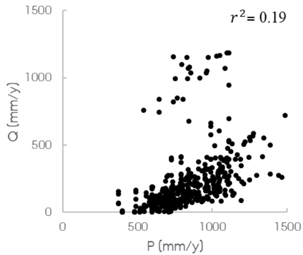
Figure 1. Correlation between measured precipitation (P) and measured drainage discharge (Q)
