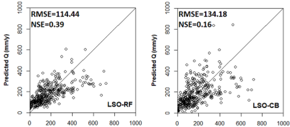
Fig. 8. Model performance of LSO-RF: Leave station out cross-validated random forest model, LSO-CB: Leave station out cross-validated cubist model, when models was ran after excluding DEM.
