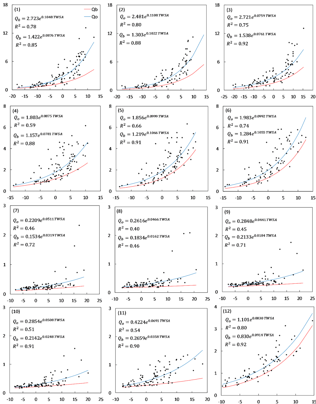
Figure 3: Non-winter (Apr-Oct) monthly observed discharge ( Q_o ; y-axis in units of cm) and storage ( S , x-axis in units of cm represented by TWSAs); the lines represent the relationship between observed discharge (blue) or baseflow (red) and storage. The plots IDs correspond to the site IDs listed Table 1 and shown in Figure 1. All relationships are significant at a 99% confidence interval (p-value < 0.00001), based on t-test.
