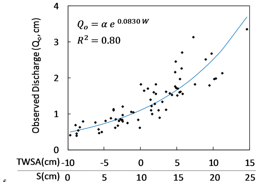
Figure 2: Storage-Discharge for the Mississippi River Basin (Site 12) based on Eq. (3) and an assumed S_o value of 10 cm, which is arbitrarily selected to illustrate the effects on Q - S relationships, where W represents storage in GRACE TWSA units (x-axis TWSA-cm) or absolute units (x-axis S-cm) and \alpha is 1.101 if W is TWSA or 0.4934 if W is S.
