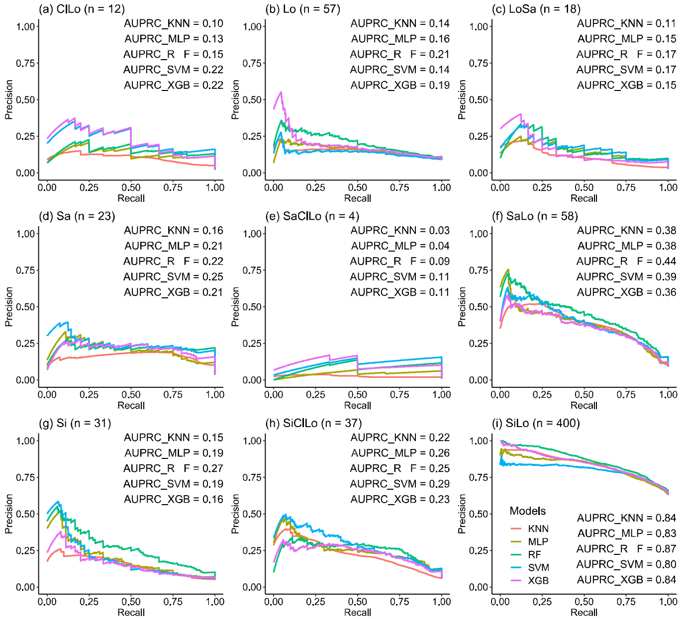
Figure 4. The AUPRCs for different machine-learning methods of each soil texture type (a) CI Lo (b) Lo (c) LoSa (d) Sa (e) SaCI Lo (f) SaLo (g) Si (h) SiCI Lo (i) SiLo; n was the sampling points of different soil texture types.
