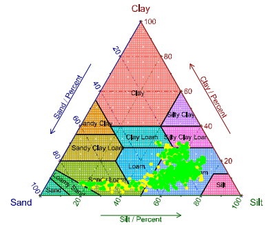
(f) RF_ILR (83.9%)
