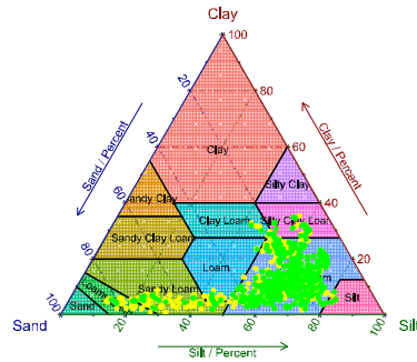
(e) MLP_ORI (63.6%)
