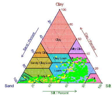
(i) SVM_ORI (66.4%)
