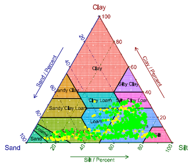
(j) XGB_ILR (67.8%)
