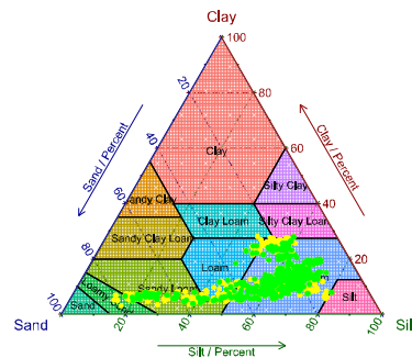
(k) XGB_ORI (68.0%)
